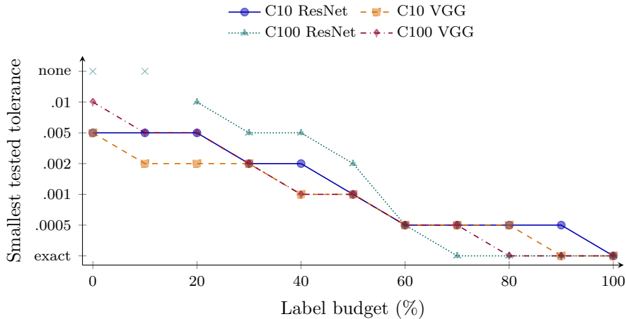
Figure 8: Choose an evaluation tolerance for a label budget. Smallest certified tolerance on the six-value grid, using static range on the four original pools ( n = 10,000 ). Marks show all eleven budgets; crosses at “none” mean no tested tolerance is certified. Lines guide the eye. The tolerance axis lists grid values, not equal numerical intervals. This is a policy-specific guarantee, not the optimal attainable tolerance.
