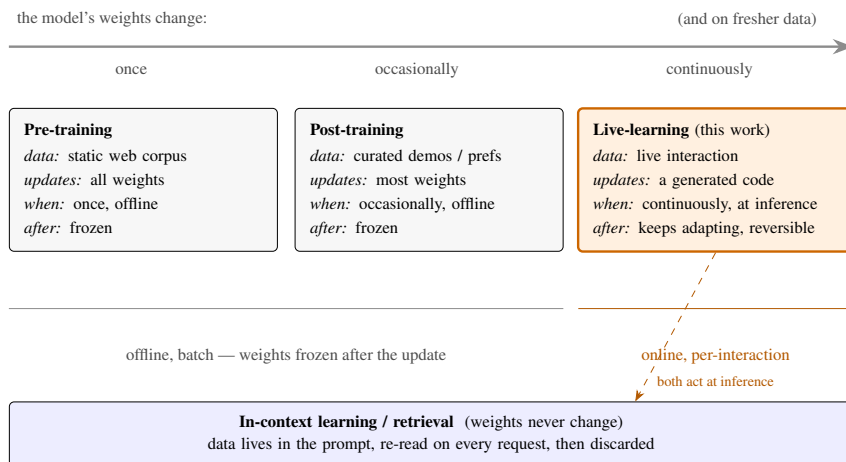
Figure 1: Three regimes for turning data into model capability, ordered by how often the model’s weights change and how recent the data they learn from is. Pre-training and post-training (SFT, RLHF) both update the weights offline, in batch, and leave them frozen thereafter; they differ mainly in the data they use and how often they run. Live-learning , the regime this work targets, updates a generated low-rank code continuously, at inference, on the interaction data — facts, corrections, outcomes — that the others cannot reach in the loop, and keeps adapting rather than freezing. In-context learning and retrieval (bottom) also act at inference, but they leave the weights unchanged and carry the data in the prompt, where it is re-read every request and then discarded. The regimes are complementary, not competing: live-learning does not replace pretraining (§ 4), it reaches the data pretraining and prompting leave on the table.
