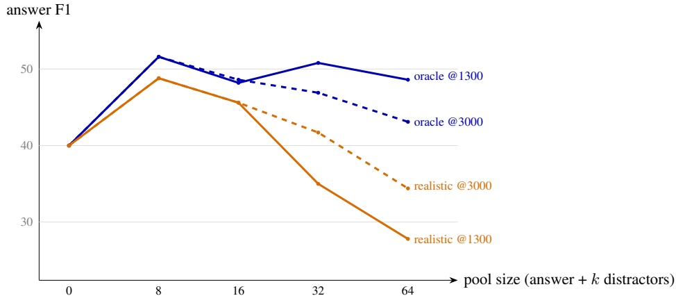
Figure 5: The dilution boundary (MS MARCO v2.1, top-1 answer F1, measured, n = 150 ), at two encoder context budgets (1300 solid, 3000 dashed). Oracle (blue) keeps the answer passage fronted so it survives truncation; realistic (orange) shuffles passage order so the answer is as exposed as any other. Even the oracle declines as the pool grows with nothing truncated ( 51.6 \rightarrow 46.9 F1 from 8 to 32 distractors at 3000 tokens, 0% truncation) — the code saturates : a fixed-size code loses fidelity as it carries more. The realistic read falls further below the oracle because the answer is either truncated out (dominant at 1300 tokens, where the 32- and 64-passages reads are 100% truncated) or, once the budget is large enough that nothing truncates (0% at 3000 for \leq 32 passages), simply buried among distractors and read less faithfully. Saturation bounds how much one code should hold; truncation and burial are failures of foregrounding the right evidence — together they motivate one bounded read per code plus a selector over the pool, rather than one ever-larger read.
