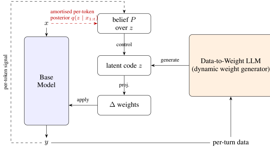
Figure 3: The architecture, organised around a belief over the latent code z . On the main (per-turn) path, live data is read by the Data-to-Weight LLM (the encoder E_\phi of § 3.2) into a latent code z ; the code generates a low-rank weight delta \Delta W that modulates the frozen base model , which produces the output. A belief P over z sits above the code and is what makes the weight move : it is updated online, carried from step to step rather than re-encoded from scratch. The per-token signal (dashed) — the running hidden state, equivalently the realised output, of the autoregressive stream — feeds the belief and is introduced only to amortise the per-token posterior q(z | x_{1:t}) ; it is not on the main data path. The belief’s form — a Gaussian over a continuous code, or a categorical posterior over materialised codes — is the architectural choice of § 3.5.
