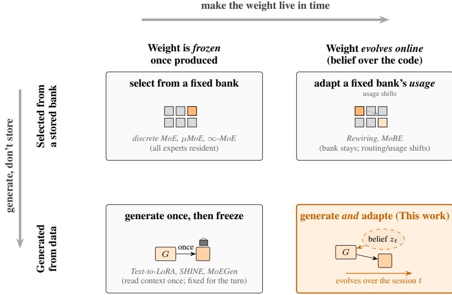
Figure 2: The two architecture axes of the design, and where prior work sits. Down — where each token’s weight comes from: selected from a stored, fully-resident bank (top), or generated on demand from a compact resident generator (bottom); this is the “generate, don’t store” move, and it buys a fixed footprint. Across — what happens to the weight after it is produced: frozen once made (left), or carried as a belief over its latent code and updated online (right); this is the axis that makes the weight live in time . Stored-bank MoE ( \mu MoE, \infty -MoE) and the one-shot weight generators (Text-to-LoRA, SHINE, MoEGen) each sit in a single cell; only the bottom-right — generate the weight from live data and keep a moving belief over the code — is occupied by this work. “Infinite parameters” is the reach this opens up: an unbounded set of effective weights and behaviours across both facts and time, from a fixed resident footprint — not an unbounded store of knowledge, which the capacity laws forbid and we do not claim (§§ 3.4 and 4). Attention is unchanged throughout; the bounded-vs-unbounded geometry of a single generated layer is developed in Figure 4.
