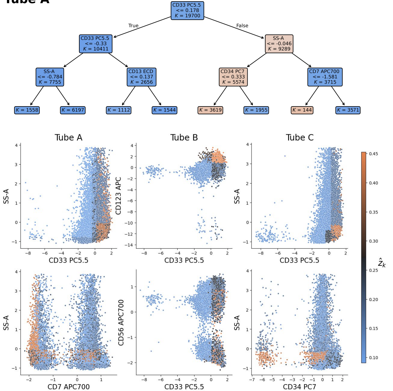
Fig. 6. Cell-level interpretation for FLT3 -ITD detection on the test dataset
