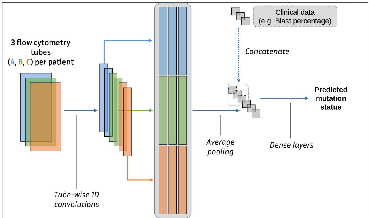
Fig. 3. Deep CNN architecture for flow cytometry analysis
