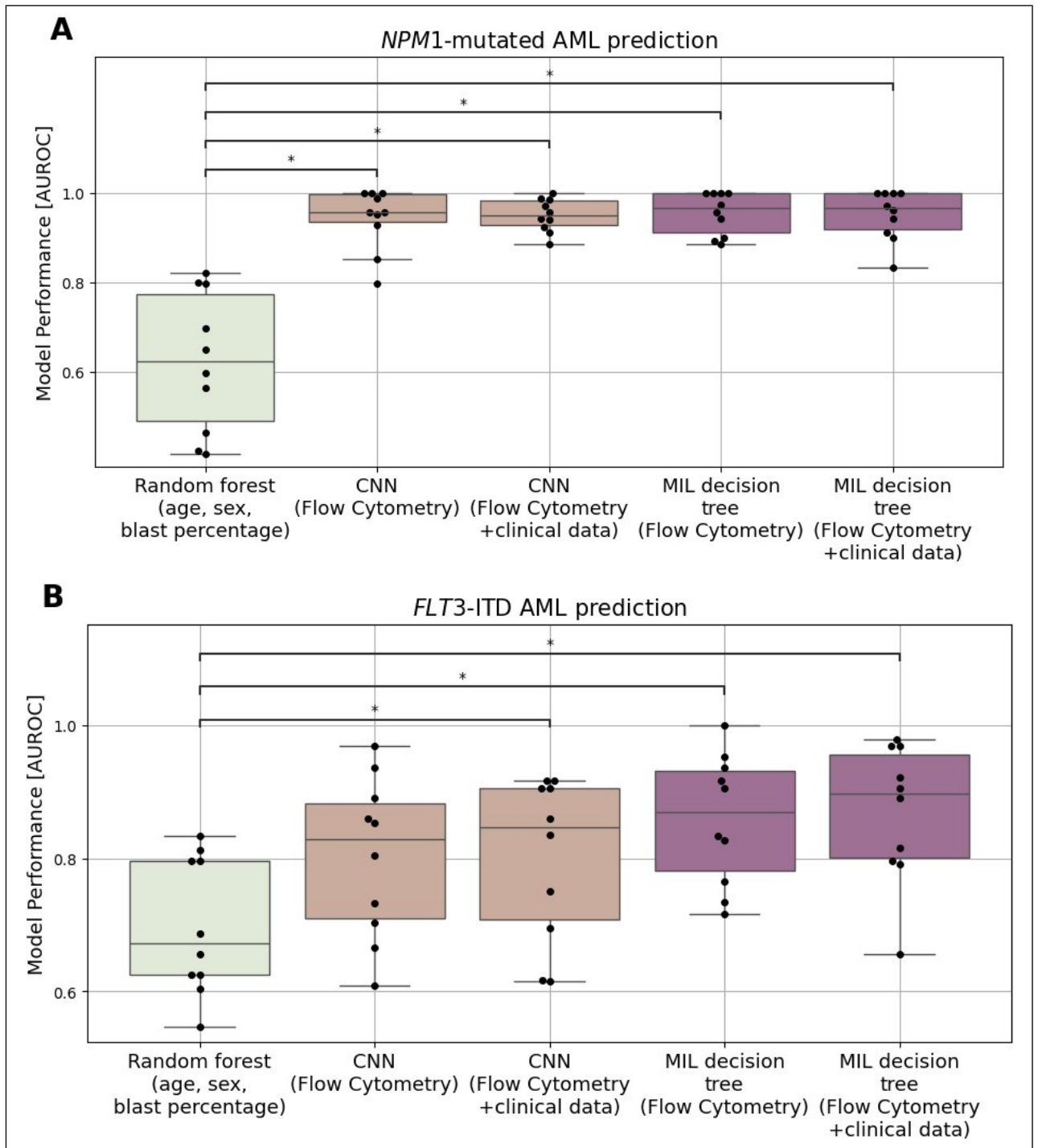
Fig. 4. Models' performance on left-out validation folds
