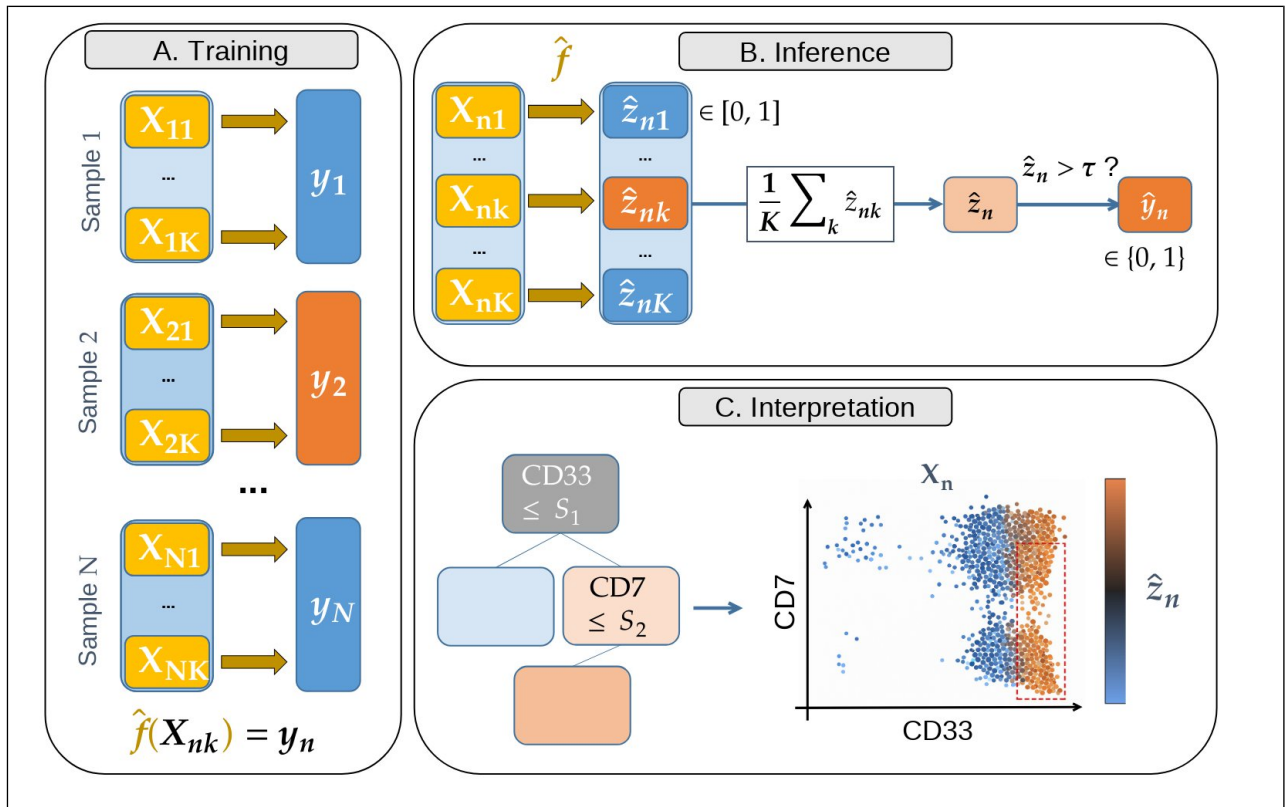
Fig. 2. Multi-instance learning model for mutation detection
