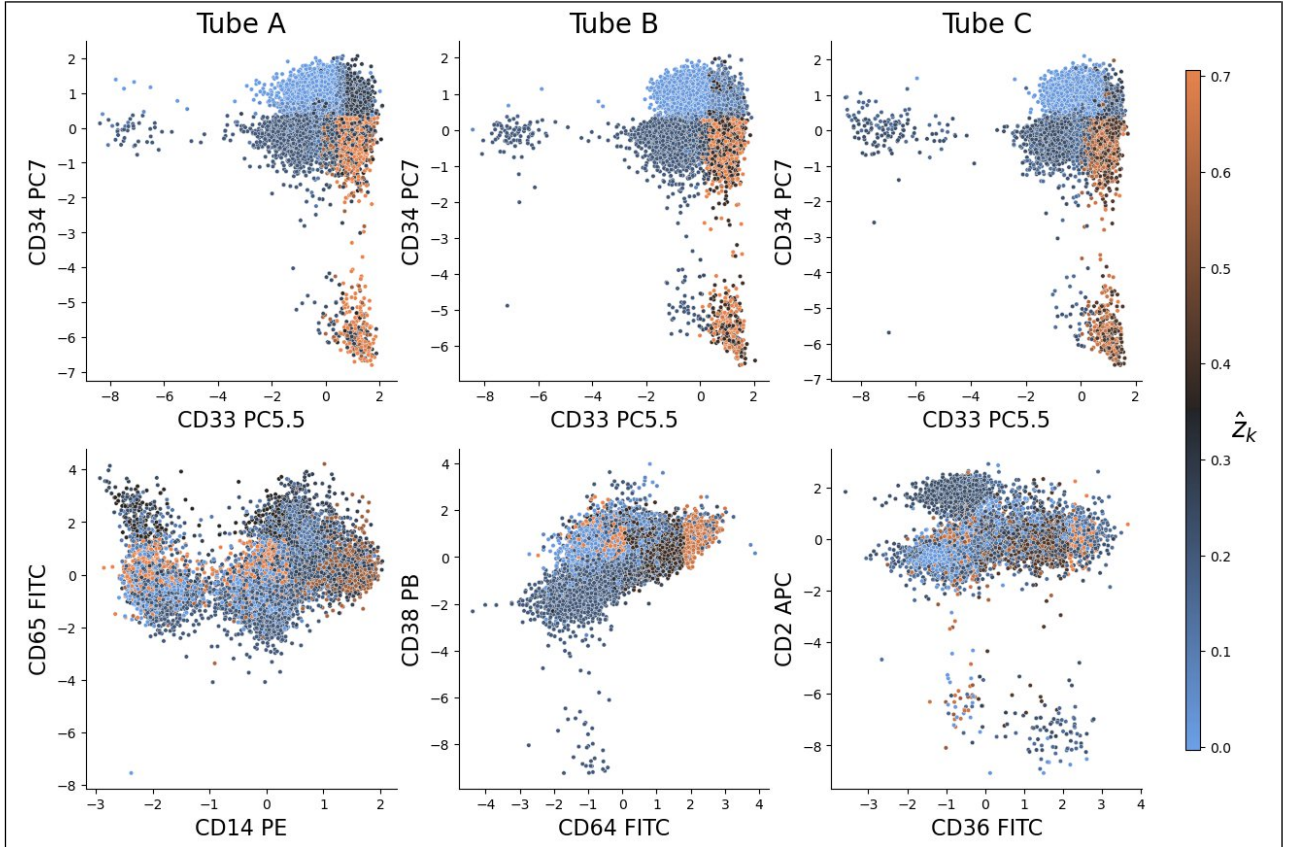
Fig. 5. Cell-level interpretation for NPM1 mutation detection on the test dataset
