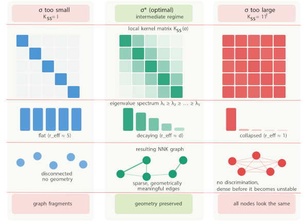
Fig. 1. Spectral regimes of the local kernel operator \mathbf{K}_{SS}(\sigma) . Left: \sigma too small — identity-like, flat spectrum, r_{\text{eff}} \approx |S| , graph fragments, no geometric information. Center: \sigma^* — decaying spectrum, r_{\text{eff}} \approx \hat{d} , well-conditioned, geometrically informative. Right: \sigma too large — rank-one, \kappa \rightarrow \infty , all directions collapsed, discrimination lost.
