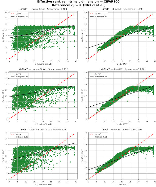
Fig. 2. r_{\text{eff}}(K_{SS}) at \sigma^* vs. per-node intrinsic dimension for 3 encoders (rows) for the LB estimator (Left) and dimMST (Right). dimMST aligns substantially better, confirming it as a better complexity target under distance concentration.
