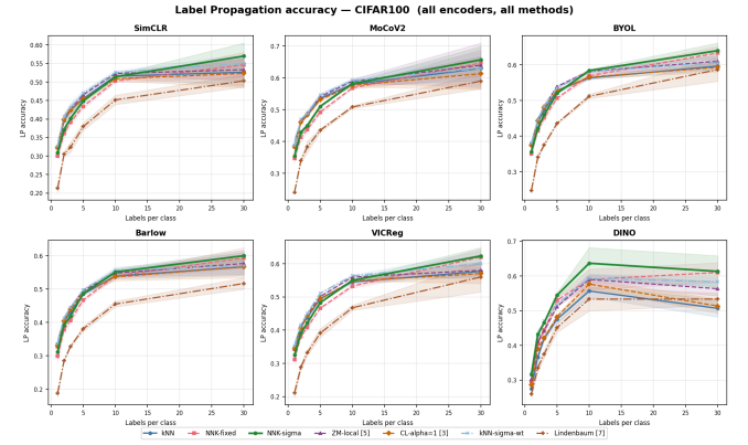
Fig. 4. LP accuracy vs. labels per class, six encoders. NNK- \sigma (green) leads on CIFAR-100 across all encoders, with gains over NNK-fixed most pronounced at \geq 10 labels per class.
