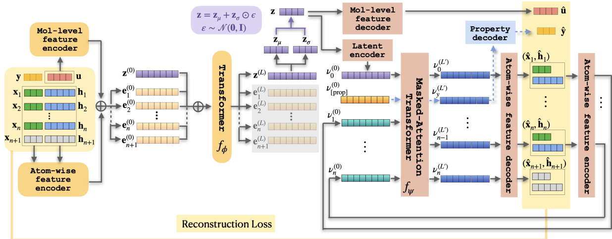
Figure 1: Overview of EF-TAVAE. A canonically ordered and aligned molecule with n atoms is represented as \mathcal{M} = (\mathbf{u}, (\mathbf{x}_1, \mathbf{h}_1), \dots, (\mathbf{x}_n, \mathbf{h}_n)) , where \mathbf{u} denotes molecule-level categorical features, and (\mathbf{x}_i, \mathbf{h}_i) denotes the canonicalized 3D coordinate and atom-level categorical features of atom i \in \{1, \dots, n\} . We append the final nonphysical end-of-molecule (EOM) token (\mathbf{x}_{n+1}, \mathbf{h}_{n+1}) with \mathbf{x}_{n+1} = \mathbf{0} and the special label [EOS] in its atom-level categorical fields. Atom- and molecule-level feature encoders form input embeddings (\mathbf{e}_1^{(0)}, \dots, \mathbf{e}_{n+1}^{(0)}) , to which a learnable sequence token \mathbf{z}^{(0)} is prepended. A bidirectional Transformer encoder f_\phi produces contextualized embeddings; its sequence-token output \mathbf{z}^{(L)} parameterizes the diagonal Gaussian posterior through (\mathbf{z}_\mu, \mathbf{z}_\sigma) . The latent code is sampled by reparameterization as \mathbf{z} = \mathbf{z}_\mu + \mathbf{z}_\sigma \odot \boldsymbol{\epsilon} , with \boldsymbol{\epsilon} \sim \mathcal{N}(\mathbf{0}, \mathbf{I}) . From \mathbf{z} , EF-TAVAE first predicts the molecule-level features \hat{\mathbf{u}} and constructs latent-conditioned decoder inputs \mathbf{v}_0^{(0)} . The causal Transformer decoder f_\psi then uses masked self-attention to generate \mathbf{v}_i^{(L)} autoregressively: it maps \mathbf{v}_i^{(L)} to next atom-level outputs (\hat{\mathbf{x}}_{i+1}, \hat{\mathbf{h}}_{i+1}) , which are then encoded into \mathbf{v}_{i+1}^{(0)} , recursively, terminating when it emits [EOS] in \hat{\mathbf{h}}_{i+1} . When optional property supervision is enabled, a learned property token \mathbf{v}_{[\text{PROP}]}^{(0)} is inserted after the latent decoder token. Its final representation \mathbf{v}_{[\text{PROP}]}^{(L)} is passed through a property readout head to predict \hat{\mathbf{y}} . The blue dashed path denotes this property-supervised readout. Autoregressive atom states never attend to the property token, so the property pathway does not alter the atom-generation process. Here, \mathbf{y} is used as a supervision target rather than as an encoder input. During training, teacher forcing supplies the preceding ground-truth atom tokens, and the reconstruction loss is applied to the molecule- and atom-level predictions. When property supervision is enabled, the property-reconstruction loss is additionally included in the training objective.
