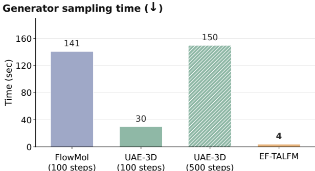
Figure 7: EF-TALFM substantially reduces generator sampling time. Generator-only sampling time for 10,000 molecules. EF-TALFM uses the adaptive fifth-order Dormand–Prince solver, UAE-3D uses a DDPM sampler, and FlowMol uses Euler integration.
