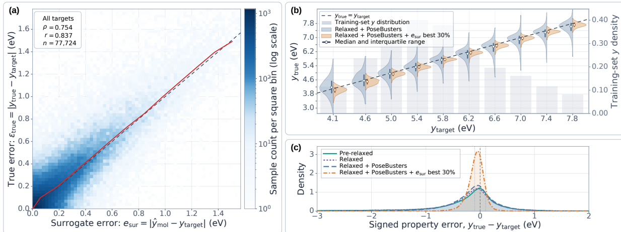
Figure 6: (a) Internal-readout error is a strong and practically useful indicator of the true error. For 77,724 conditionally generated molecules, the internal-readout error e_{\text{sur}} is strongly correlated with the true error \epsilon_{\text{true}} , with Spearman \rho = 0.754 and Pearson r = 0.837 . The binned-median trend (red solid line) broadly follows the diagonal x = y (dashed line), showing that molecules with smaller internal-readout errors tend to have true properties closer to their targets. (b) Selecting by internal-readout error substantially narrows the true-property distributions around the requested targets. For each target property y_{\text{target}} , the panel shows the distribution of corresponding true properties y_{\text{true}} for \mathcal{M}_{\text{gen}} (left-half violin) and for the best 30% independently selected by e_{\text{sur}} within each target (right-half violin). Circles and thick bars denote the median and interquartile range, respectively; gray bars show the training-set HOMO-LUMO gap distribution. (c) Geometry refinement, molecular validity screening, and internal-readout selection progressively concentrate generated molecules around the requested HOMO-LUMO gap. Pooled distributions of the signed property error y_{\text{true}} - y_{\text{target}} are shown across all conditioning targets. We compare all pre-relaxed molecules, relaxed molecules, screened relaxed molecules ( \mathcal{M}_{\text{gen}} ), and the target-wise best 30% of \mathcal{M}_{\text{gen}} ranked by internal-readout error e_{\text{sur}} defined in Equation (6). The combined refinement-and-screening step substantially reduces the broad error tails, while internal-readout selection produces sharply concentrated distributions near zero. The dashed vertical line indicates exact agreement with the conditioning target, and the two dotted lines indicate signed property errors of \pm 0.1 eV.
