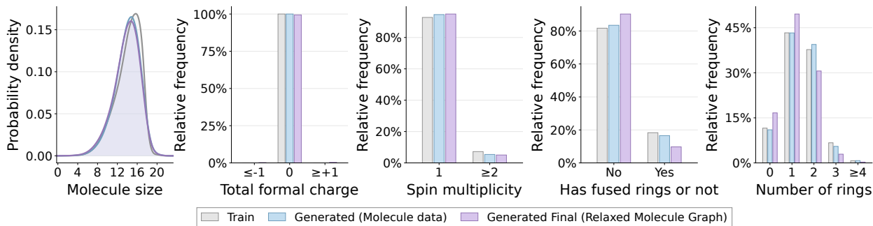
Figure 4: EF-TALFM matches training-set chemical distributions before and after postprocessing. Normalized distributions of atom count, ring count, fused-ring occurrence, spin multiplicity, and total charge are shown for the training data, raw outputs decoded from 100,000 generated latents, and final relaxed molecular graphs.
