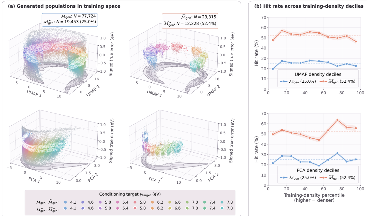
Figure 5: Internal-readout selection increases DFT-verified hit rates across every training-density decile in the learned property representation. The top and bottom rows correspond to fixed uniform manifold approximation and projection (UMAP) and principal component analysis (PCA) mappings of the penultimate molecule-path property representation \mathbf{r} , respectively. Panel (a) compares the screened relaxed population \mathcal{M}_{\text{gen}} (left) with its selected subset \widehat{\mathcal{M}}_{\text{gen}} (right), obtained by retaining the target-wise best 30% ranked by e_{\text{sur}} . The signed true-property error, y_{\text{true}} - y_{\text{target}} is clipped at \pm 1.0 eV. Colors identify the ten conditioning targets. Generation hits with \epsilon_{\text{true}} < 0.1 are shown as white-outlined diamond-shaped markers, whereas misses are represented by round-shaped markers whose target colors progressively fade toward gray with increasing absolute error. The floor shading and contours represent the smoothed density of the full training population; contour boundaries enclose the highest-density regions containing q \in \{1, 10, 50, 90, 99, 99.5\}\% of the training molecules. The corresponding hit populations are \mathcal{M}_{\text{gen}}^* and \widehat{\mathcal{M}}_{\text{gen}}^* . Panel (b) reports the corresponding hit rates across training-density percentile deciles; shaded bands denote 95% Wilson intervals and dashed lines indicate overall hit rates.
