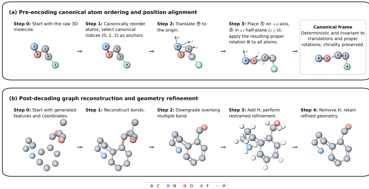
Figure 2: (a) Example preprocessing of molecular data prior to encoding. A C_2H_6FNO conformer from PCQM4Mv2 is shown. Hydrogen atoms are implicit and omitted from the visualization; numbers denote atom-row indices at each stage. (b) Deterministic reconstruction and restrained refinement of a generated heavy-atom configuration. The decoder supplies atom identities and 3D coordinates, together with per-atom and molecule-level attributes, but no molecular graph. Connectivity and valence-compatible bond orders are inferred without changing the generated coordinates. The initial graph contains two connected components: the hatched four-heavy-atom propylene oxide fragment is discarded, whereas the 12-heavy-atom component is retained. Brown marks an initially assigned C=C bond whose length is inconsistent with a carbon-carbon double bond. Demotion to C-C (green) dearomatizes the ring. Aromatic bonds before correction are depicted by a solid bond with a thin dashed inner line. Explicit hydrogens are subsequently added for fixed-topology, restrained refinement; dashed element-colored outlines indicate the pre-refinement heavy-atom positions. Finally, the temporary hydrogens are removed while retaining the refined heavy-atom coordinates.
