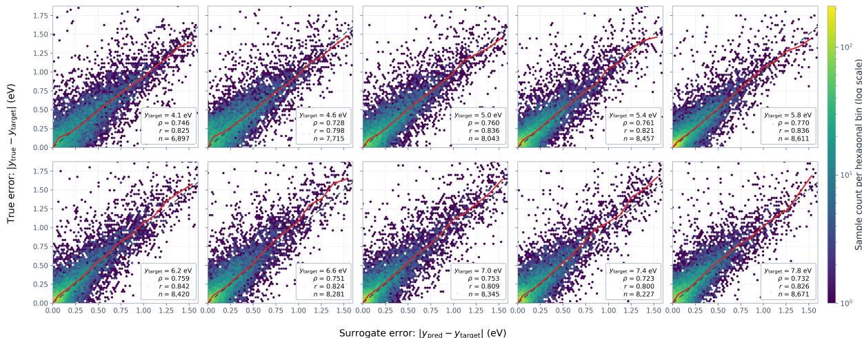
Figure 9: The internal-readout property error is a strong and practically useful indicator of the true error. For conditionally generated molecules across 10 target HOMO-LUMO gaps, the internal-readout and true errors are strongly correlated, with Spearman \rho = 0.728 –0.770 and Pearson r = 0.798 –0.842. The binned-median trend (red solid line) broadly follows the diagonal x = y (dashed line), showing that molecules with smaller internal-readout errors tend to have true properties closer to their targets.
