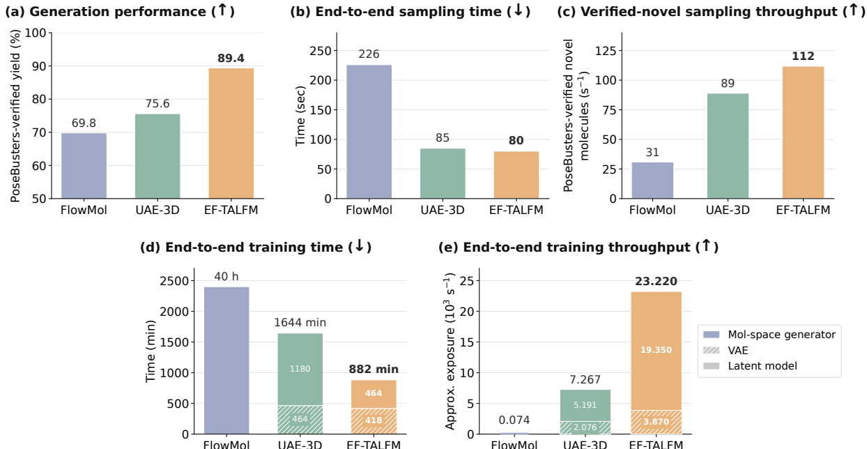
Figure 3: Generation quality and end-to-end computational efficiency on PCQM4Mv2. Arrows indicate the better performance. Panel (a) shows that EF-TALFM achieves the highest PoseBusters-verified novel yield among the 10,000 molecules generated by each method, which counts unique, training-set-novel samples that pass sanitization and all six PoseBusters geometry checks. Panel (b) shows that EF-TALFM generates the 10,000 molecules in the shortest end-to-end time, including time for generator sampling, reconstruction, and relaxation. Panel (c) then shows that EF-TALFM delivers the highest sampling throughput, for PoseBusters-verified novel molecules, shown in panel (a). Panel (d) shows that EF-TALFM requires the shortest end-to-end training time while achieving the highest end-to-end training throughput. This pipeline-average rate divides approximate exposure by total training time, with stacked segments showing stage contributions. FlowMol’s displayed rate uses a molecule-equivalent proxy derived from its edge-level exposure; because the exposure units are not directly interchangeable, panel (e) contextualizes data-processing throughput rather than providing a FLOP-matched comparison.
