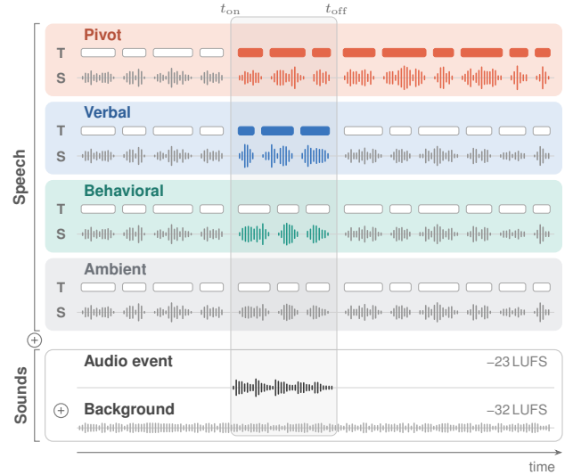
Fig. 1. Four types of speaker reaction to an audio event. Each block shows the transcript (T, one box per word) and the speech signal (S) over time. The shaded box marks the audio event [t_{on}, t_{off}] . Colored elements are altered by the event. Pivot : persistent change of T and S. Verbal : local verbal reaction (T and S). Behavioral : local change of S only. Ambient : no impact. The speech signal, the audio event ( -23 LUFS) and the background ( -32 LUFS) are summed ( \oplus ) to form the final mix.
