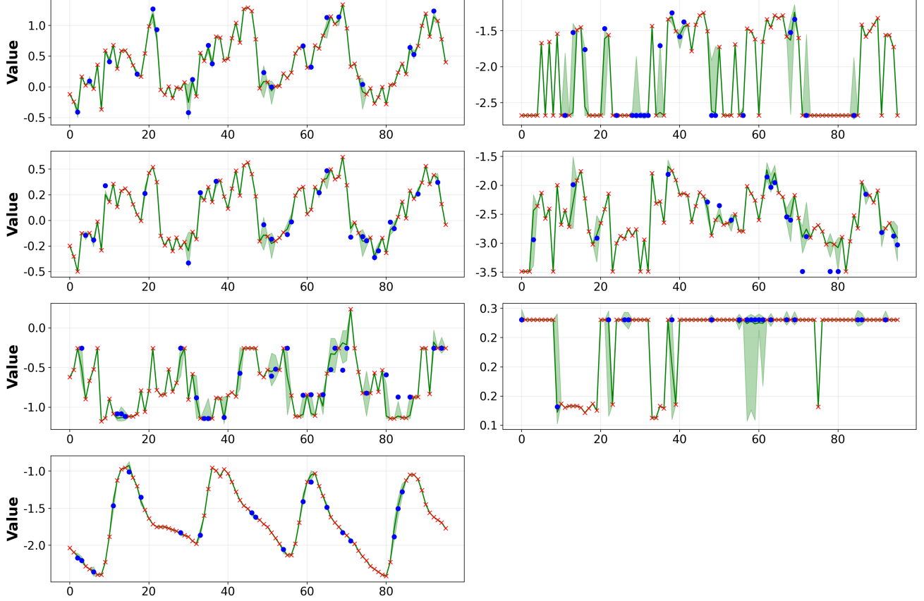
Fig. 4: Visualization of probabilistic imputation results on ETTh2 (20% missingness). The results are for a time series sample with all 7 features. The median and 90% predictive intervals are shown in green, observed points in red and targets in blue.
