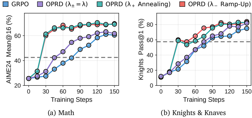
Figure 7: Comparison of three branch-scheduling strategies. We compare the default \lambda_- ramp-up ( \lambda_+ = 0.5 , \lambda_- : 0 \rightarrow 0.5 ), \lambda_+ annealing ( \lambda_+ : 0.5 \rightarrow 0 , \lambda_- = 0 ), and fixed symmetric scaling ( \lambda_+ = \lambda_- = 1.0 ) against GRPO. The two scheduled variants use horizons of 30 updates for Math and 75 updates for Knights & Knaves. We use Qwen3-4B and Qwen3-4B-Base teacher checkpoints obtained after 75 and 105 RL training steps, respectively. Gray dashed lines denote teacher performance. All other training configurations follow Appendix C .
