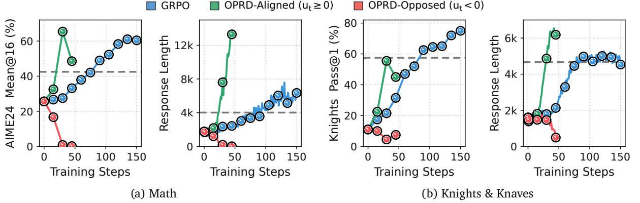
Figure 6: Evaluation performance and response length over training for OPRD variants with only the positive- or negative-alignment branch active. For Math and Knights & Knaves, we use Qwen3-4B and Qwen3-4B-Base teacher checkpoints obtained after 75 and 105 RL training steps, respectively. The two single-branch OPRD variants are trained for 45 steps with \lambda = 0.5 , while GRPO is shown through 150 steps for reference. The maximum generation lengths are 20K and 8K tokens for the two settings, respectively. The gray dashed lines denote the performance or response length of the corresponding weak teachers. All other training settings follow the dataset-specific default configurations described in Appendix C.
