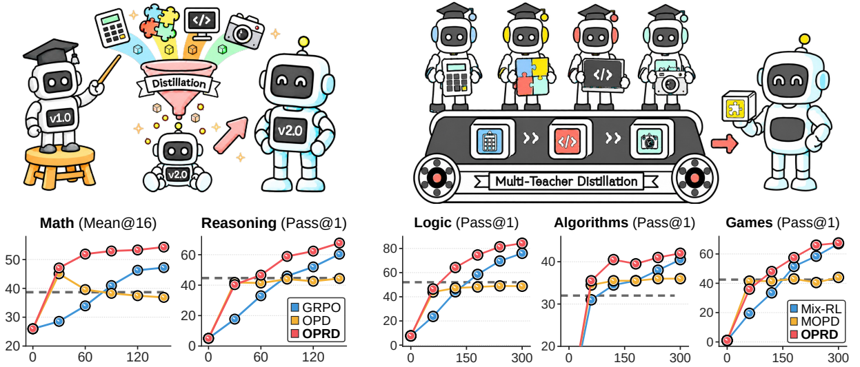
Figure 1: On-policy reverse distillation (OPRD) enables faster and stronger weak-to-strong generalization across two key settings. (Left) For successive model transfer, a checkpoint from a post-trained 4B-scale model serves as the teacher for an 8B-scale student. We average evaluations conducted every 30 training steps: Mean@16 over AIME’24, AIME’25, HMMT’25, and OlympiadBench for math, and Pass@1 over Knights & Knaves, Quantum Lock, String Manipulation, and Countdown for reasoning tasks. (Right) In multi-domain consolidation, four domain-specialized 4B-scale teachers are distilled into a single 8B-scale student. Training examples are randomly mixed within each batch, with the corresponding domain teacher activated for each example. We report performance every 60 steps for Logic (averaged over Knights & Knaves and Quantum Lock), Algorithms (String Manipulation), and Games (Countdown). The gray dashed lines denote the performance of the corresponding weak teachers.
