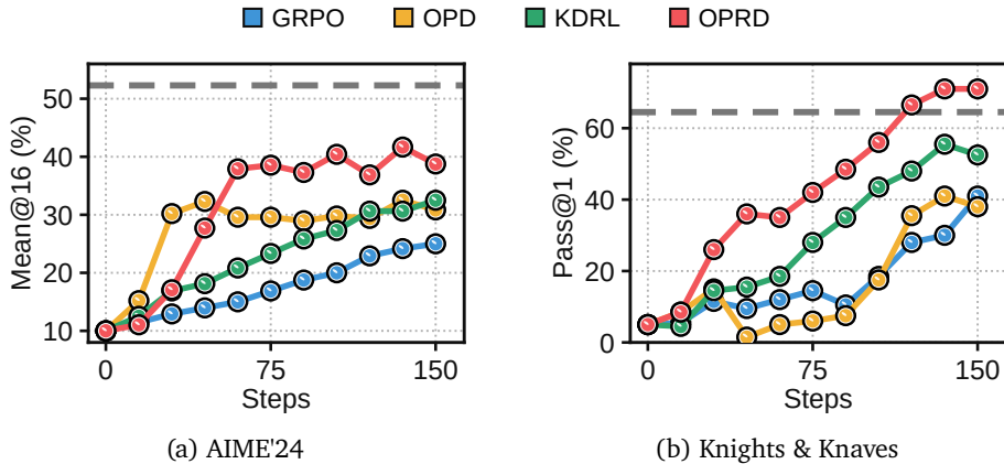
Figure 13: Learning curves for strong-to-weak distillation on two tasks. We evaluate Qwen3-8B \rightarrow Qwen3-1.7B on AIME'24 and Qwen3-8B-Base \rightarrow Qwen3-0.6B on Knights & Knaves, using teachers from step 105 of task-specific GRPO. Gray dashed lines mark teacher performance. All other settings follow Appendix C, with method-specific distillation coefficients scheduled over the first 45 updates.
