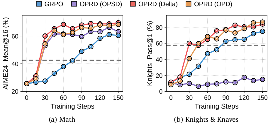
Figure 16: Comparison of guidance-direction constructions. The variants construct \mathbf{d}_t from the teacher–reference policy shift (Delta), the teacher–student mismatch (OPD), or the privileged-context discrepancy (OPSD). Using stronger teacher checkpoints than those used in Figure 3a , we pair the step-75 Qwen3-4B teacher with a Qwen3-8B student for Math and the step-105 Qwen3-4B-Base teacher with a Qwen3-8B-Base student for Knights & Knaves. Gray dashed lines mark teacher performance. All other training configurations follow Appendix C .
