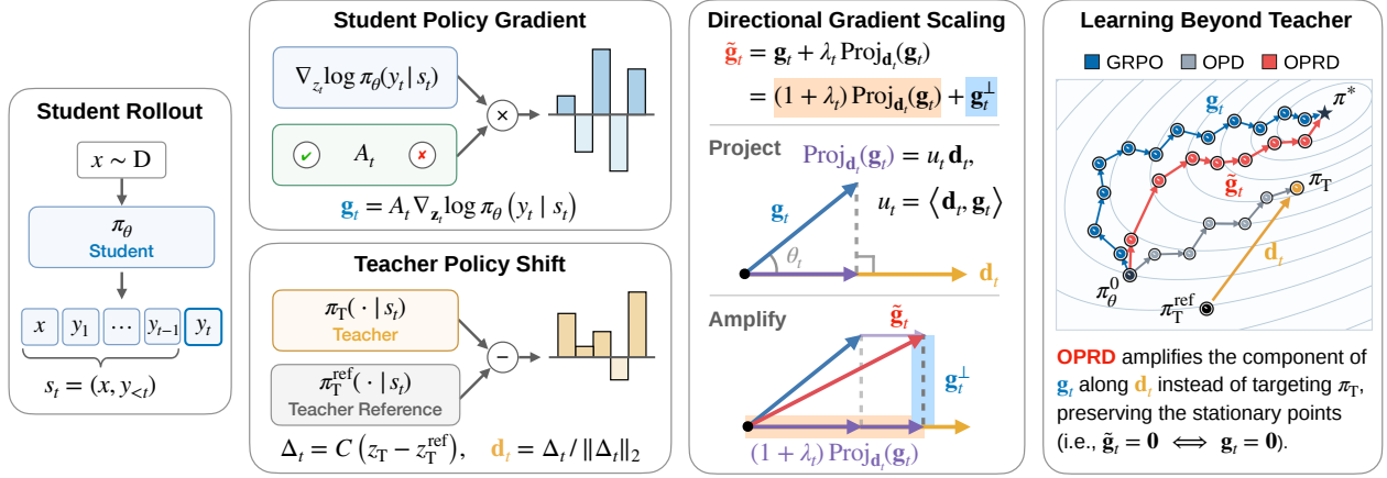
Figure 2: Conceptual overview of On-Policy Reverse Distillation (OPRD). The figure illustrates OPRD’s gradient correction procedure for a single query. Here, \mathbf{z}_T denotes the logits of the weak teacher after post-training and \mathbf{z}_T^{\text{ref}} those of its reference policy, and C denotes mean-centering. Their centered difference \Delta_t is the teacher’s policy shift at that student-visited prefix, and OPRD keeps only its unit direction \mathbf{d}_t . In practice, we use a simple top-10 truncation under the student policy to focus the correction on its high-probability vocabulary region. The rightmost panel provides a conceptual view of the resulting student trajectory in the optimization landscape, where the student follows the verifier-driven policy gradient g_t with its component along \mathbf{d}_t amplified by 1 + \lambda_t at each token and its orthogonal component left unchanged.
