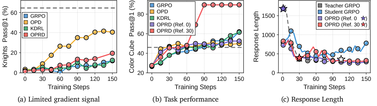
Figure 4: (a) Results under limited policy-gradient signal. On Knights & Knaves, we transfer a step-105 Qwen3-8B-Base teacher to a Qwen3-1.7B-Base student, with OPRD’s negative-branch scale \lambda_t warmed up over the first 75 steps. (b, c) Effect of reference-policy selection on length bias. On Color Cube, we transfer a step-105 Qwen3-4B-Base teacher \pi_T to a Qwen3-8B-Base student, using either the step-0 or step-30 checkpoint from the same GRPO run as \pi_T^{\text{ref}} . OPRD’s negative-branch scale \lambda_t is warmed up over the first 75 steps. The gray dashed line marks teacher performance, while the colored stars denote the mean response lengths of the two choices of \pi_T^{\text{ref}} , and the white star marks that of \pi_T . All other settings follow Section 3.1.
