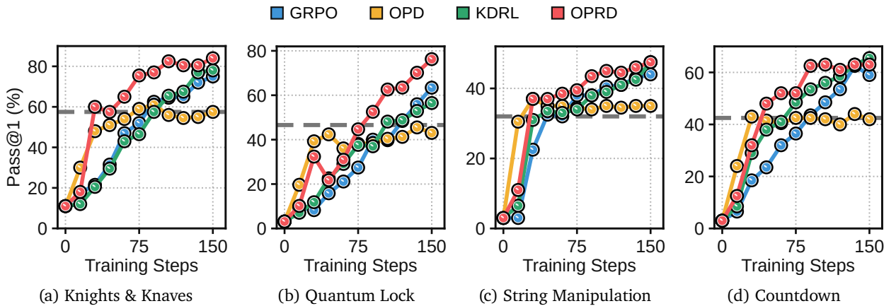
Figure 9: Learning curves for successive model transfer on individual reasoning benchmarks. We use Qwen3-4B-Base as the teacher and Qwen3-8B-Base as the student. The gray dashed line denotes the performance of the weak teacher. All training settings follow the default Reasoning Gym configuration described in Appendix C.
