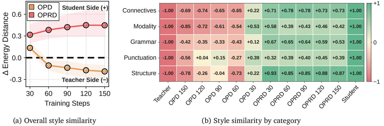
Figure 18: (a) Comparing response style distributions over training. Energy-distance differences are averaged across 30 AIME'24 problems, with positive values indicating greater similarity to the GRPO student and negative values to the teacher. Shading shows 95% confidence intervals from 2,000 bootstrap resamples of the problems. (b) Measuring similarity to teacher and student response styles. Normalized distance differences compare average styles in five categories, with red indicating greater similarity to the teacher and green to the GRPO student. Both panels use fixed references: the Qwen3-4B teacher at GRPO update 75 and the Qwen3-8B GRPO student at update 150.
