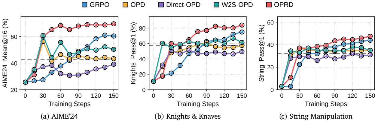
Figure 15: Training dynamics of weak-to-strong methods using the weak policy delta. The horizontal dashed lines indicate weak-teacher performance. See Appendix G.1 for baseline implementation details.
