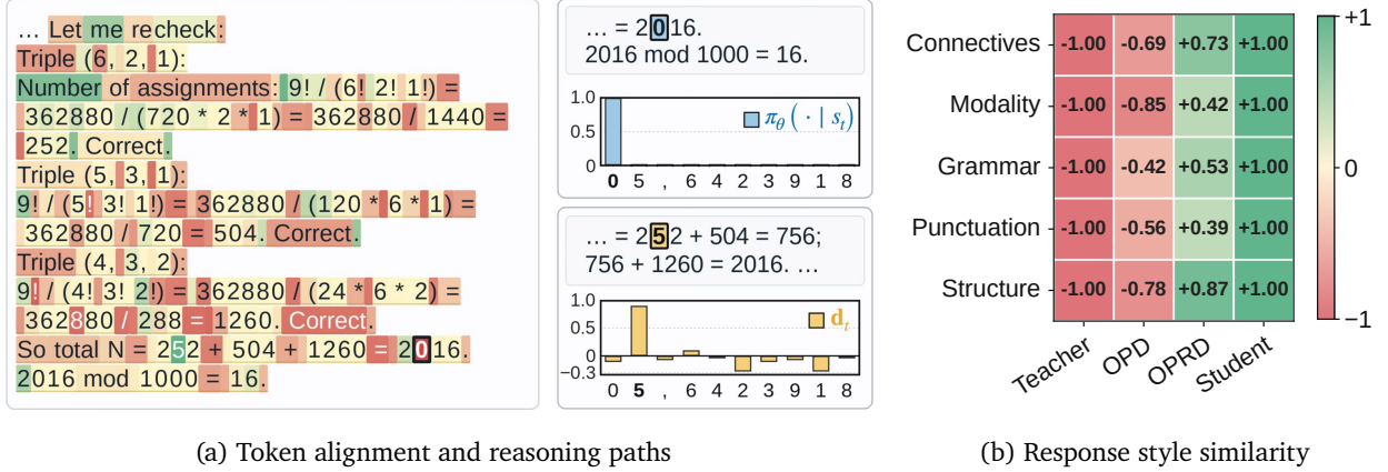
Figure 5: (a) Visualizing token alignment and reasoning continuations. An AIME'25 response from the OPRD student at update 150. Green and red indicate positive and negative cosine similarity between d_t and the student policy gradient g_t with A_t = 1 , respectively (see Appendix J.1). The token outlined in black, 0 , has the lowest cosine similarity among displayed tokens. The student's top-1 token 0 completes 2016 directly. Forcing 5 , the top-1 token under d_t , leads the same student to this result through an intermediate sum. The plots show the student's top-10 token probabilities above and their teacher-shift values ( d_t ) below. (b) Measuring similarity to teacher and student response styles. On AIME'24, we compare response styles using 101 standardized features across five categories. Normalized distance differences indicate whether each method's average style is closer to the weak teacher (red) or the GRPO-trained student at update 150 (green).
