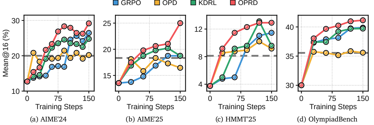
Figure 10: Learning curves on individual math benchmarks using Qwen3-Base models. We use Qwen3-4B-Base as the teacher and Qwen3-8B-Base as the student. The gray dashed line denotes the performance of the weak teacher. All other settings follow the default Math configuration in Appendix C , but we omit the system prompt and reduce the mini-batch size to 32, yielding two optimizer steps per training batch.
