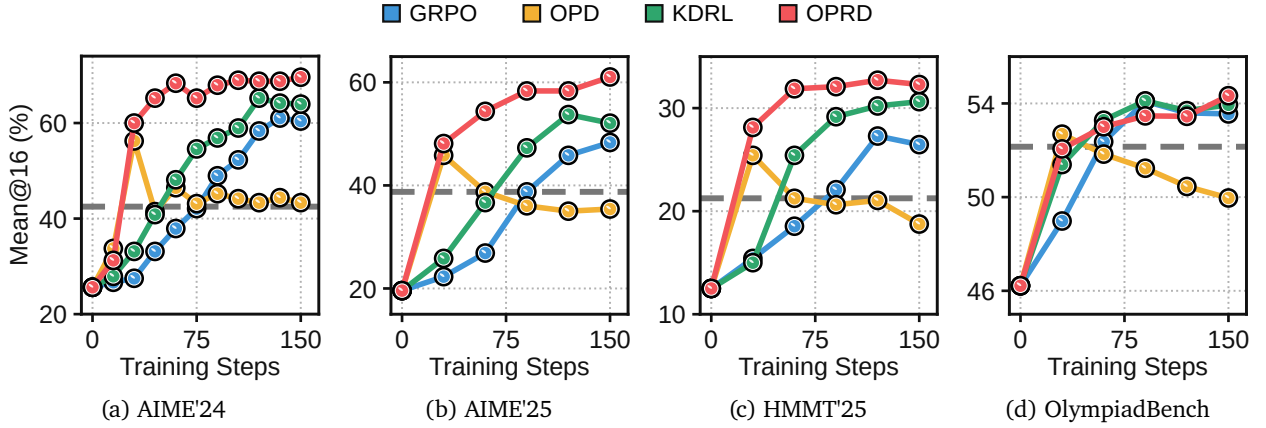
Figure 8: Learning curves for successive model transfer on individual math benchmarks. We use Qwen3-4B as the teacher and Qwen3-8B as the student. The gray dashed line denotes the performance of the weak teacher. All training settings follow the default Math configuration described in Appendix C.
