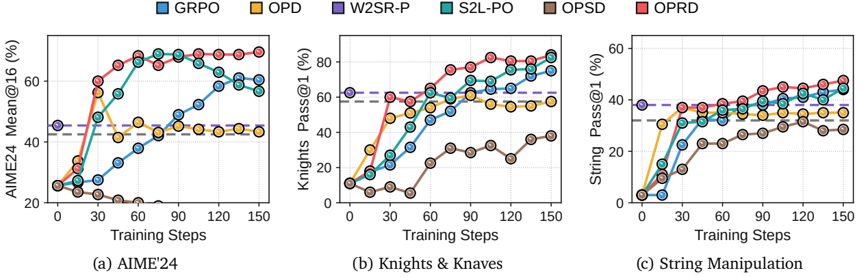
Figure 14: Training dynamics of weak-to-strong methods using off-policy generations from the weak teacher. Because W2SR-P performs SFT without subsequent RL, its final performance is shown as a horizontal dashed line. The gray dashed lines indicate weak-teacher performance. See Appendix G.1 for baseline implementation details.
