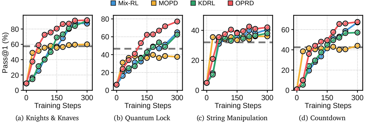
Figure 12: Learning curves on individual Reasoning Gym tasks under multi-teacher distillation. We use four task-specific Qwen3-4B-Base models as teachers and jointly train a Qwen3-8B-Base student. The gray dashed line denotes the performance of the corresponding specialist teacher. All other settings follow the configurations described in Section C.
