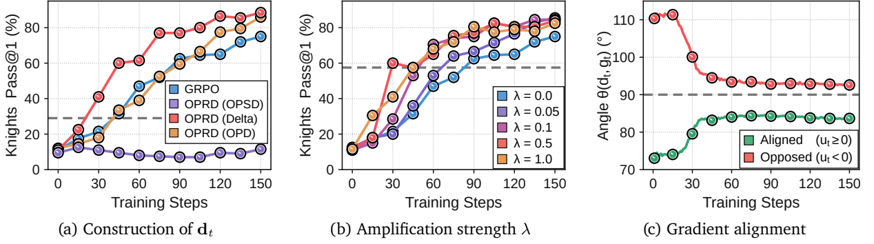
Figure 3: (a) Ablations of scaling-direction construction. All OPRD variants use the step-60 GRPO checkpoint as the weak teacher. For OPSD, a verified draft generated by this teacher is provided as privileged context. (b) Ablation of directional amplification strength. We vary \lambda , the coefficient applied to OPRD’s directional correction term. \lambda = 0 corresponds to GRPO. The gray dashed line marks the performance of the teacher checkpoint. All other settings follow the default configurations in Section 3.1. (c) Alignment dynamics between d_t and g_t . On Knights & Knaves, we track \theta_t between d_t and g_t during OPRD with a Qwen3-8B-Base student and Qwen3-4B-Base weak teacher. Excluding rollout groups with g_t = 0 (identical rewards within the group), we report token-averaged angles for aligned ( u_t \geq 0 ) and opposed ( u_t < 0 ) tokens.
