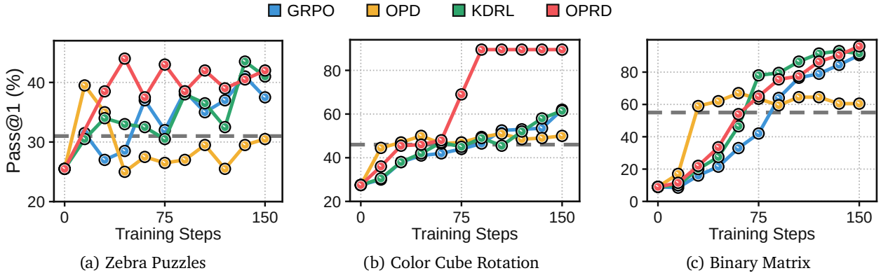
Figure 11: Learning curves on additional three Reasoning Gym tasks. We use Qwen3-4B-Base as the teacher and Qwen3-8B-Base as the student. The gray dashed line denotes the performance of the weak teacher. For Color Cube Rotation and Binary Matrix, we use the teacher checkpoints from steps 30 and 45, respectively, as the reference policies instead of the raw step-0 models to mitigate length bias (see Appendix I for details).
