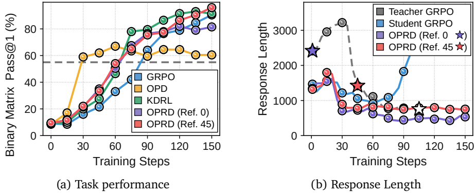
Figure 17: Effect of reference-policy selection on length bias in Binary Matrix. We transfer a step-105 Qwen3-4B-Base teacher \pi_T to a Qwen3-8B-Base student, using either the step-0 or step-45 checkpoint from the same GRPO run as \pi_T^{\text{ref}} . OPRD’s negative-branch scale \lambda_t is warmed up over the first 75 steps. The gray dashed line marks teacher performance, while the colored stars denote the mean response lengths of the two choices of \pi_T^{\text{ref}} , and the white star marks that of \pi_T . All other settings follow Appendix C.
