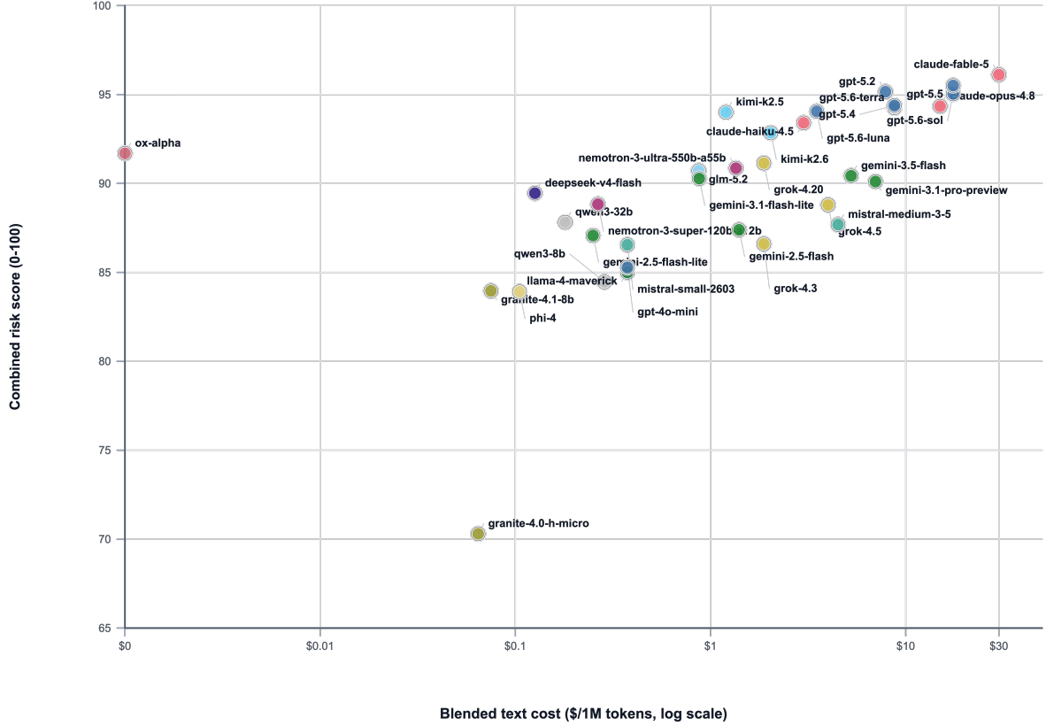
Figure 4. Combined-risk performance in relation to model inference cost. Each point represents the highest-overall-scoring evaluated configuration for one base model. The horizontal axis shows blended text cost in US dollars per one million tokens on a logarithmic scale, and the vertical axis shows combined-risk score on the 0–100 scale. Labels identify base models and colours distinguish provider families. Cost reflects the pricing inputs used for the public leaderboard and should be interpreted as a comparative estimate for the evaluated configuration.
