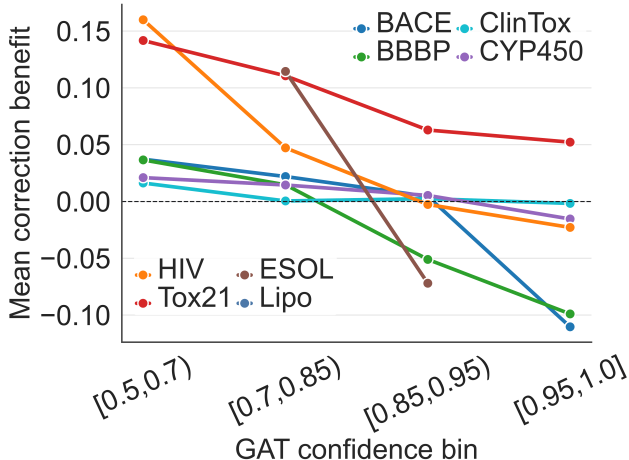
Figure 3: Confidence-binned behavior. Mean correction benefit is largest in lower-confidence GAT bins and shrinks as the GAT becomes more confident.
