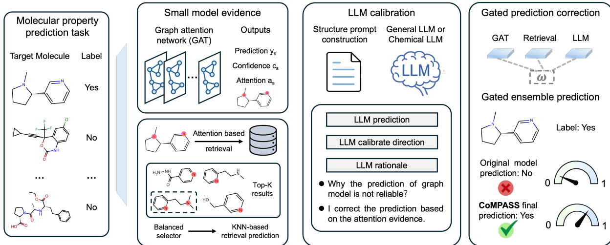
Figure 1: CoMPASS overview . A GAT produces the base prediction and attention evidence. Retrieval supplies top- K calibration molecules. The LLM proposes an evidence-conditioned correction, and a bounded gate controls how much that proposal changes the final prediction.
