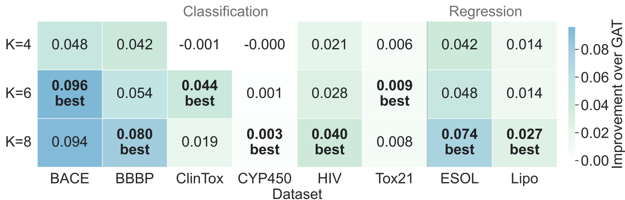
Figure 2: Main-result heatmap over retrieval size. Cells show improvement over the GAT baseline in each dataset’s metric units: ROC-AUC points for classification and original-scale RMSE reduction for regression.
