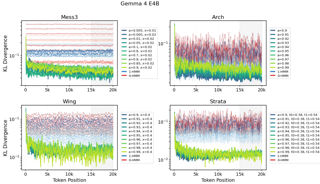
Figure 21: Gemma 4 E4B : KL divergence between the LLM's next-token probabilities (NTP) and full HMM's ground-truth NTP, alongside that between the order-1's and order-0's ground-truth NTP and the full HMM's, for all 40 HMMs.
