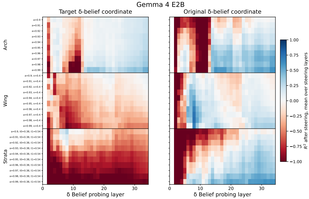
Figure 64: Gemma 4 E2B : Post-steering \delta -coordinate decodability across all HMM parametrizations. Each cell reports the R^2 of a probe applied to steered activations, averaged over all steering layers at least two layers below the probing layer. The probe is fit on unsteered activations to decode the original beliefs' \delta -coordinate and is applied unchanged after steering, and its predictions are scored against the target beliefs' \delta -coordinate ( left ) and the original beliefs' \delta -coordinate ( right ). Rows index HMM parametrizations grouped by family; columns index the probing layer. Blue indicates positive R^2 , red negative. The first two columns are undefined, as no steering layer lies at least two layers below. Mess3 is absent, as its full-rank M admits no NTP-preserving direction. Values are means across 10 sequences.
