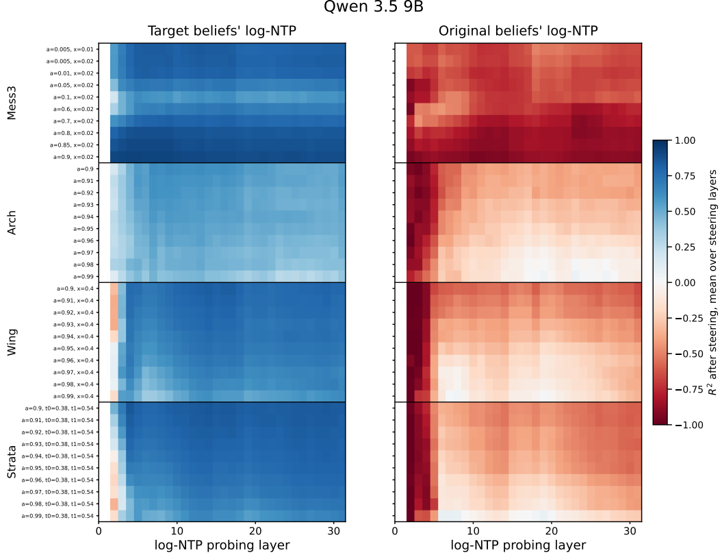
Figure 53: Qwen 3.5 9B : Post-steering decodability across all HMM parametrizations. Each cell reports the R^2 of a probe applied to steered activations, averaged over all steering layers at least two layers below the probing layer. The probe is fit on unsteered activations to decode the original beliefs' implied log-NTP and is applied unchanged after steering, and its predictions are scored against the target beliefs' implied log-NTP ( left ) and the original beliefs' implied log-NTP ( right ). Rows index HMM parametrizations grouped by family; columns index the probing layer. Blue indicates positive R^2 , red negative. The first two columns are undefined, as no steering layer lies at least two layers below. Values are means across 10 sequences.
