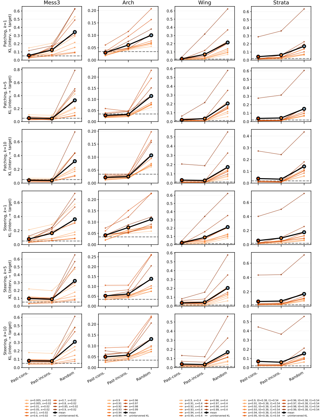
Figure 72: Qwen 3.5 4B : KL between the intervened prediction and the injected target belief's NTP, averaged over the final 70% of layers, for each parametrization (orange lines; black = mean). Rows are intervention type and k -suffix length (patching then steering, k \in \{1, 5, 10\} ); columns are HMM families. Lower means the prediction moved closer to the injected belief. The dashed gray line marks the model's unintervened KL to the ground-truth NTP, a reference for how closely the model tracks a target it follows; for the random condition, the target is the stationary belief's NTP.
