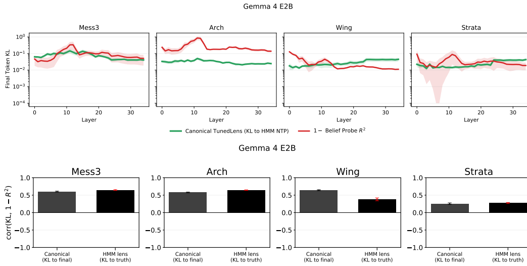
Figure 82: Gemma 4 E2B : Top : canonical lens KL to HMM ground truth (green) vs. 1 - R^2 (red), by layer. Mean over parametrizations; bands \pm 1 std. Bottom : per-sequence Pearson correlation between each lens’s KL-by-layer curve and 1 - R^2 of the belief probe (mean over 10 parametrizations \times 10 seeds; error bars 95% CI): the canonical lens scored on its training objective, KL to the model’s final-layer distribution ( left bar ), and the ground-truth-supervised lens of Section 8 scored on KL to the ground truth ( right bar ).
