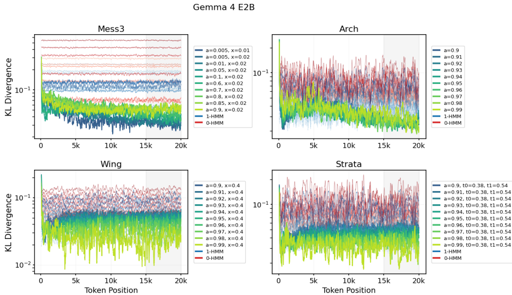
Figure 22: Gemma 4 E2B : KL divergence between the LLM's next-token probabilities (NTP) and full HMM's ground-truth NTP, alongside that between the order-1's and order-0's ground-truth NTP and the full HMM's, for all 40 HMMs.
