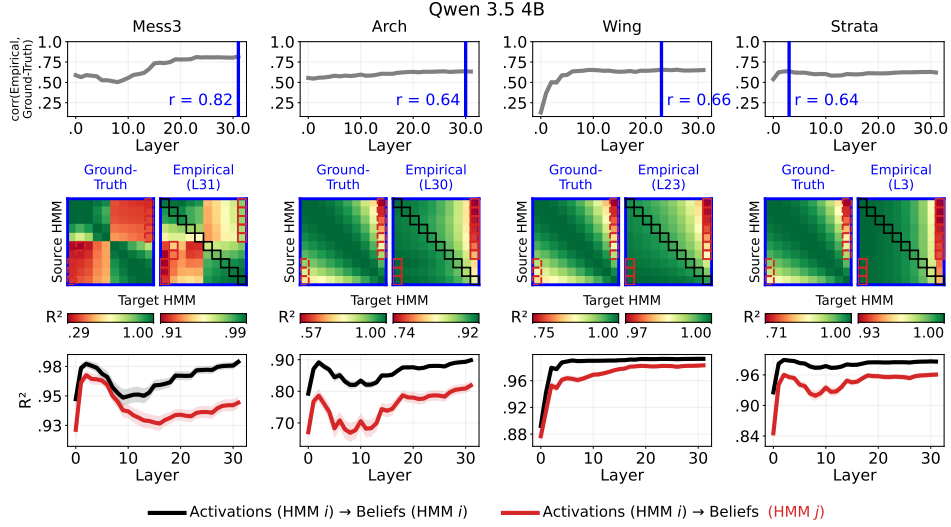
Figure 36: Qwen 3.5 4B : Probes fit to beliefs of HMMs that were not the HMM that generated the token sequence. HMM j (bordered red in the heatmaps) is the parametrization whose ground-truth transfer R^2 is lowest from activations on HMM i 's sequence. The last row of plots shows that predicting HMM j 's beliefs from activations on HMM i 's sequence is poorer than predicting HMM i 's beliefs.
