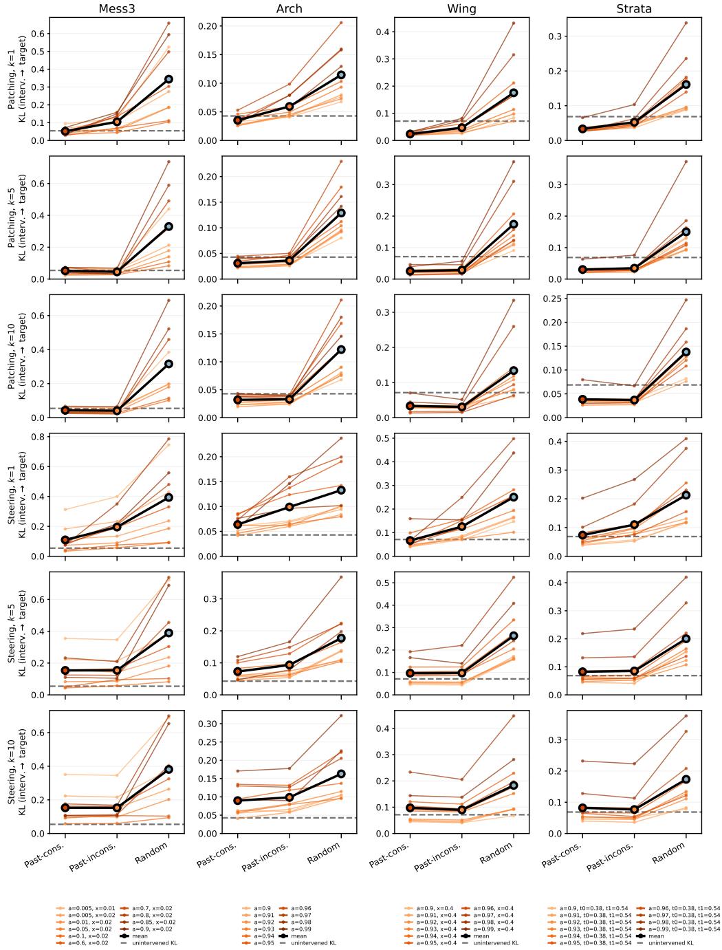
Figure 74: Llama 3.2 3B : KL between the intervened prediction and the injected target belief’s NTP, averaged over the final 70% of layers, for each parametrization (orange lines; black = mean). Rows are intervention type and k -suffix length (patching then steering, k \in \{1, 5, 10\} ); columns are HMM families. Lower means the prediction moved closer to the injected belief. The dashed gray line marks the model’s unintervened KL to the ground-truth NTP, a reference for how closely the model tracks a target it follows; for the random condition, the target is the stationary belief’s NTP.
