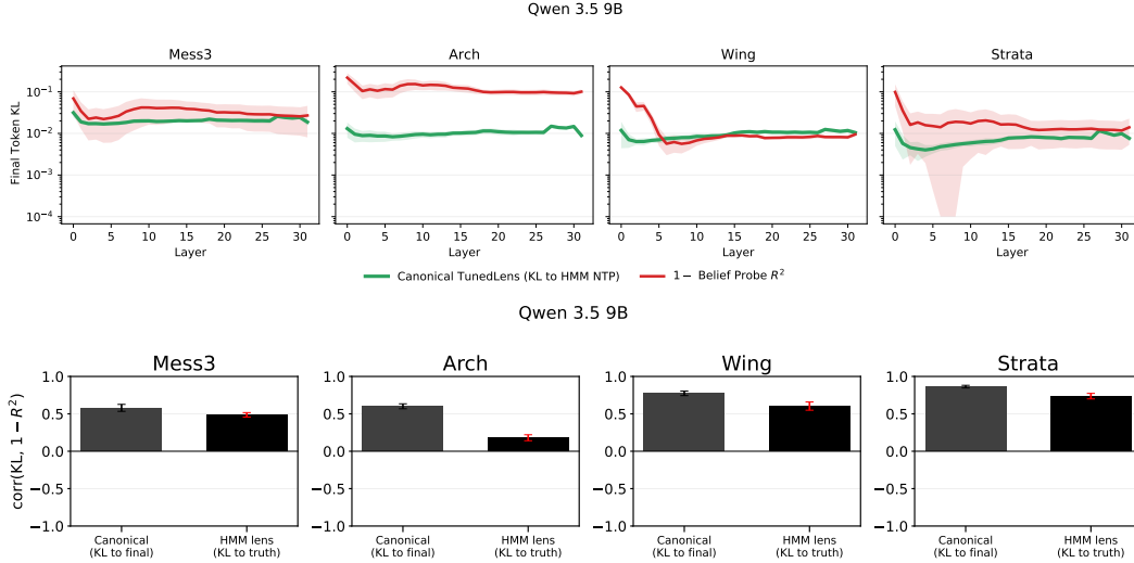
Figure 77: Qwen 3.5 9B: Top: canonical lens KL to HMM ground truth (green) vs. 1 - R^2 (red), by layer. Mean over parametrizations; bands \pm 1 std. Bottom: per-sequence Pearson correlation between each lens’s KL-by-layer curve and 1 - R^2 of the belief probe (mean over 10 parametrizations \times 10 seeds; error bars 95% CI): the canonical lens scored on its training objective, KL to the model’s final-layer distribution ( left bar ), and the ground-truth-supervised lens of Section 8 scored on KL to the ground truth ( right bar ).
