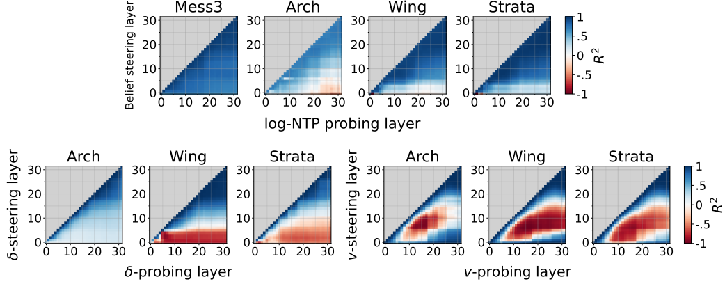
Figure 6: Belief state steering moves log-NTP decodability, and NTP-preserving belief steering moves the belief’s NTP-invisible component. Top : Each cell reports the R^2 of probes decoding the target beliefs’ implied log-NTP, across belief steering layers (rows) and probing layers (columns). Bottom : We steer to targets \eta_{\text{target}} = \eta_{\text{original}} + \delta with \delta M = 0 (left) or steer activations along a random direction v with matched magnitude (right) and report the R^2 of probes decoding the steered component of the target beliefs. We exclude Mess3, as its M is invertible and no \delta exists. Blue indicates decodability and red indicates lack of decodability. Values are means across 10 sequences.
