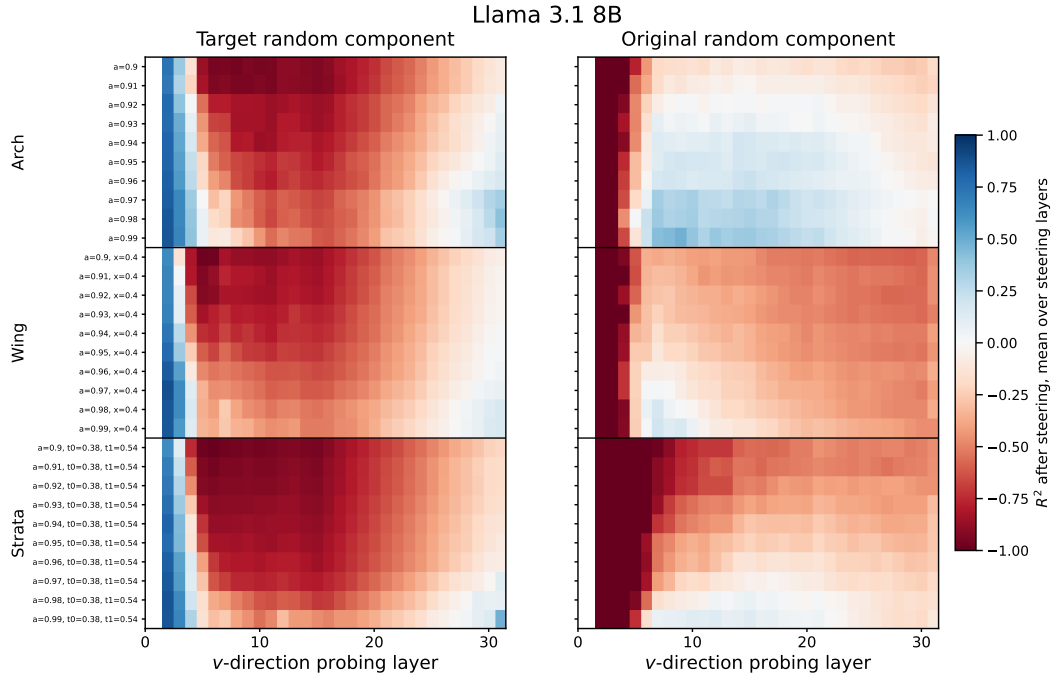
Figure 67: Llama 3.1 8B : Post-steering v -component decodability across all HMM parametrizations. Each cell reports the R^2 of the projection of steered activations onto the random direction v , averaged over all steering layers at least two layers below the probing layer, scored against the pre-steering projection plus the injected magnitude ( left , the target component) and against the pre-steering projection ( right , the original component). Rows index HMM parametrizations grouped by family; columns index the v -direction probing layer. Blue indicates positive R^2 , red negative. The first two columns are undefined, as no steering layer lies at least two layers below. Mess3 is absent, as the steer magnitudes are matched to the \delta -belief steer, which requires a rank-deficient M . Values are means across 10 sequences.
