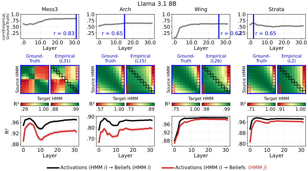
Figure 37: Llama 3.1 8B : Probes fit to beliefs of HMMs that were not the HMM that generated the token sequence. HMM j (bordered red in the heatmaps) is the parametrization whose ground-truth transfer R^2 is lowest from activations on HMM i 's sequence. The last row of plots shows that predicting HMM j 's beliefs from activations on HMM i 's sequence is poorer than predicting HMM i 's beliefs.
