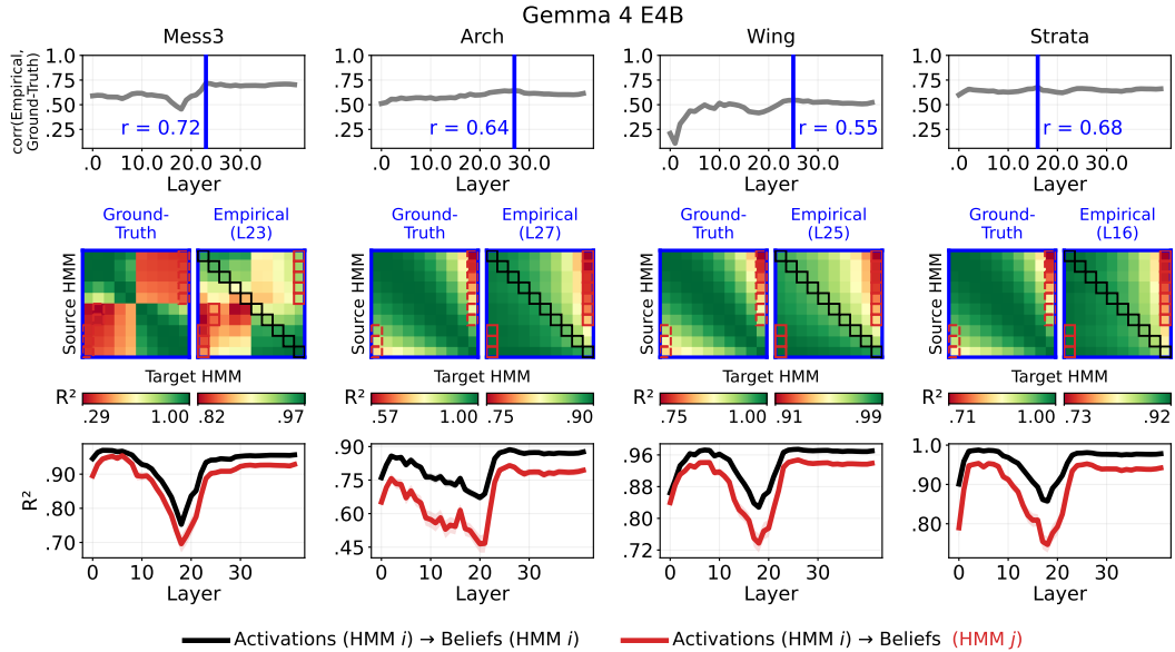
Figure 39: Gemma 4 E4B : Probes fit to beliefs of HMMs that were not the HMM that generated the token sequence. HMM j (bordered red in the heatmaps) is the parametrization whose ground-truth transfer R^2 is lowest from activations on HMM i 's sequence. The last row of plots shows that predicting HMM j 's beliefs from activations on HMM i 's sequence is poorer than predicting HMM i 's beliefs.
