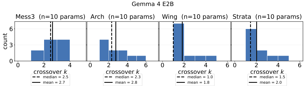
Figure 28: Gemma 4 E2B : Distribution of the crossover order k across the 10 parametrizations of each HMM family. The crossover k is the smallest Markov order whose k -HMM predictor matches the LLM’s converged KL—the first k at which the k -HMM’s KL to the full HMM falls to the LLM’s. Dashed and solid lines mark the median and mean.
