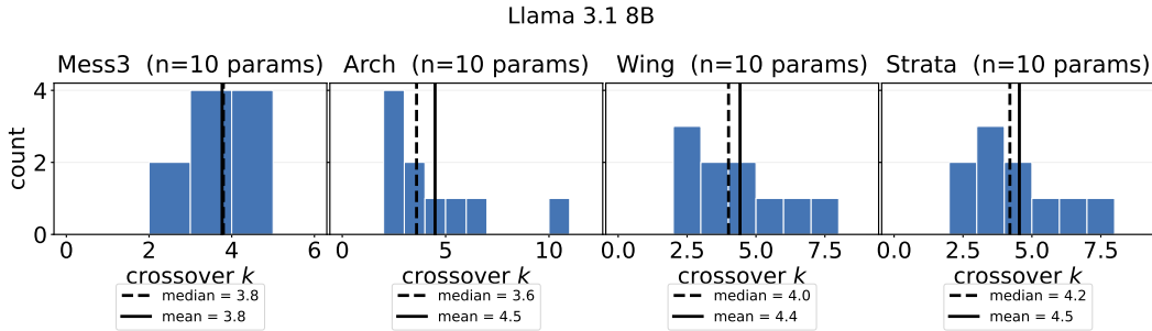
Figure 25: Llama 3.1 8B : Distribution of the crossover order k across the 10 parametrizations of each HMM family. The crossover k is the smallest Markov order whose k -HMM predictor matches the LLM’s converged KL—the first k at which the k -HMM’s KL to the full HMM falls to the LLM’s. Dashed and solid lines mark the median and mean.
