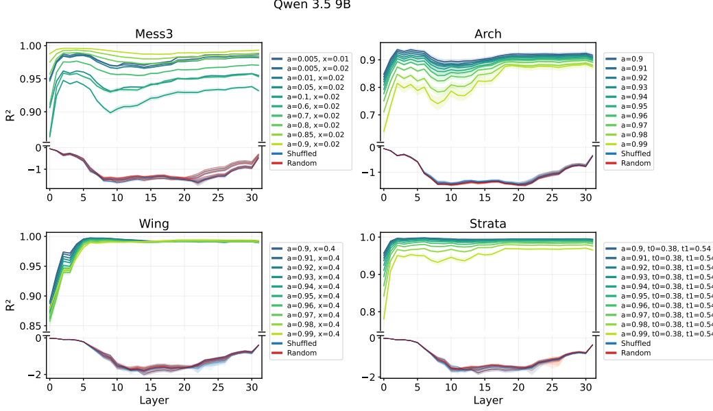
Figure 29: Qwen 3.5 9B : All 40 HMM linear probe fits, including fits to each HMM’s corresponding shuffled belief and random belief controls.
