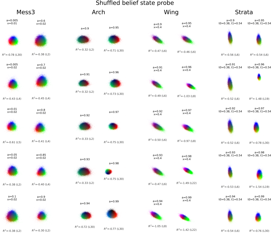
Figure 13: Geometries recovered by control probes trained on shuffled belief states, with their fit (held-out R^2 , averaged over 10 sequences) at each HMM's best-fitting layer in Qwen 3.5 9B, for all 10 sequences as in Figure 11. No structure is recovered.
