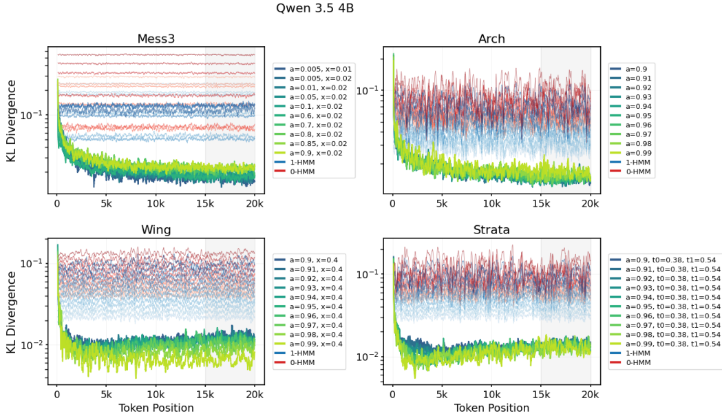
Figure 18: Qwen 3.5 4B : KL divergence between the LLM’s next-token probabilities (NTP) and full HMM’s ground-truth NTP, alongside that between the order-1’s and order-0’s ground-truth NTP and the full HMM’s, for all 40 HMMs.
