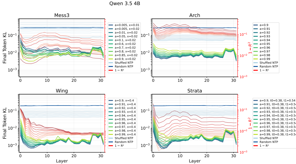
Figure 84: Qwen 3.5 4B : For every parametrization of each family, the per-layer KL of the tuned lens to the HMM ground-truth NTP (colored by parametrization, left axis) shown against the belief probe’s 1 - R^2 (red, right axis). Lenses trained to shuffled- and random-NTP controls (light/dark blue) stay high across all layers.
