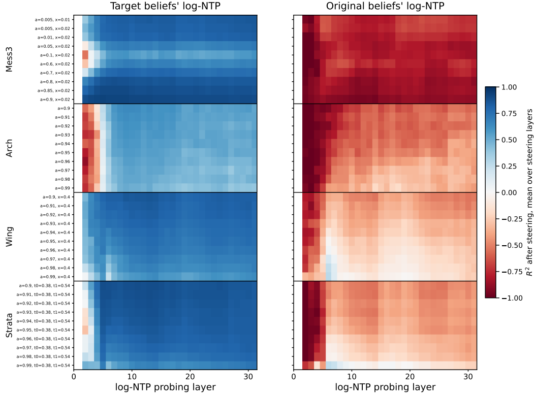
Figure 54: Qwen 3.5 4B : Post-steering decodability across all HMM parametrizations. Each cell reports the R^2 of a probe applied to steered activations, averaged over all steering layers at least two layers below the probing layer. The probe is fit on unsteered activations to decode the original beliefs' implied log-NTP and is applied unchanged after steering, and its predictions are scored against the target beliefs' implied log-NTP ( left ) and the original beliefs' implied log-NTP ( right ). Rows index HMM parametrizations grouped by family; columns index the probing layer. Blue indicates positive R^2 , red negative. The first two columns are undefined, as no steering layer lies at least two layers below. Values are means across 10 sequences.
