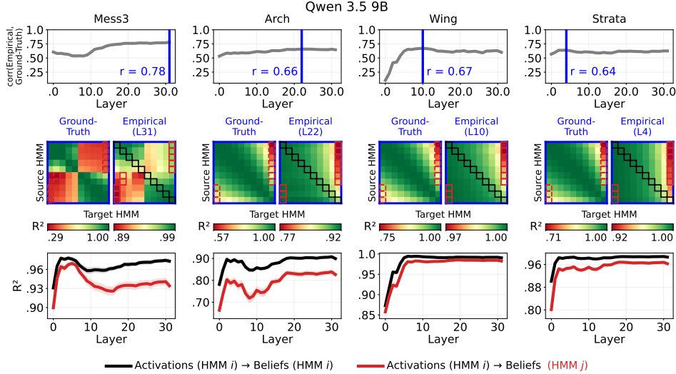
Figure 35: Qwen 3.5 9B: Probes fit to beliefs of HMMs that were not the HMM that generated the token sequence. HMM j (bordered red in the heatmaps) is the parametrization whose ground-truth transfer R^2 is lowest from activations on HMM i 's sequence. The last row of plots shows that predicting HMM j 's beliefs from activations on HMM i 's sequence is poorer than predicting HMM i 's beliefs.
