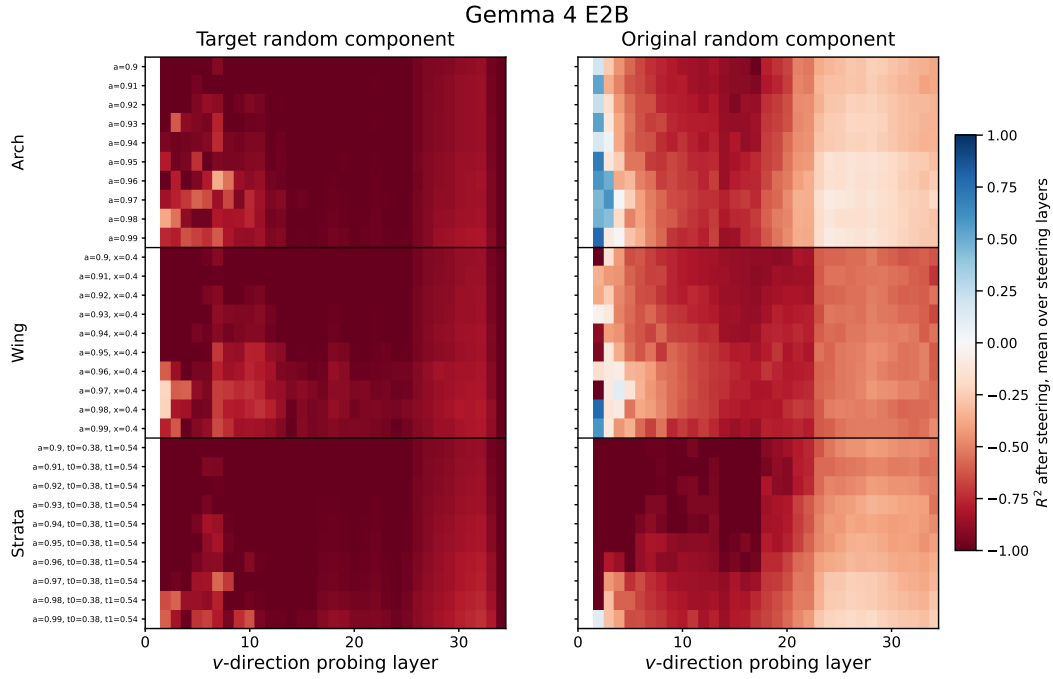
Figure 70: Gemma 4 E2B : Post-steering v -component decodability across all HMM parametrizations. Each cell reports the R^2 of the projection of steered activations onto the random direction v , averaged over all steering layers at least two layers below the probing layer, scored against the pre-steering projection plus the injected magnitude ( left , the target component) and against the pre-steering projection ( right , the original component). Rows index HMM parametrizations grouped by family; columns index the v -direction probing layer. Blue indicates positive R^2 , red negative. The first two columns are undefined, as no steering layer lies at least two layers below. Mess3 is absent, as the steer magnitudes are matched to the \delta -belief steer, which requires a rank-deficient M . Values are means across 10 sequences.
