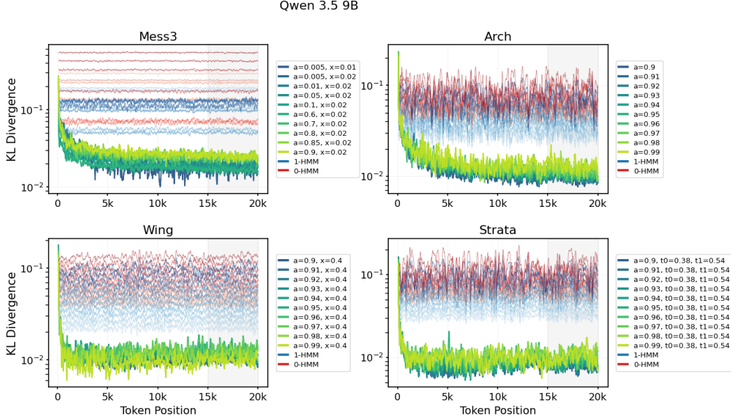
Figure 17: Qwen 3.5 9B : KL divergence between the LLM’s next-token probabilities (NTP) and full HMM’s ground-truth NTP, alongside that between the order-1’s and order-0’s ground-truth NTP and the full HMM’s, for all 40 HMMs.
