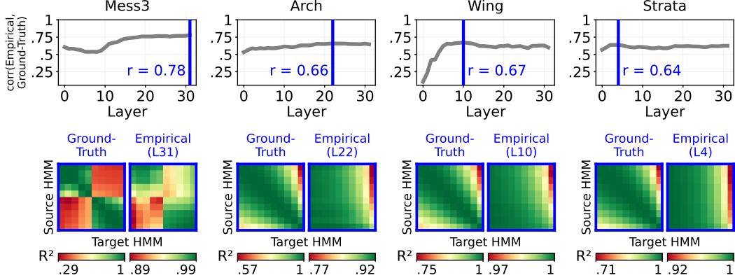
Figure 4: A probe trained on one parametrization decodes a similar parametrization’s beliefs well, but a dissimilar one’s poorly. This cross-parametrization decodability is shown in an “empirical matrix” where entry (i, j) = beliefs of parametrization j decoded from activations on parametrization i . Across layers, the empirical matrix correlates with the ground-truth cross-parametrization decodability. The best-matching layer’s empirical matrix is shown (blue line).
