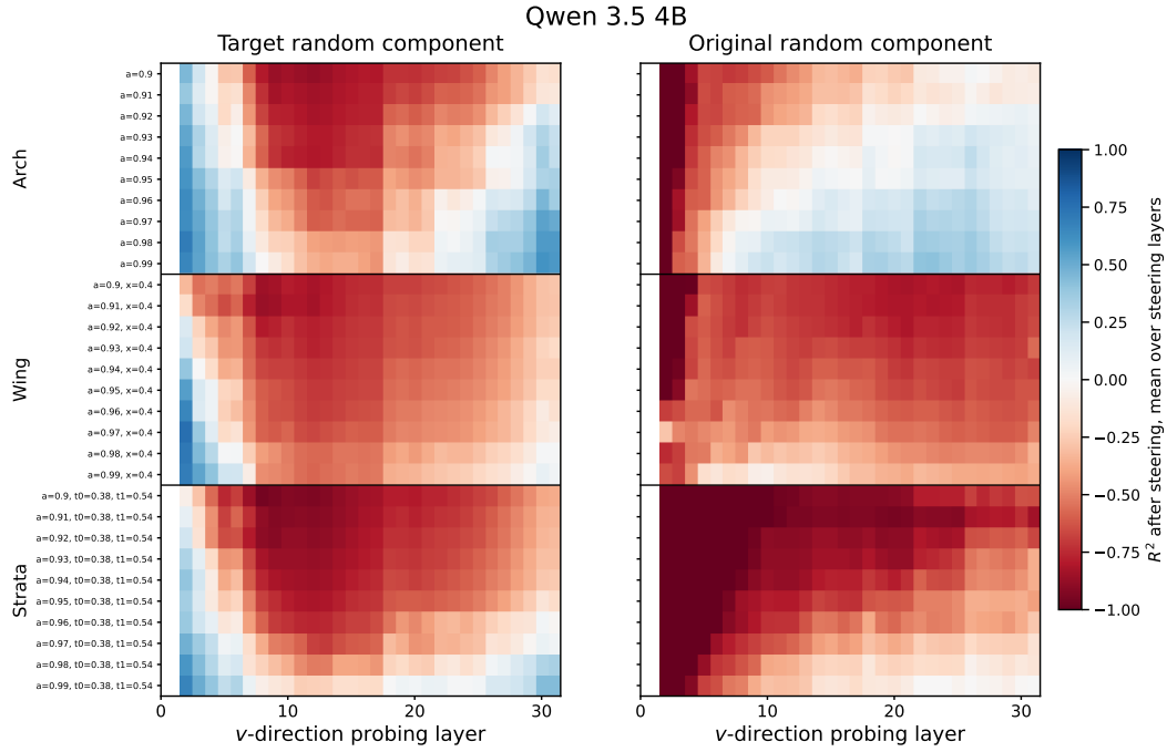
Figure 66: Qwen 3.5 4B : Post-steering v -component decodability across all HMM parametrizations. Each cell reports the R^2 of the projection of steered activations onto the random direction v , averaged over all steering layers at least two layers below the probing layer, scored against the pre-steering projection plus the injected magnitude ( left , the target component) and against the pre-steering projection ( right , the original component). Rows index HMM parametrizations grouped by family; columns index the v -direction probing layer. Blue indicates positive R^2 , red negative. The first two columns are undefined, as no steering layer lies at least two layers below. Mess3 is absent, as the steer magnitudes are matched to the \delta -belief steer, which requires a rank-deficient M . Values are means across 10 sequences.
