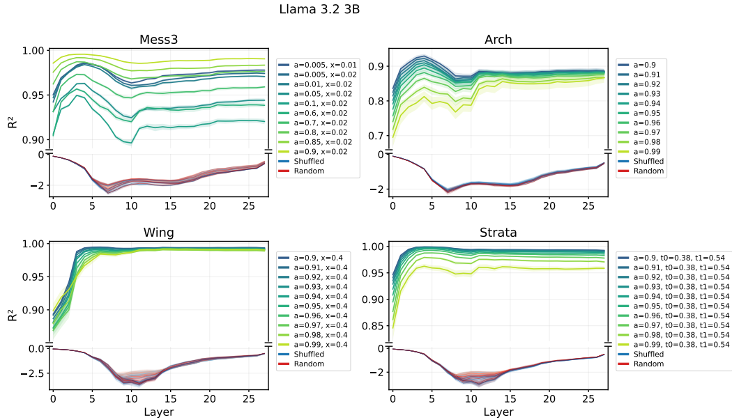
Figure 32: Llama 3.2 3B : All 40 HMM linear probe fits, including fits to each HMM's corresponding shuffled belief and random belief controls.
