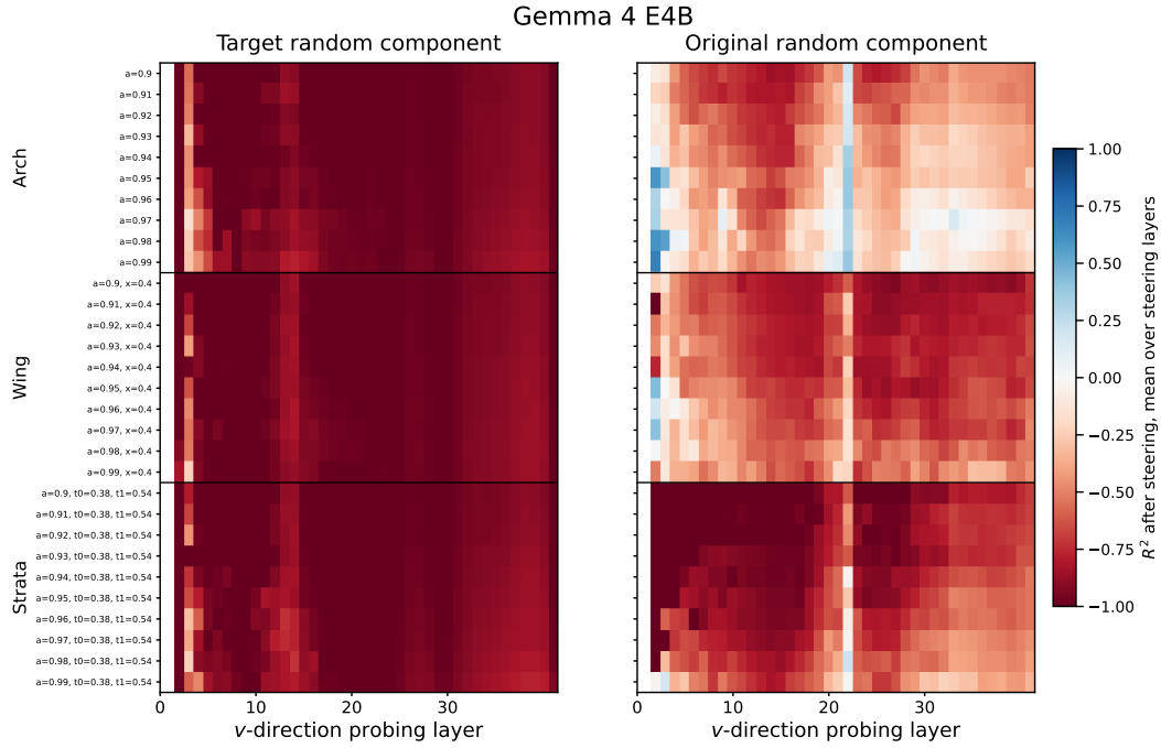
Figure 69: Gemma 4 E4B : Post-steering v -component decodability across all HMM parametrizations. Each cell reports the R^2 of the projection of steered activations onto the random direction v , averaged over all steering layers at least two layers below the probing layer, scored against the pre-steering projection plus the injected magnitude ( left , the target component) and against the pre-steering projection ( right , the original component). Rows index HMM parametrizations grouped by family; columns index the v -direction probing layer. Blue indicates positive R^2 , red negative. The first two columns are undefined, as no steering layer lies at least two layers below. Mess3 is absent, as the steer magnitudes are matched to the \delta -belief steer, which requires a rank-deficient M . Values are means across 10 sequences.
