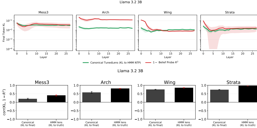
Figure 80: Llama 3.2 3B : Top : canonical lens KL to HMM ground truth (green) vs. 1 - R^2 (red), by layer. Mean over parametrizations; bands \pm 1 std. Bottom : per-sequence Pearson correlation between each lens’s KL-by-layer curve and 1 - R^2 of the belief probe (mean over 10 parametrizations \times 10 seeds; error bars 95% CI): the canonical lens scored on its training objective, KL to the model’s final-layer distribution ( left bar ), and the ground-truth-supervised lens of Section 8 scored on KL to the ground truth ( right bar ).
