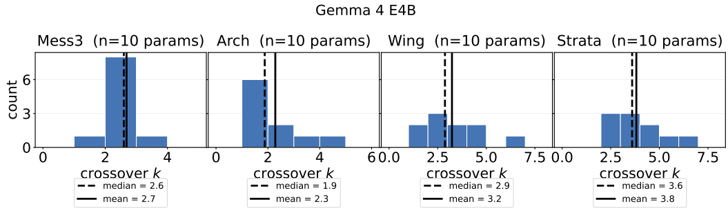
Figure 27: Gemma 4 E4B : Distribution of the crossover order k across the 10 parametrizations of each HMM family. The crossover k is the smallest Markov order whose k -HMM predictor matches the LLM’s converged KL—the first k at which the k -HMM’s KL to the full HMM falls to the LLM’s. Dashed and solid lines mark the median and mean.
