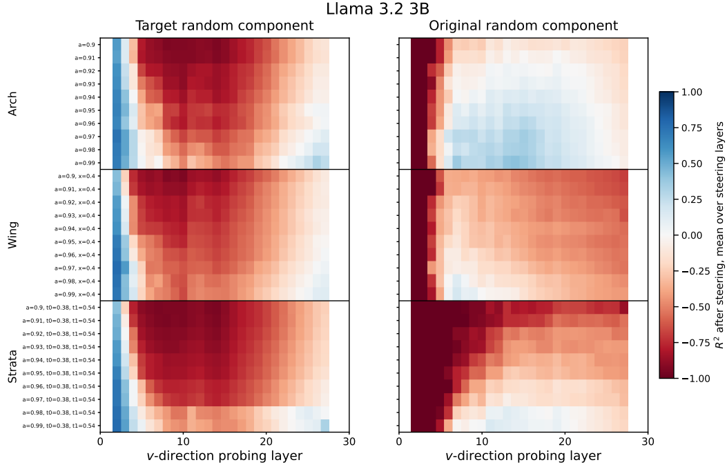
Figure 68: Llama 3.2 3B : Post-steering v -component decodability across all HMM parametrizations. Each cell reports the R^2 of the projection of steered activations onto the random direction v , averaged over all steering layers at least two layers below the probing layer, scored against the pre-steering projection plus the injected magnitude ( left , the target component) and against the pre-steering projection ( right , the original component). Rows index HMM parametrizations grouped by family; columns index the v -direction probing layer. Blue indicates positive R^2 , red negative. The first two columns are undefined, as no steering layer lies at least two layers below. Mess3 is absent, as the steer magnitudes are matched to the \delta -belief steer, which requires a rank-deficient M . Values are means across 10 sequences.
