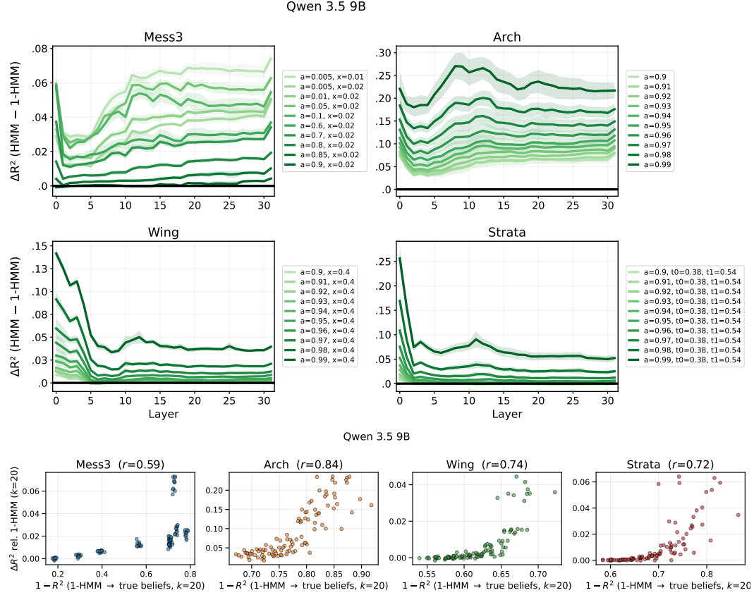
Figure 41: Qwen 3.5 9B : Top : R^2 differences at suffix length k = 20 between probes fit to the beliefs of the real HMM and those of the order-1 HMM at k -suffix length 20 across all layers for all 40 HMMs. Bottom : each sequence’s \Delta R^2 at the best layer against its theoretical counterpart, 1 - R^2 of linearly predicting the true belief state at k = 20 from the 1-HMM belief state on the same sequence. Each point is one sequence (10 parametrizations \times 10 seeds per family); panel titles report the Pearson correlation.
