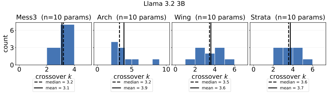
Figure 26: Llama 3.2 3B : Distribution of the crossover order k across the 10 parametrizations of each HMM family. The crossover k is the smallest Markov order whose k -HMM predictor matches the LLM’s converged KL—the first k at which the k -HMM’s KL to the full HMM falls to the LLM’s. Dashed and solid lines mark the median and mean.
