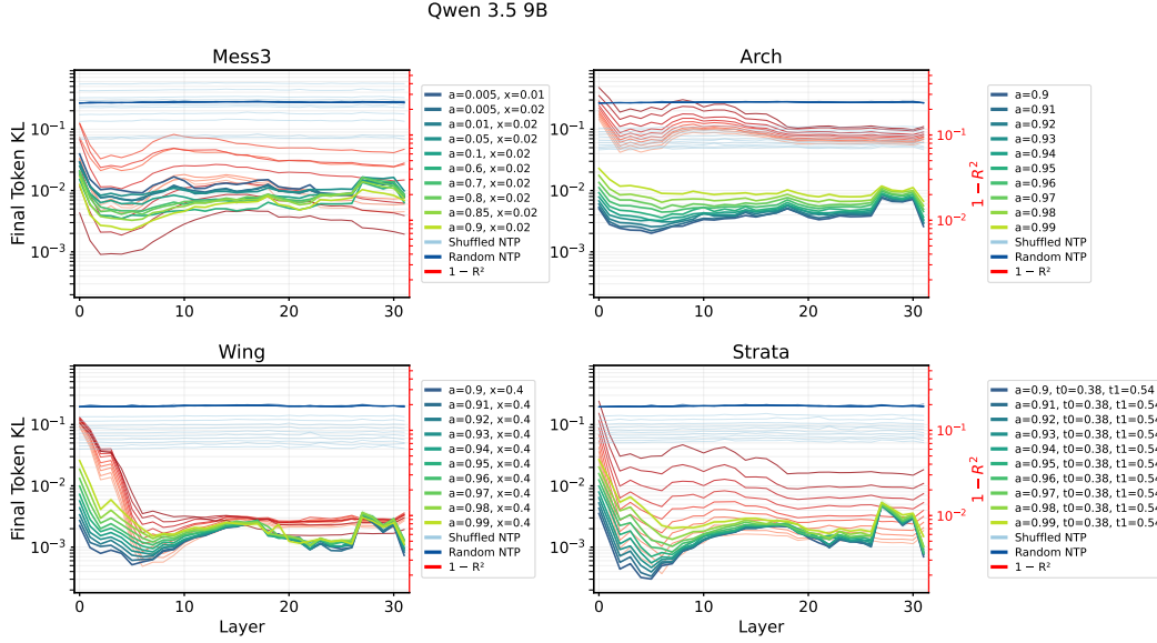
Figure 83: Qwen 3.5 9B : For every parametrization of each family, the per-layer KL of the tuned lens to the HMM ground-truth NTP (colored by parametrization, left axis) shown against the belief probe’s 1 - R^2 (red, right axis). Lenses trained to shuffled- and random-NTP controls (light/dark blue) stay high across all layers.
