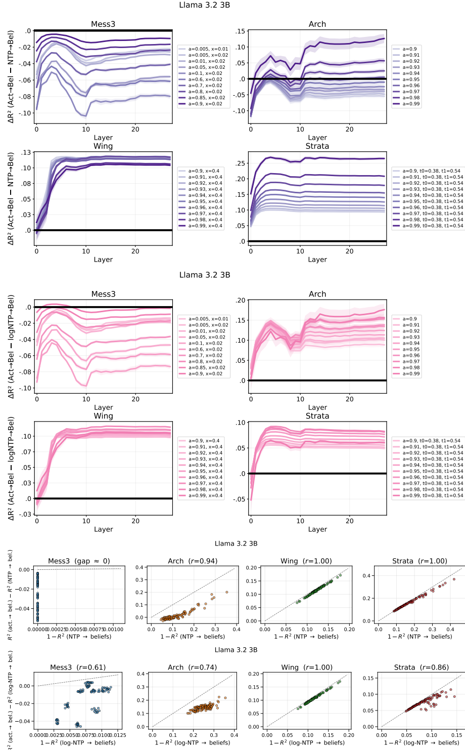
Figure 50: Llama 3.2 3B : Rows 1–2: R^2 differences between probes fit to belief states from activations and from NTP or log-NTP across all layers for all 40 HMMs. Rows 3–4: each sequence’s \Delta R^2 at the best layer against its theoretical counterpart, 1 - R^2 of linearly predicting the belief state from the ground-truth NTP (row 3) or log-NTP (row 4) on the same sequence. Each point is one sequence (10 parametrizations \times 10 seeds per family); panel titles report the Pearson correlation, and the dashed line marks the maximum possible \Delta R^2 . For Mess3 the map from beliefs to NTP is invertible, so the theoretical counterpart is zero and no correlation is defined.
