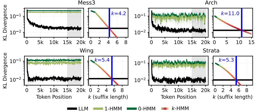
Figure 2: KL divergence between the next-token probabilities (NTP) of the ground-truth HMM and those of Qwen 3.5-9B and of k -HMM predictors. In each pair of plots, the left plot shows the KL values over token position, with the gray band marking the last 5,000 tokens over which the converged KL is computed. The right plot shows the crossover between the converged KL of Qwen 3.5-9B and that of a k -HMM as a function of k . Error bands are 95% confidence intervals over 10 sequences.
