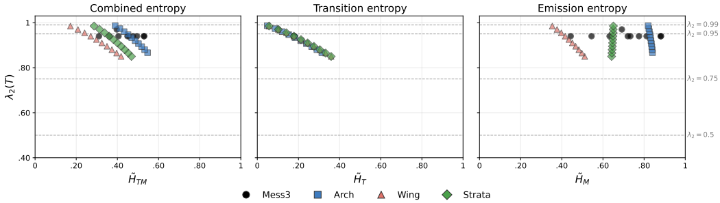
Figure 10: The 40-process sweep covers a region of the entropy–mixing plane and samples from the slow-mixing, low entropy area. Markers show 40 HMM parametrizations (10 per family); colors and shapes encode the family. The y-axis is the mixing rate \lambda_2(T) ; horizontal dashed lines mark the discrete grid \lambda_2 \in \{0.5, 0.75, 0.95, 0.99\} used by Dai et al. (2025). Panels show, left to right, the combined normalized entropy \tilde{H}_{TM} (their Figure 4 left-panel axis), the transition entropy \tilde{H}_T , and the emission entropy \tilde{H}_M . Wing, Strata, and Arch sweep \lambda_2 at three entropy bands; Mess3 sweeps entropy at near-fixed \lambda_2 \approx 0.94 as an entropy-only control.
