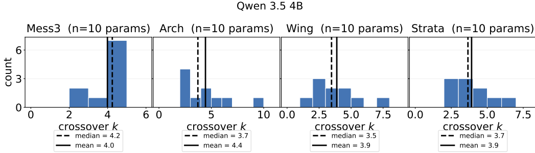
Figure 24: Qwen 3.5 4B : Distribution of the crossover order k across the 10 parametrizations of each HMM family. The crossover k is the smallest Markov order whose k -HMM predictor matches the LLM’s converged KL—the first k at which the k -HMM’s KL to the full HMM falls to the LLM’s. Dashed and solid lines mark the median and mean.
