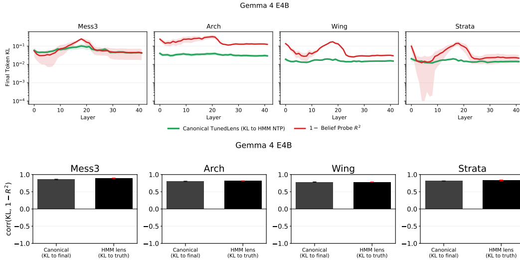
Figure 81: Gemma 4 E4B : Top : canonical lens KL to HMM ground truth (green) vs. 1 - R^2 (red), by layer. Mean over parametrizations; bands \pm 1 std. Bottom : per-sequence Pearson correlation between each lens’s KL-by-layer curve and 1 - R^2 of the belief probe (mean over 10 parametrizations \times 10 seeds; error bars 95% CI): the canonical lens scored on its training objective, KL to the model’s final-layer distribution ( left bar ), and the ground-truth-supervised lens of Section 8 scored on KL to the ground truth ( right bar ).
