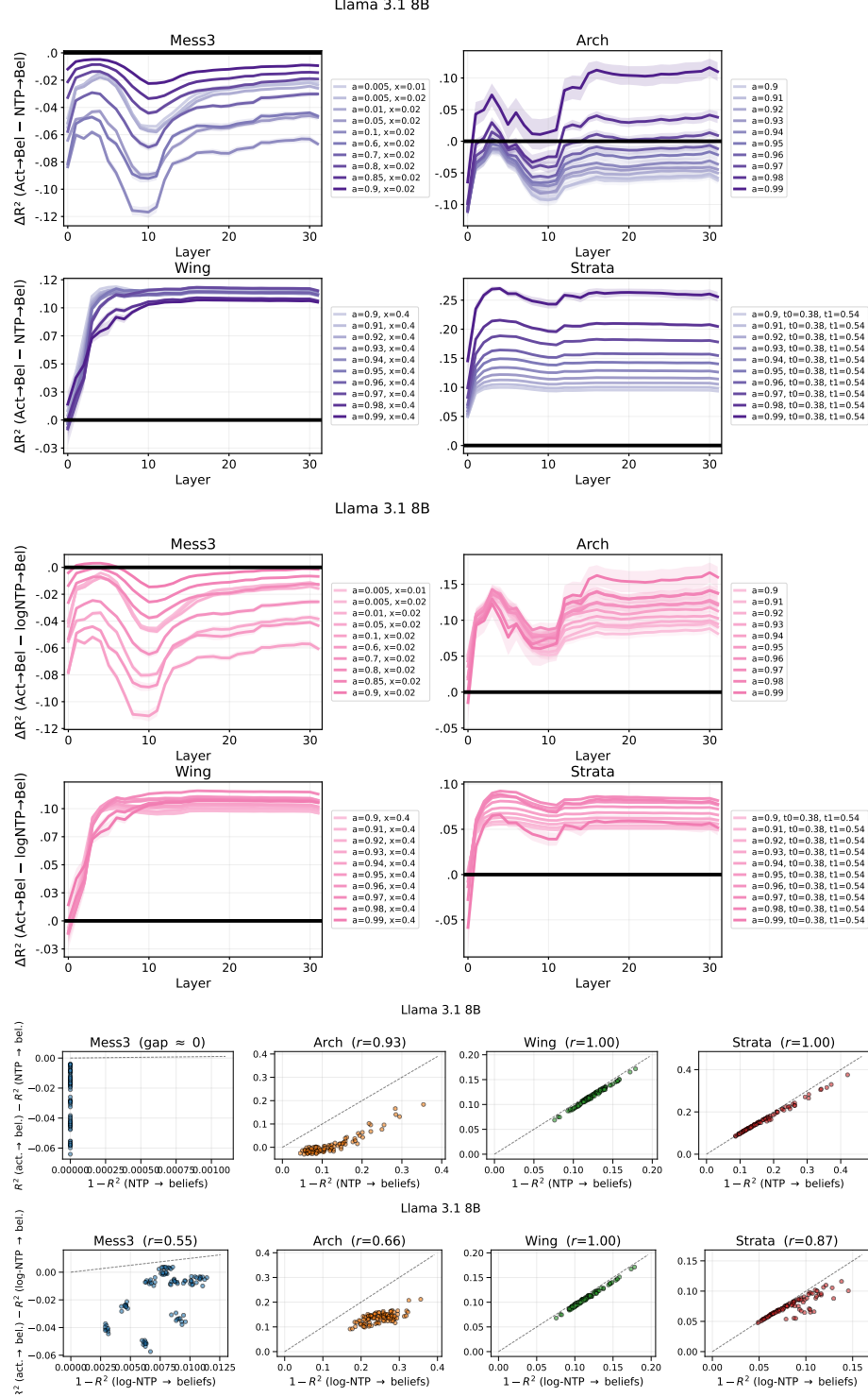
Figure 49: Llama 3.1 8B : Rows 1–2: R^2 differences between probes fit to belief states from activations and from NTP or log-NTP across all layers for all 40 HMMs. Rows 3–4: each sequence’s \Delta R^2 at the best layer against its theoretical counterpart, 1 - R^2 of linearly predicting the belief state from the ground-truth NTP (row 3) or log-NTP (row 4) on the same sequence. Each point is one sequence (10 parametrizations \times 10 seeds per family); panel titles report the Pearson correlation, and the dashed line marks the maximum possible \Delta R^2 . For Mess3 the map from beliefs to NTP is invertible, so the theoretical counterpart is zero and no correlation is defined.
