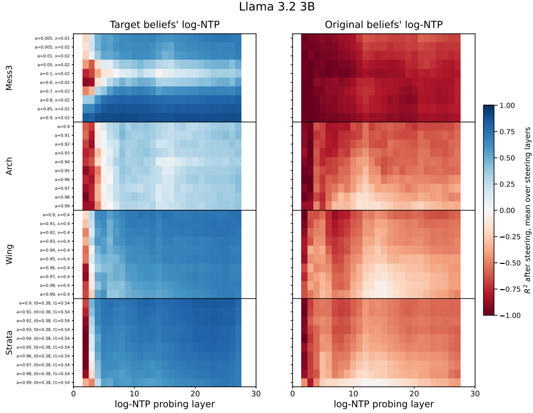
Figure 56: Llama 3.2 3B : Post-steering decodability across all HMM parametrizations. Each cell reports the R^2 of a probe applied to steered activations, averaged over all steering layers at least two layers below the probing layer. The probe is fit on unsteered activations to decode the original beliefs' implied log-NTP and is applied unchanged after steering, and its predictions are scored against the target beliefs' implied log-NTP ( left ) and the original beliefs' implied log-NTP ( right ). Rows index HMM parametrizations grouped by family; columns index the probing layer. Blue indicates positive R^2 , red negative. The first two columns are undefined, as no steering layer lies at least two layers below. Values are means across 10 sequences.
