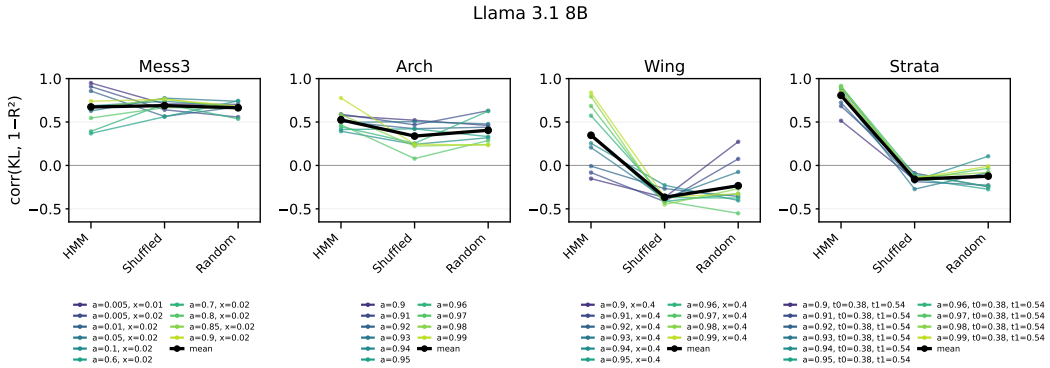
Figure 91: Llama 3.1 8B : Correlation between KL and 1 - R^2 for all conditions and every HMM.
