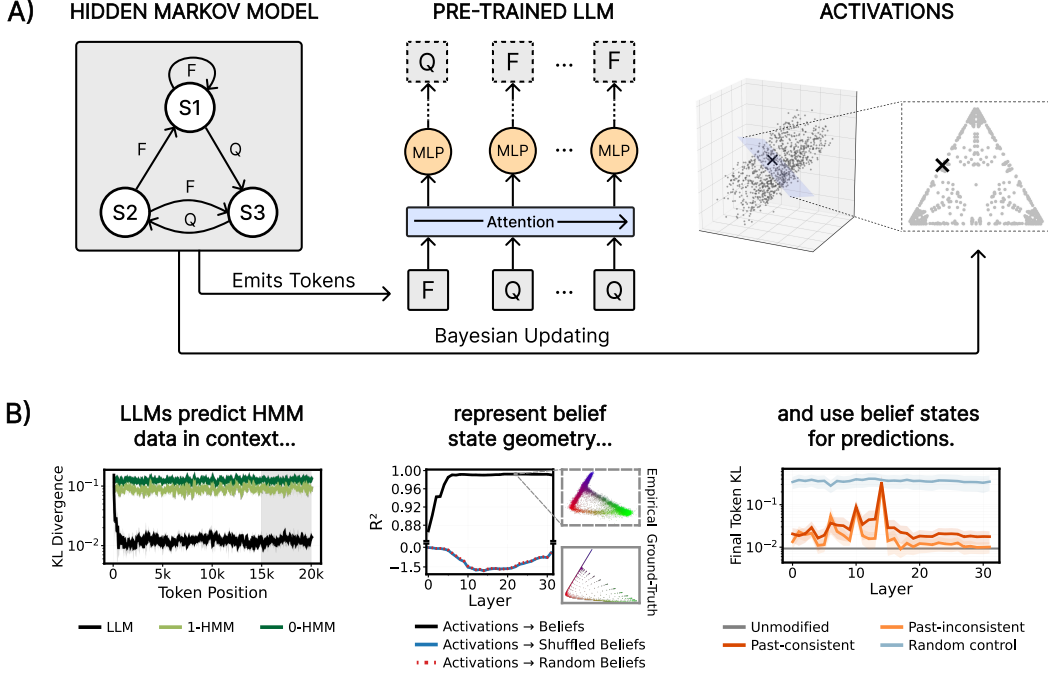
Figure 1: HMMs induce belief state geometry in LLMs. (a) An HMM (left) emits tokens by transitioning between hidden states (S1, S2, S3). Conditioning on this sequence in-context, an LLM (middle) predicts the next token. Computational mechanics suggests that optimal prediction requires tracking the belief state—the posterior over the HMM’s hidden states—whose reachable set traces a characteristic geometry in the activation space (right). (b) Results preview for one HMM (Wing). The LLM predicts near-optimally in-context (left), linear probes recover the belief geometry far beyond controls (middle), and intervening on the belief subspace influences the predictions (right).
