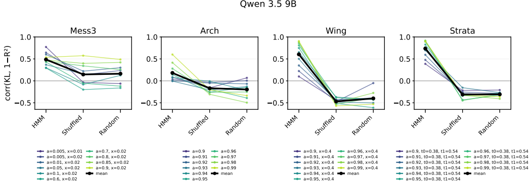
Figure 89: Qwen 3.5 9B : Correlation between KL and 1 - R^2 for all conditions and every HMM.
