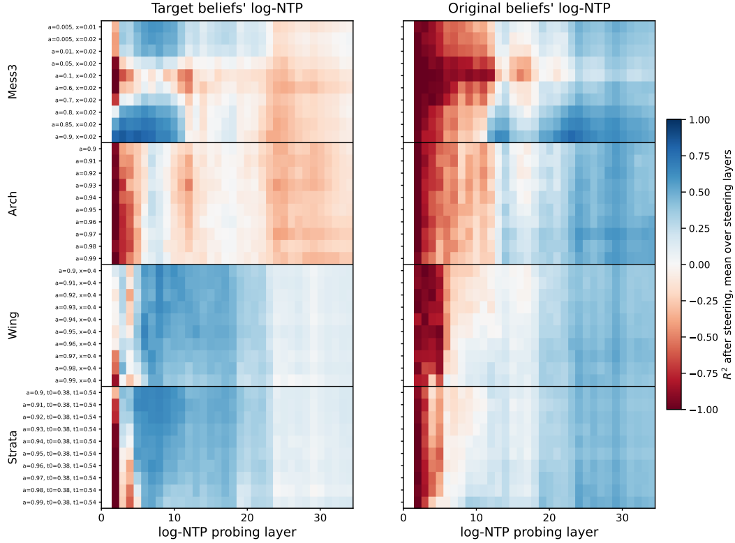
Figure 58: Gemma 4 E2B : Post-steering decodability across all HMM parametrizations. Each cell reports the R^2 of a probe applied to steered activations, averaged over all steering layers at least two layers below the probing layer. The probe is fit on unsteered activations to decode the original beliefs' implied log-NTP and is applied unchanged after steering, and its predictions are scored against the target beliefs' implied log-NTP ( left ) and the original beliefs' implied log-NTP ( right ). Rows index HMM parametrizations grouped by family; columns index the probing layer. Blue indicates positive R^2 , red negative. The first two columns are undefined, as no steering layer lies at least two layers below. Values are means across 10 sequences.
