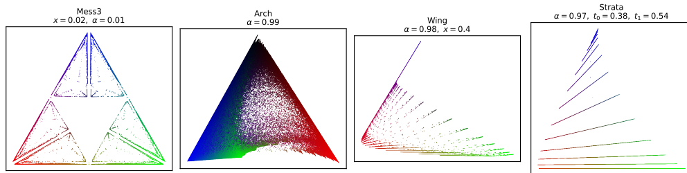
Figure 9: Belief-state geometry for the four HMM families. Each point is a belief state drawn from 50 independently sampled sequences of 10,000 tokens; colors encode the first three belief coordinates as RGB. Three-state processes (Mess3, Wing, Strata) are projected onto the 2-simplex via an equilateral-triangle embedding; the four-state Arch process is shown in its leading two PCA components.
