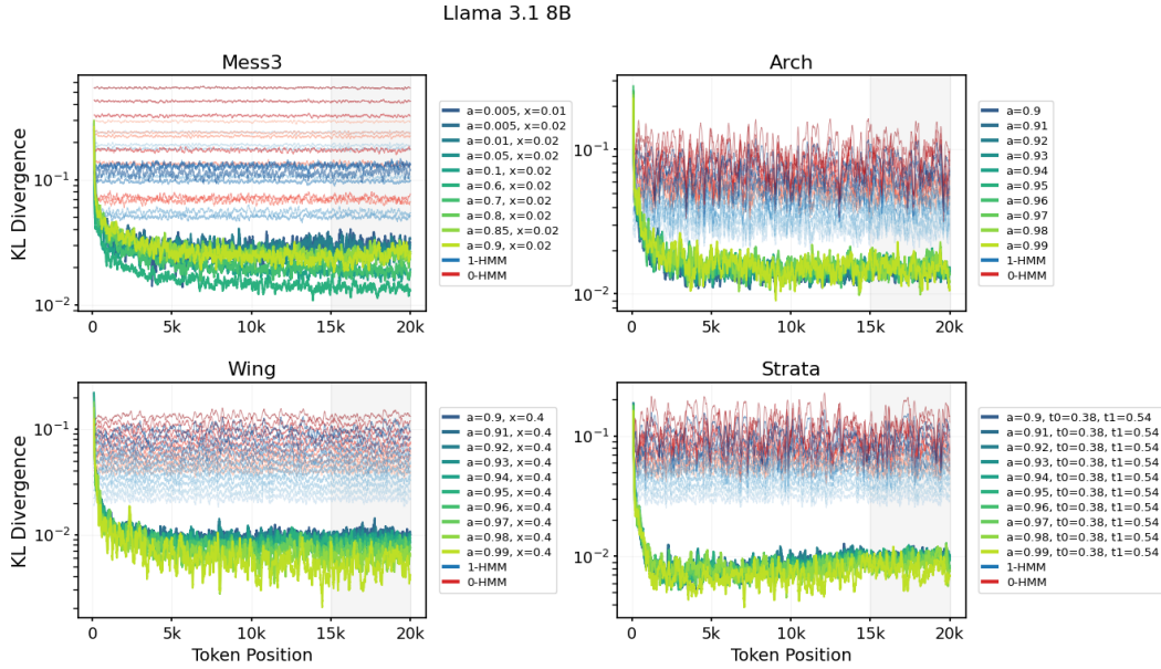
Figure 19: Llama 3.1 8B : KL divergence between the LLM's next-token probabilities (NTP) and full HMM's ground-truth NTP, alongside that between the order-1's and order-0's ground-truth NTP and the full HMM's, for all 40 HMMs.
