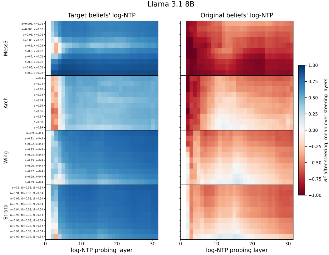
Figure 55: Llama 3.1 8B : Post-steering decodability across all HMM parametrizations. Each cell reports the R^2 of a probe applied to steered activations, averaged over all steering layers at least two layers below the probing layer. The probe is fit on unsteered activations to decode the original beliefs' implied log-NTP and is applied unchanged after steering, and its predictions are scored against the target beliefs' implied log-NTP ( left ) and the original beliefs' implied log-NTP ( right ). Rows index HMM parametrizations grouped by family; columns index the probing layer. Blue indicates positive R^2 , red negative. The first two columns are undefined, as no steering layer lies at least two layers below. Values are means across 10 sequences.
