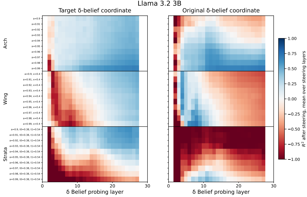
Figure 62: Llama 3.2 3B : Post-steering \delta -coordinate decodability across all HMM parametrizations. Each cell reports the R^2 of a probe applied to steered activations, averaged over all steering layers at least two layers below the probing layer. The probe is fit on unsteered activations to decode the original beliefs' \delta -coordinate and is applied unchanged after steering, and its predictions are scored against the target beliefs' \delta -coordinate ( left ) and the original beliefs' \delta -coordinate ( right ). Rows index HMM parametrizations grouped by family; columns index the probing layer. Blue indicates positive R^2 , red negative. The first two columns are undefined, as no steering layer lies at least two layers below. Mess3 is absent, as its full-rank M admits no NTP-preserving direction. Values are means across 10 sequences.
