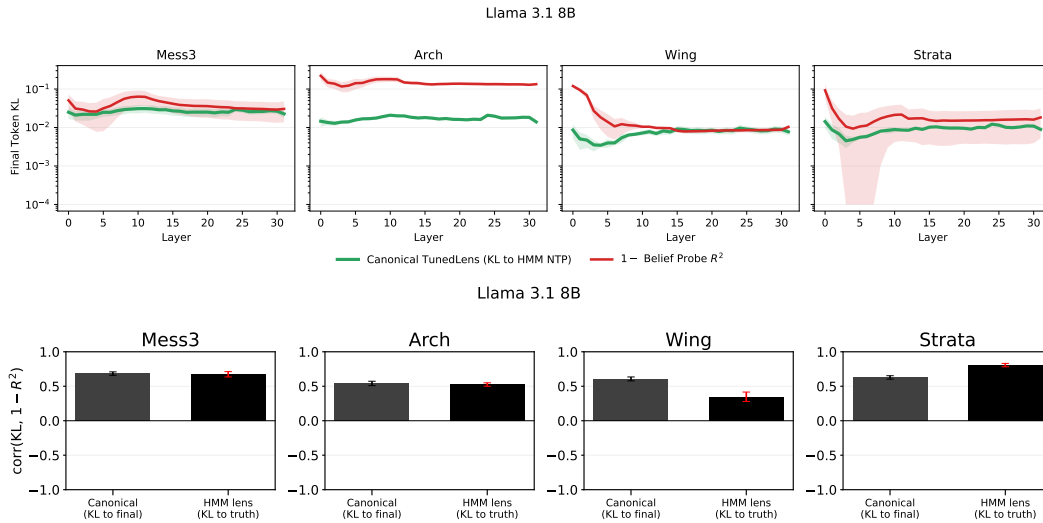
Figure 79: Llama 3.1 8B : Top : canonical lens KL to HMM ground truth (green) vs. 1 - R^2 (red), by layer. Mean over parametrizations; bands \pm 1 std. Bottom : per-sequence Pearson correlation between each lens’s KL-by-layer curve and 1 - R^2 of the belief probe (mean over 10 parametrizations \times 10 seeds; error bars 95% CI): the canonical lens scored on its training objective, KL to the model’s final-layer distribution ( left bar ), and the ground-truth-supervised lens of Section 8 scored on KL to the ground truth ( right bar ).
