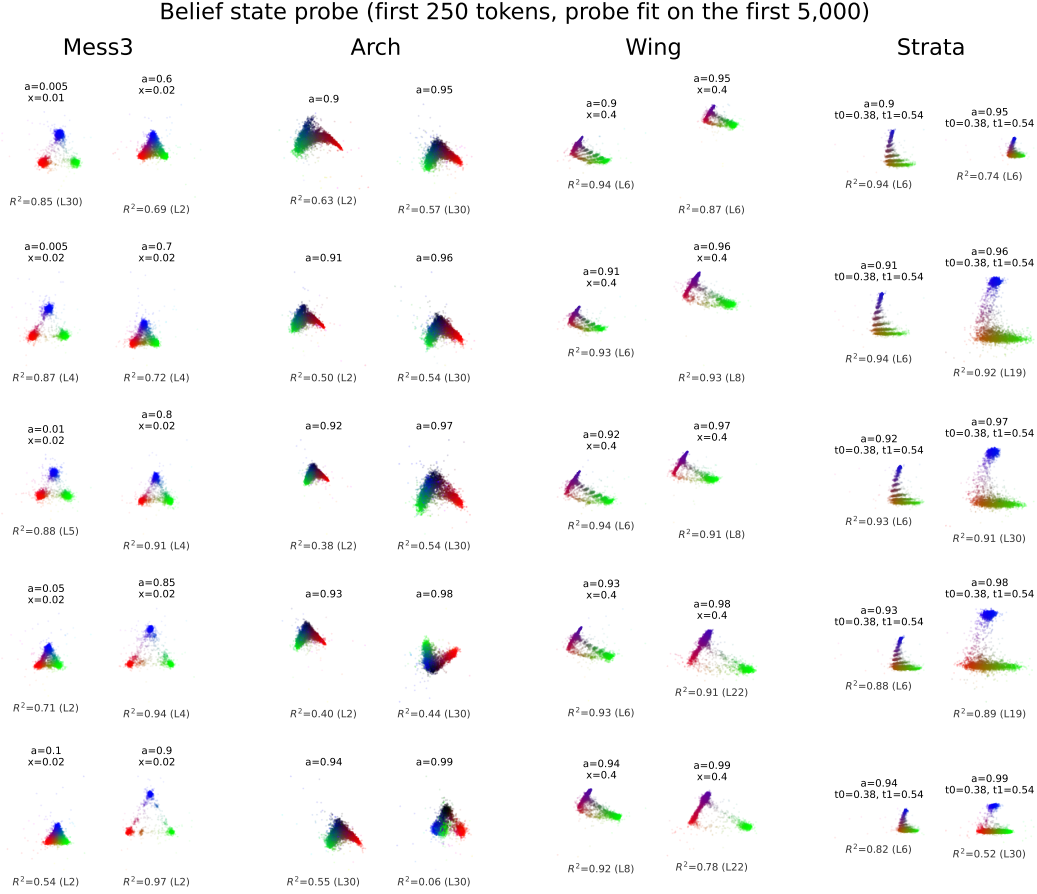
Figure 15: Geometries discovered by linear probes trained on 1,000 random positions among the first 5,000 token positions of each sequence and evaluated on their held-out positions among the first 250 tokens, with their fit (held-out R^2 on those positions, averaged over 10 sequences) at each HMM's best-fitting layer in Qwen 3.5 9B, for all 10 sequences as in Figure 11. The probes are the same size as those of Figure 11; only the positions on which they are evaluated differ. We evaluate on the first 250 tokens only, because the model's in-context prediction accuracy almost fully converges after the first few hundred tokens (Figure 2). The belief state geometry is visibly weaker in the first 250 tokens.
