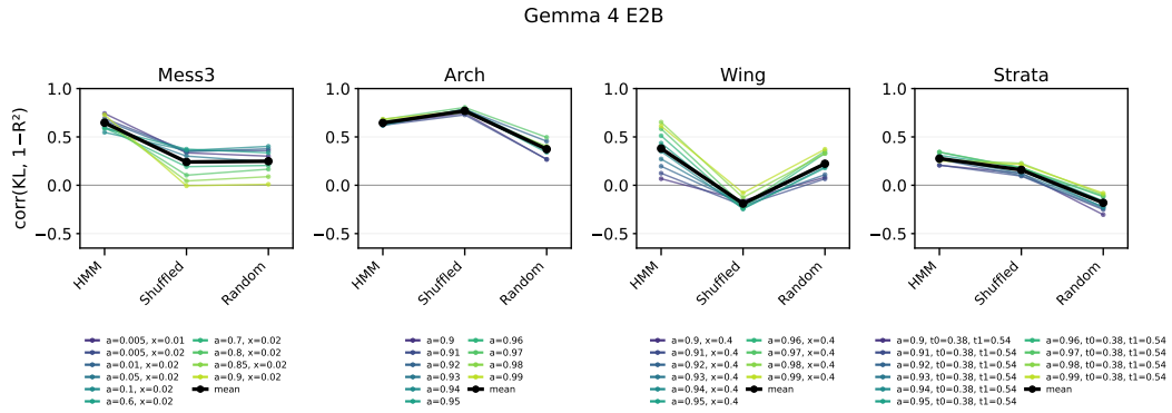
Figure 94: Gemma 4 E2B : Correlation between KL and 1 - R^2 for all conditions and every HMM.
