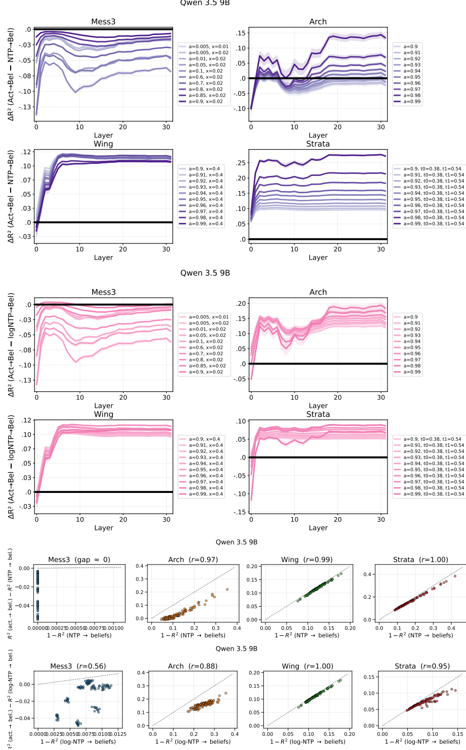
Figure 47: Qwen 3.5 9B : Rows 1–2: R^2 differences between probes fit to belief states from activations and from NTP or log-NTP across all layers for all 40 HMMs. Rows 3–4: each sequence’s \Delta R^2 at the best layer against its theoretical counterpart, 1 - R^2 of linearly predicting the belief state from the ground-truth NTP (row 3) or log-NTP (row 4) on the same sequence. Each point is one sequence (10 parametrizations \times 10 seeds per family); panel titles report the Pearson correlation, and the dashed line marks the maximum possible \Delta R^2 . For Mess3 the map from beliefs to NTP is invertible, so the theoretical counterpart is zero and no correlation is defined.
