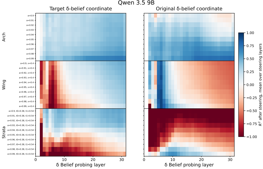
Figure 59: Qwen 3.5 9B : Post-steering \delta -coordinate decodability across all HMM parametrizations. Each cell reports the R^2 of a probe applied to steered activations, averaged over all steering layers at least two layers below the probing layer. The probe is fit on unsteered activations to decode the original beliefs' \delta -coordinate and is applied unchanged after steering, and its predictions are scored against the target beliefs' \delta -coordinate ( left ) and the original beliefs' \delta -coordinate ( right ). Rows index HMM parametrizations grouped by family; columns index the probing layer. Blue indicates positive R^2 , red negative. The first two columns are undefined, as no steering layer lies at least two layers below. Mess3 is absent, as its full-rank M admits no NTP-preserving direction. Values are means across 10 sequences.
