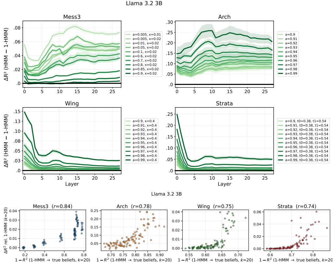
Figure 44: Llama 3.2 3B: Top: R^2 differences at suffix length k = 20 between probes fit to the beliefs of the real HMM and those of the order-1 HMM at k -suffix length 20 across all layers for all 40 HMMs. Bottom: each sequence's \Delta R^2 at the best layer against its theoretical counterpart, 1 - R^2 of linearly predicting the true belief state at k = 20 from the 1-HMM belief state on the same sequence. Each point is one sequence (10 parametrizations \times 10 seeds per family); panel titles report the Pearson correlation.
