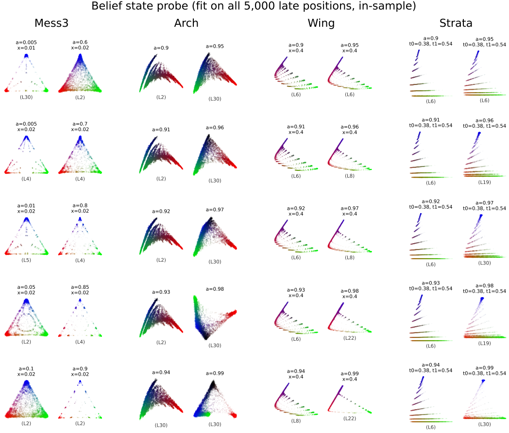
Figure 12: Geometries recovered by linear probes fit on all 5,000 late token positions of each sequence and shown on those same positions, for each of the 10 sequences, at each HMM’s best-fitting layer in Qwen 3.5 9B. These in-sample fits are shown for comparison with the previous figure (Figure 11).
