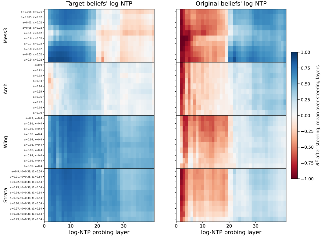
Figure 57: Gemma 4 E4B: Post-steering decodability across all HMM parametrizations. Each cell reports the R^2 of a probe applied to steered activations, averaged over all steering layers at least two layers below the probing layer. The probe is fit on unsteered activations to decode the original beliefs' implied log-NTP and is applied unchanged after steering, and its predictions are scored against the target beliefs' implied log-NTP ( left ) and the original beliefs' implied log-NTP ( right ). Rows index HMM parametrizations grouped by family; columns index the probing layer. Blue indicates positive R^2 , red negative. The first two columns are undefined, as no steering layer lies at least two layers below. Values are means across 10 sequences.
