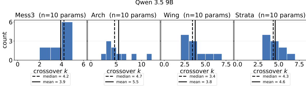
Figure 23: Qwen 3.5 9B : Distribution of the crossover order k across the 10 parametrizations of each HMM family. The crossover k is the smallest Markov order whose k -HMM predictor matches the LLM’s converged KL—the first k at which the k -HMM’s KL to the full HMM falls to the LLM’s. Dashed and solid lines mark the median and mean.
