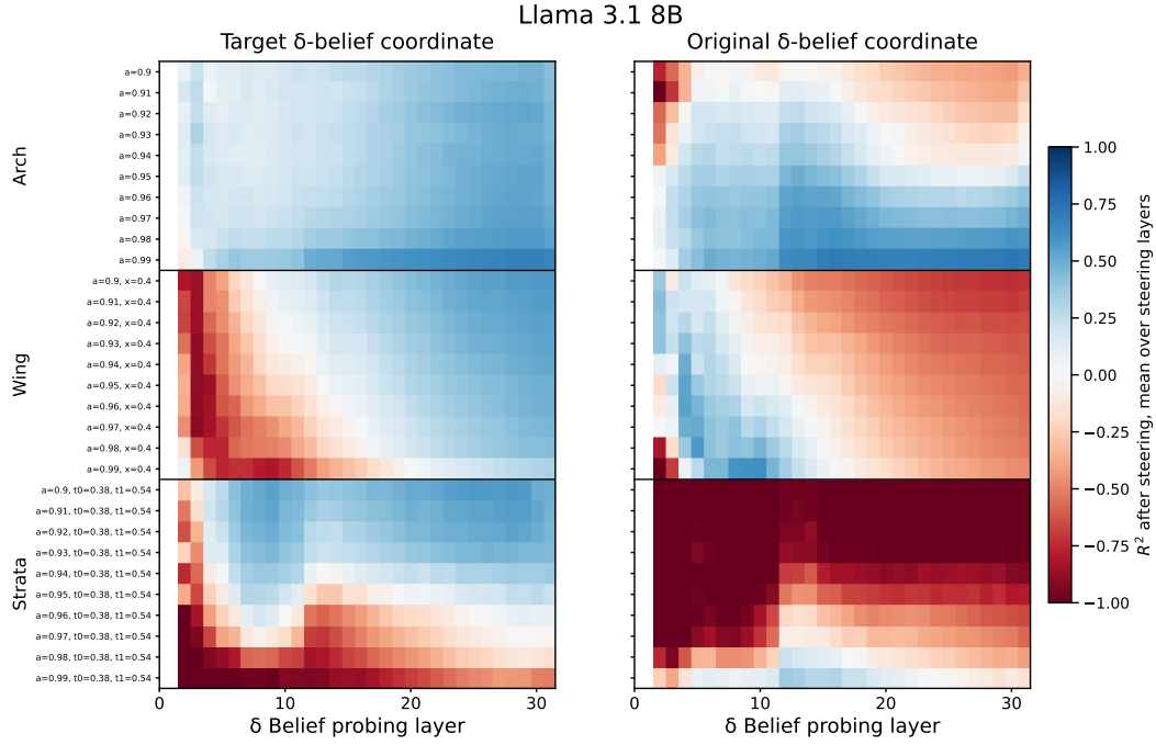
Figure 61: Llama 3.1 8B : Post-steering \delta -coordinate decodability across all HMM parametrizations. Each cell reports the R^2 of a probe applied to steered activations, averaged over all steering layers at least two layers below the probing layer. The probe is fit on unsteered activations to decode the original beliefs' \delta -coordinate and is applied unchanged after steering, and its predictions are scored against the target beliefs' \delta -coordinate ( left ) and the original beliefs' \delta -coordinate ( right ). Rows index HMM parametrizations grouped by family; columns index the probing layer. Blue indicates positive R^2 , red negative. The first two columns are undefined, as no steering layer lies at least two layers below. Mess3 is absent, as its full-rank M admits no NTP-preserving direction. Values are means across 10 sequences.
