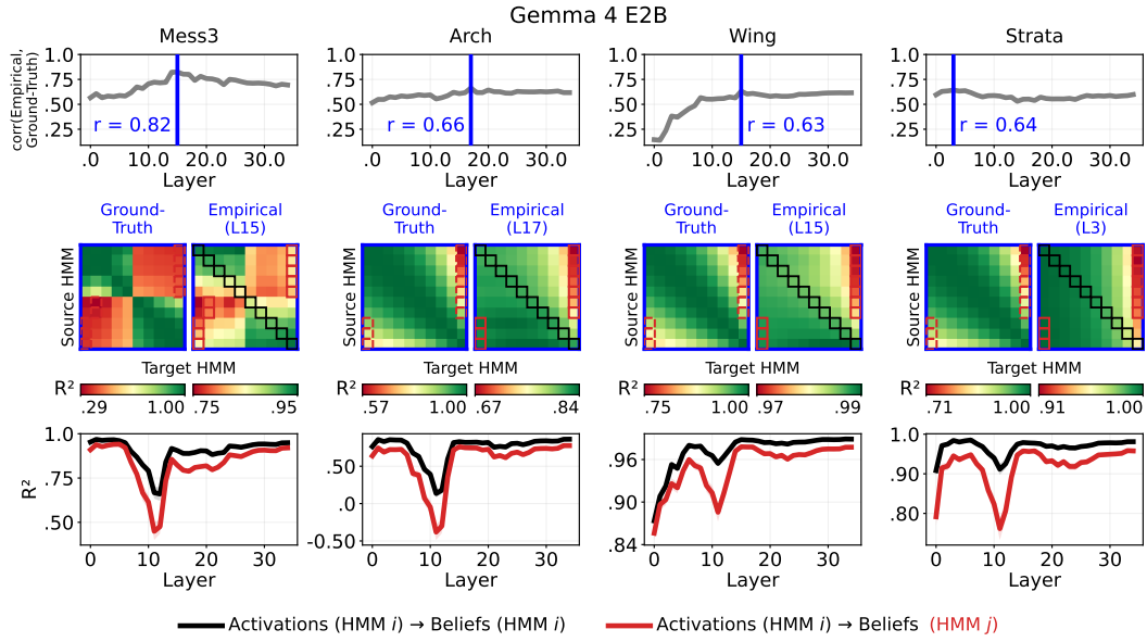
Figure 40: Gemma 4 E2B : Probes fit to beliefs of HMMs that were not the HMM that generated the token sequence. HMM j (bordered red in the heatmaps) is the parametrization whose ground-truth transfer R^2 is lowest from activations on HMM i 's sequence. The last row of plots shows that predicting HMM j 's beliefs from activations on HMM i 's sequence is poorer than predicting HMM i 's beliefs.
