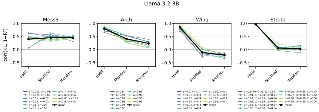
Figure 92: Llama 3.2 3B : Correlation between KL and 1 - R^2 for all conditions and every HMM.
