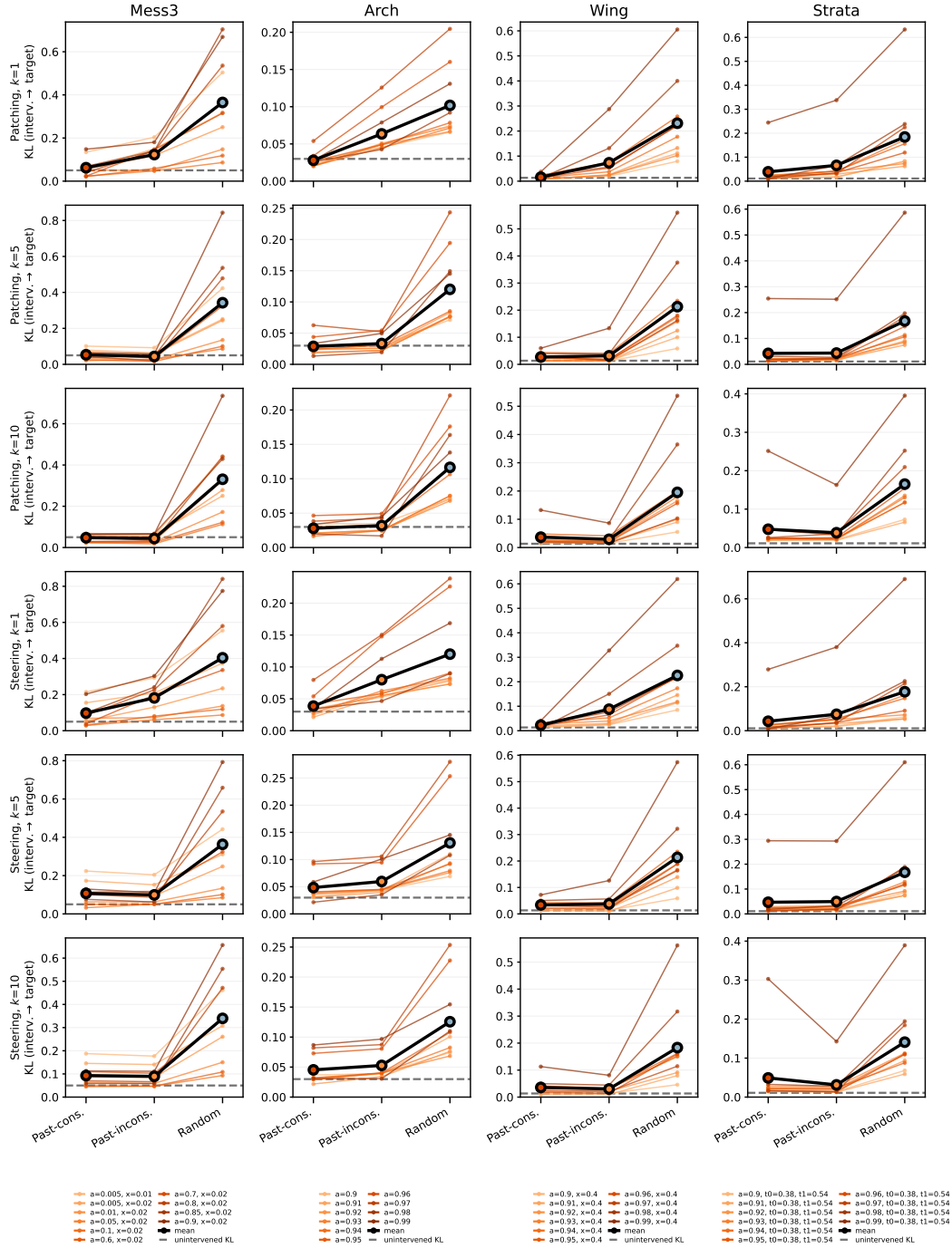
Figure 71: Qwen 3.5 9B : KL between the intervened prediction and the injected target belief’s NTP, averaged over the final 70% of layers, for each parametrization (orange lines; black = mean). Rows are intervention type and k -suffix length (patching then steering, k \in \{1, 5, 10\} ); columns are HMM families. Lower means the prediction moved closer to the injected belief. The dashed gray line marks the model’s unintervened KL to the ground-truth NTP, a reference for how closely the model tracks a target it follows; for the random condition, the target is the stationary belief’s NTP.
