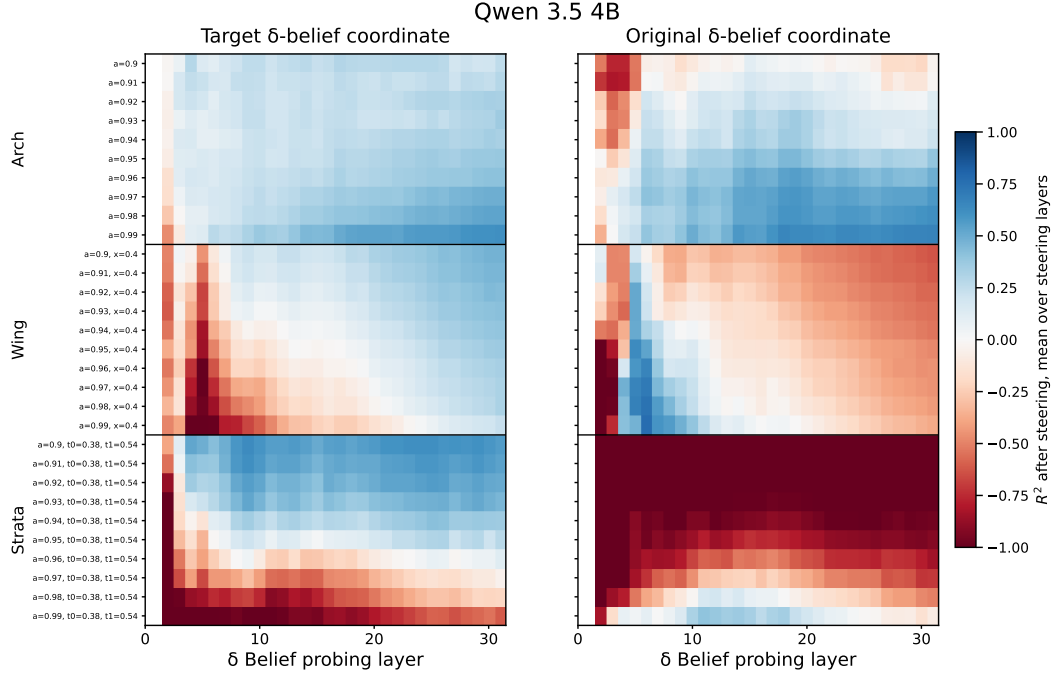
Figure 60: Qwen 3.5 4B : Post-steering \delta -coordinate decodability across all HMM parametrizations. Each cell reports the R^2 of a probe applied to steered activations, averaged over all steering layers at least two layers below the probing layer. The probe is fit on unsteered activations to decode the original beliefs’ \delta -coordinate and is applied unchanged after steering, and its predictions are scored against the target beliefs’ \delta -coordinate ( left ) and the original beliefs’ \delta -coordinate ( right ). Rows index HMM parametrizations grouped by family; columns index the probing layer. Blue indicates positive R^2 , red negative. The first two columns are undefined, as no steering layer lies at least two layers below. Mess3 is absent, as its full-rank M admits no NTP-preserving direction. Values are means across 10 sequences.
