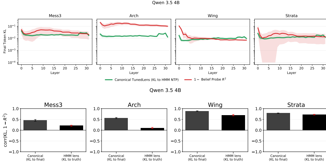
Figure 78: Qwen 3.5 4B : Top : canonical lens KL to HMM ground truth (green) vs. 1 - R^2 (red), by layer. Mean over parametrizations; bands \pm 1 std. Bottom : per-sequence Pearson correlation between each lens’s KL-by-layer curve and 1 - R^2 of the belief probe (mean over 10 parametrizations \times 10 seeds; error bars 95% CI): the canonical lens scored on its training objective, KL to the model’s final-layer distribution ( left bar ), and the ground-truth-supervised lens of Section 8 scored on KL to the ground truth ( right bar ).
