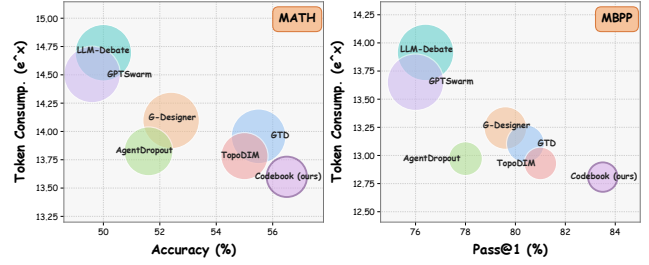
Figure 4: Accuracy–token trade-off on MATH and MBPP. Each bubble is one method: x is accuracy, y is \ln(\text{tokens} \times n) so that Token Consump. = e^y , and area scales with mean tokens per query. Lower-right is better; Codebook Agent sits nearest that corner on both benchmarks.
