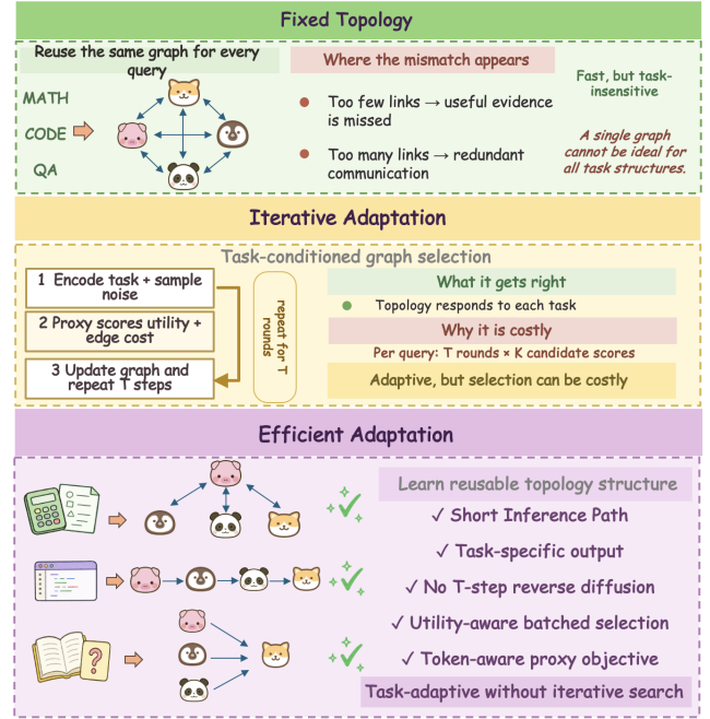
Figure 1: Three regimes of topology design. (Top) A fixed topology is reused for every query: zero design cost, but no single graph fits every task. (Middle) Query-conditioned generators adapt the graph via an iterative loop that samples and scores K candidates at each of T steps, typically with a proxy trained on utility and edge count. (Bottom) Codebook Agent keeps per-query adaptation and removes the loop: the design space is discretized once offline into a codebook, a query embedding selects codes, and one batched proxy call under a token-based cost objective returns the winner.
