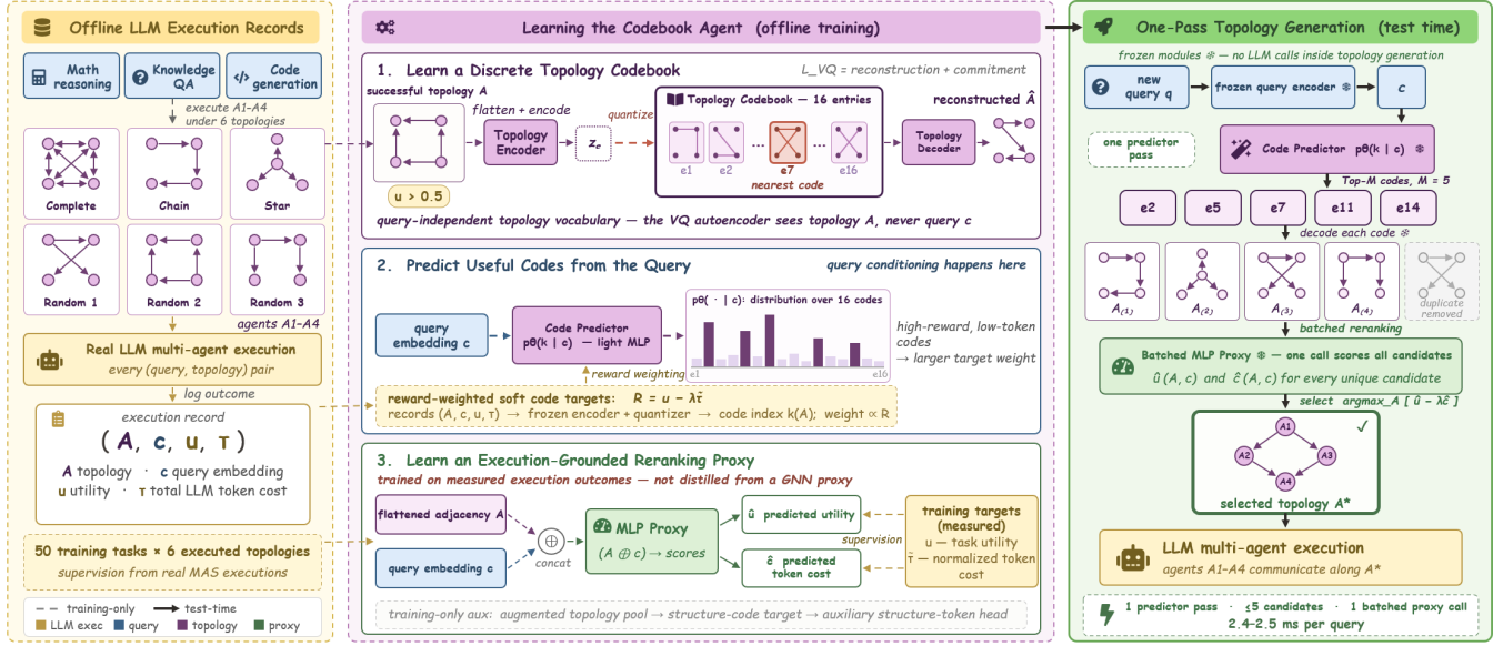
Figure 2: Overview of Codebook Agent. Left: offline collection executes fixed topologies on the training split and logs (A, c, u, \tau) for every (query, topology) pair. Middle: (1) a VQ autoencoder compresses successful topologies ( u > 0.5 ) into a query-independent codebook; (2) an MLP predictor p_\theta(k | c) is fit to the reward-weighted soft targets of Eq. (6); (3) an MLP proxy f_\phi is regressed on measured utility and per-task normalized token cost (Eqs. (8)–(10)), with an auxiliary structure-token head used in training only. Right: at test time the top M codes are decoded, deduplicated, and scored in one batched proxy call; the candidate maximizing \hat{u} - \lambda \hat{c} (Eq. (11)) is executed. Dashed arrows are training-only; solid arrows are the frozen test-time path (no LLM calls inside topology generation).
