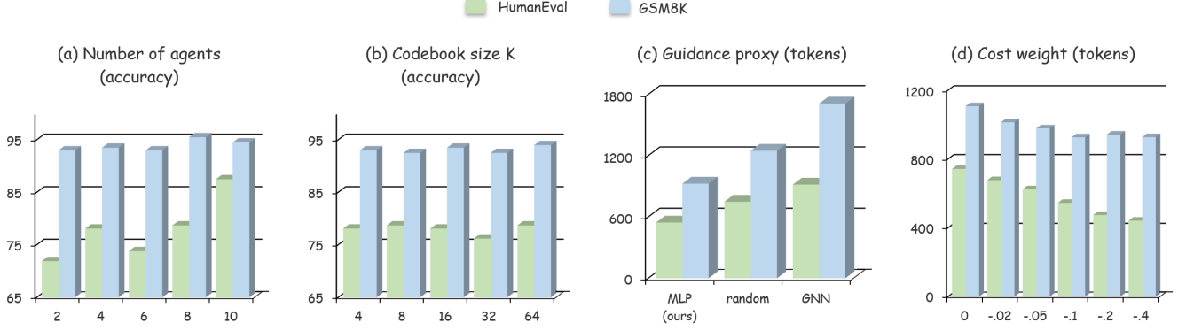
Figure 5: Ablations on GSM8K and homogeneous HumanEval. (a) Accuracy versus team size N (retrained per N on the same training budget). (b) Accuracy versus codebook size K ; used codes saturate near six for every K \geq 8 . (c) Mean tokens per query for MLP, random, and GNN reranking under a fixed candidate set. (d) Mean tokens versus the rerank cost weight \lambda_{\text{cost}} , with default -0.1 .
