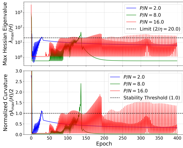
Fig. A.1 Learning dynamics of GD on the Ridge across varying storage loads ( P/N \in \{2.0, 8.0, 16.0\} ) at a fixed learning rate ( \eta = 0.1 ). (Top) Maximum Hessian eigenvalue \lambda_{\max}(\mathbf{H}) on a logarithmic scale. The initial curvature spike increases proportionally with the storage load P . (Bottom) Normalized curvature \eta\lambda_{\max}(\mathbf{H})/2 . Regardless of the load, the trajectory undergoes a transient self-stabilization phase near the 1.0 threshold before eventually escaping into the stable convergence regime.
