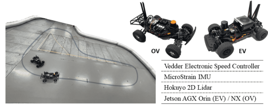
Fig. 5: 1/10th scale racing experiments setup. L-shape racing track and the vehicles' specifications.
