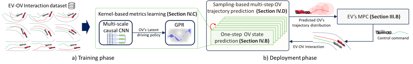
Fig. 2: The architecture of the proposed algorithm: (a) the training process of the one-step state prediction model, which utilizes the proposed kernel-based metrics learning for DKL; and (b) an autonomous racing algorithm for EV, which plans its maneuver based on the predicted trajectory distribution of OV.
