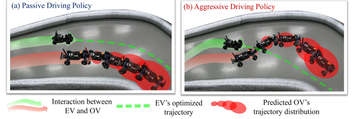
Fig. 1: Overtaking scenarios where the EV maximizes its progress while taking into account the predicted trajectory distribution of the OV, which is based on the driving policy inferred from the observed EV-OV interaction. (a) OV exhibits non-blocking behavior, allowing the EV to navigate without interference; (b) OV actively tries to block the EV's progress.
