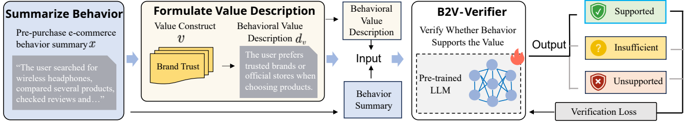
Figure 5: Overview of Value Verification Tuning. Given a behavior summary and verbalized value descriptions, B2V-Verifier determines whether the observed behavior supports the value and predicts a three-way verification label.
