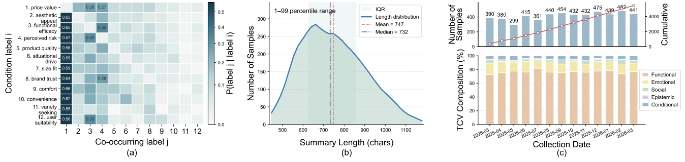
Figure 4: Characteristics of B2V-Bench. (a) Label co-occurrence patterns among frequent value constructs. (b) Distribution of behavioral summary lengths. (c) Monthly data volume and TCV composition over time.
