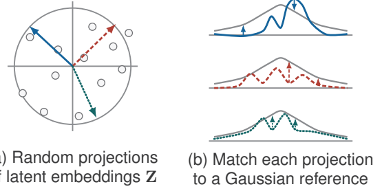
Figure 2: Illustration of SIGReg. Random one-dimensional projections are drawn from the latent embedding distribution, and each projected distribution is matched to a Gaussian reference.
