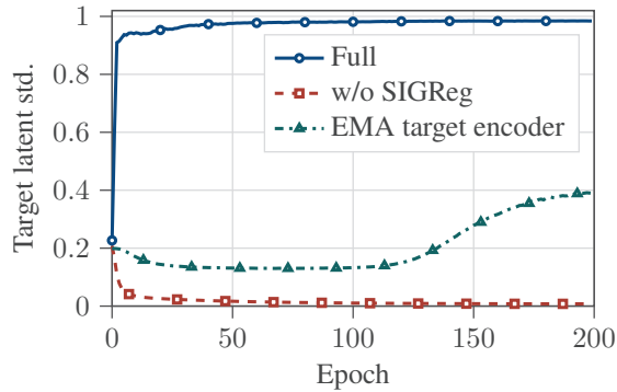
Figure 4: Target-latent standard deviation over pretraining epochs for representative component-ablation variants on MSRAAction-3D.
