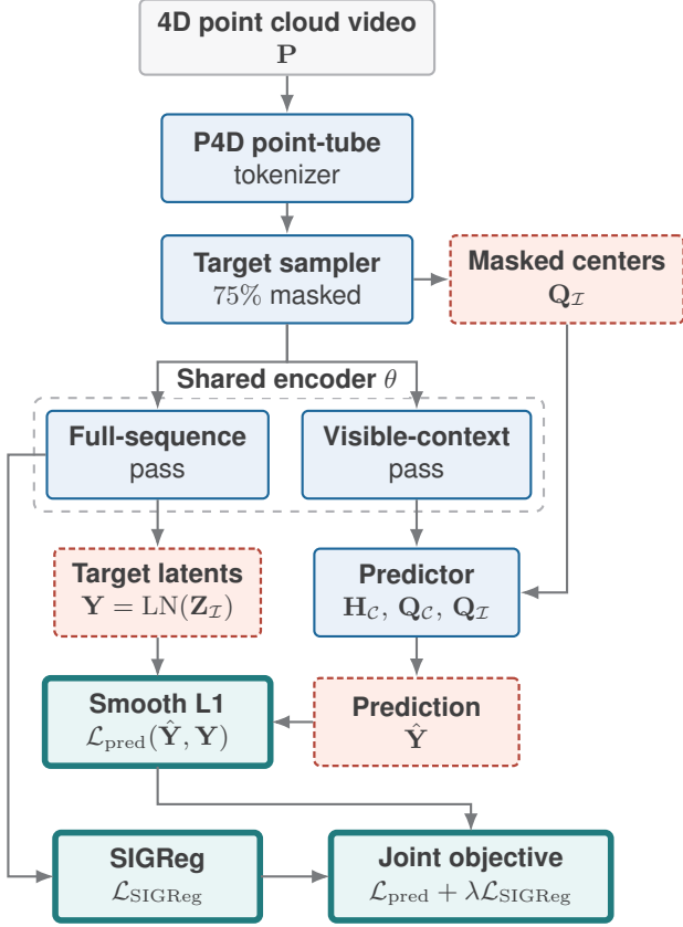
Figure 1: Overview of the proposed pretraining framework. Point-tube tokens are split into visible context and masked targets; a predictor infers target latents while SIGReg regularizes the latent distribution.
