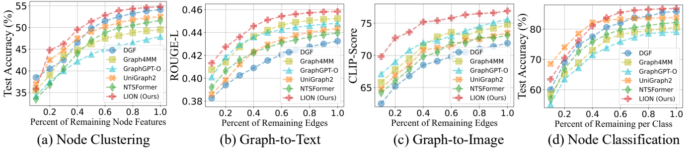
Fig. 5. Performance of LION under different sparsity levels on the Grocery dataset.
