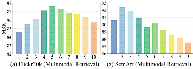
Fig. 3. Hyperparameter analysis of CGP depth.
