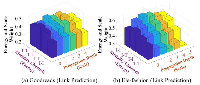
Fig. 4. AHA visualization. T and I are text and image; T-T, T-I, I-T, and I-I denote ordered modality-pair diagnostics rather than one-to-one Clifford basis blades.
