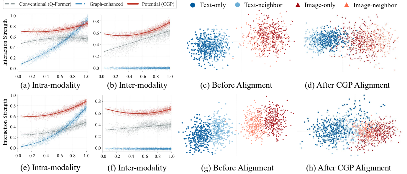
Fig. 2. (a)-(d) The G2Text visualization of CGP modality interaction and alignment (i.e., geometric-induced adaptive graph propagation) on Flickr30k. (e)-(h) The G2Image visualization of CGP modality interaction and alignment on SemArt.
