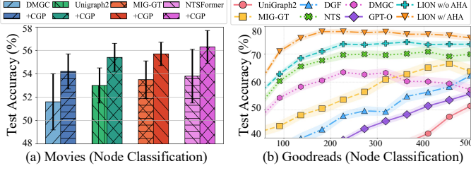
Fig. 1. Empirical evaluations of CGP (a) and AHA (b), where the x-axis for AHA (b) is training time in seconds.
