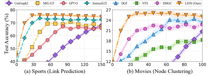
Fig. 6. The convergence efficiency curves.
