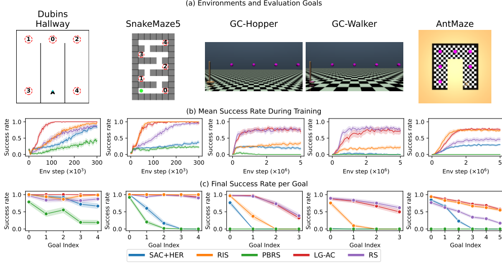
Figure 1: (a) The five goal-conditioned environments and the corresponding evaluation goal sets. (b) Mean success rate on the evaluation goal set during training. Each evaluation is repeated 10 times, with results reported as the mean and 95% confidence interval (computed with bootstrapping) over 30 seeds. (c) Final performance per individual evaluation goal for each method, averaged over the last five evaluations. In GC-Hopper and GC-Walker, RS achieves the best performance with LG-AC following closely behind, whereas in AntMaze, RIS and LG-AC perform best. In Dubins Hallway , PBRS has the worst performance, often failing to reach far-away goals.
