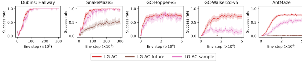
Figure 4: Mean success rate on the evaluation goal set during training. Each evaluation was repeated 10 times, with results reported as the mean and 95% confidence interval (computed with bootstrapping) over 10 seeds. LG-AC-future leads to low SR, only learning in SnakeMaze5 . LG-AC performs equally or better compared to LG-AC-sample.
