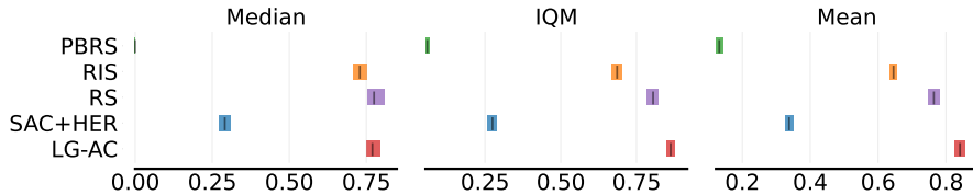
Figure 2: Aggregated median, interquartile mean (IQM), and mean performance across environments, computed from the last five final evaluations of each run shown in Figure 1. Confidence intervals are estimated using percentile bootstrap with stratified sampling [Agarwal et al., 2021] from 30 seeds. While RS, RIS, and LG-AC achieve similar median performance, LG-AC outperforms the baselines on all other metrics.
