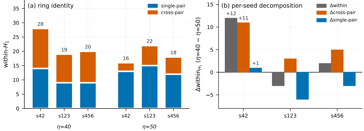
Figure 4: The ring identity. (a) For each of 3 seeds and both \eta_{40} / \eta_{50} FM0 pairs, the stacked bar shows within = single-pair rings (blue) + cross-pair same-class rings (orange), total labeled on top. The identity within = single + cross holds with zero residual at all 6 checkpoints (e.g., \eta_{40} s42: 14 + 14 = 28 ; \eta_{50} s42: 13 + 3 = 16 ). (b) Per-seed decomposition of the FM0-pair within difference ( \eta_{40} - \eta_{50} ) into \Delta single + \Delta cross. The single-seed (s42) reading ( \Delta within = +12, carried entirely by \Delta cross-pair = +11) does not survive: s123 is single-pair dominant with the \eta direction reversed ( -6/+3 ), s456 is mixed ( -3/+5 ). Only the identity itself and the FM0 val_acc record ( \sim 0.96 ) survive multi-seed.
