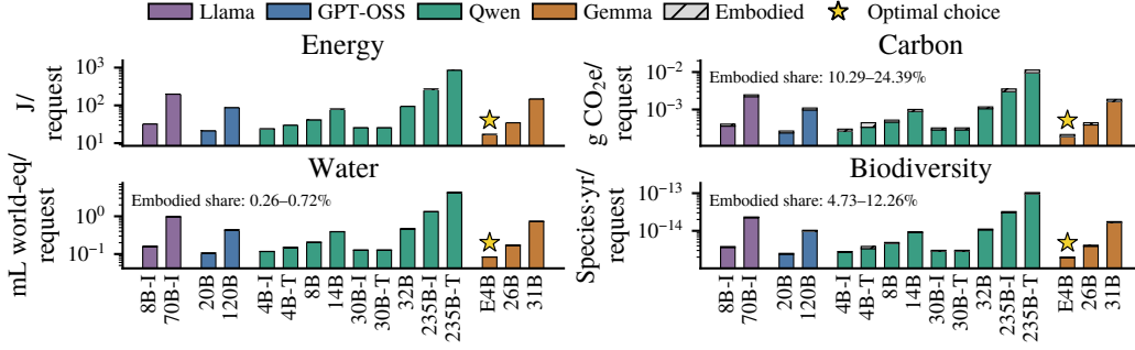
Figure 2: Impact of model family and size on per-request energy, carbon, water, and biodiversity. Solid and hatched bars denote operational and embodied impacts, respectively; stars mark the minimum-impact configuration for each dimension.
