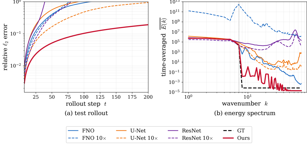
Figure 5: Partial-physics regime on the advection–diffusion benchmark. (a) Test-rollout relative \ell_2 error for the proposed surrogate and the purely data-driven baselines at matched and tenfold ( 10\times ) trainable dynamics-map budgets. (b) Time-averaged energy spectra; the dotted line marks the initial-condition band edge.
