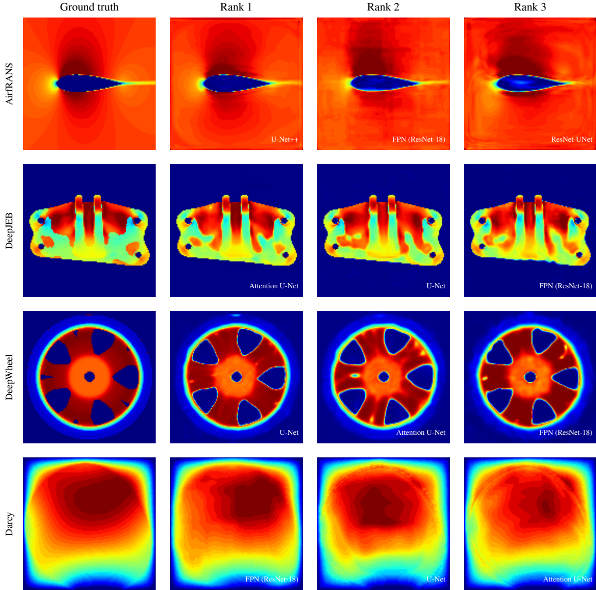
Figure 9: Qualitative 2D field prediction at scale XL. Each row shows ground truth and the top-three ranked models on one test sample per dataset, for AirfRANS: streamwise velocity u , DeepJEB: stress, DeepWheel: depth, and Darcy: pressure. Ranks are those of the field shown, not of the dataset aggregate over all of its targets. Each row shares a jet color scale, and the model is named in each panel.
