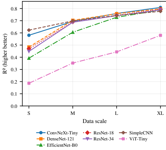
(a) 2D scalar prediction ( R^2 \uparrow )
