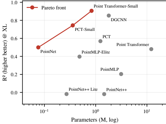
(a) 3D scalar prediction (DeepWheel)
