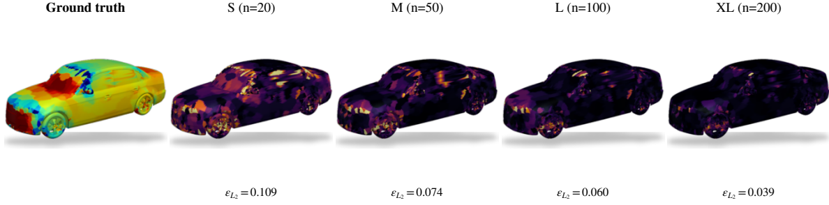
Figure 8: Field prediction error versus data scale on the DrivAerML surface-pressure case. The ground-truth pressure field is at left in jet, and the remaining panels map the absolute error |\text{pred} - \text{GT}| of GeoTransolver on the same held-out car for the model trained at scale S through XL, on one shared error scale where darker is lower error. Each panel is labelled with its relative L_2 error \epsilon_{L_2} .
