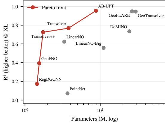
(b) 3D field prediction (DrivAerML)
