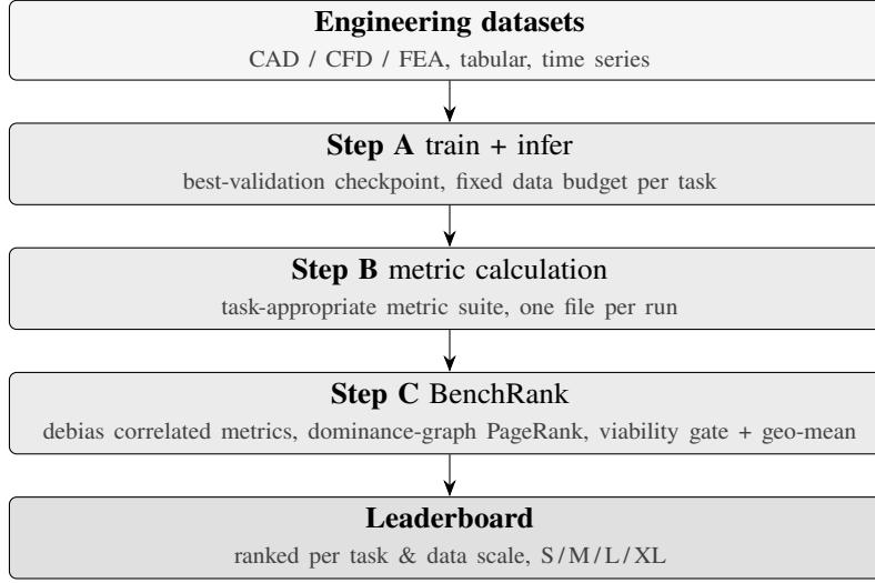
Figure 1: Overview of the PhysicsBench evaluation pipeline. The datasets combine industrial CAD/CFD/FEA simulation sets with established public references.
