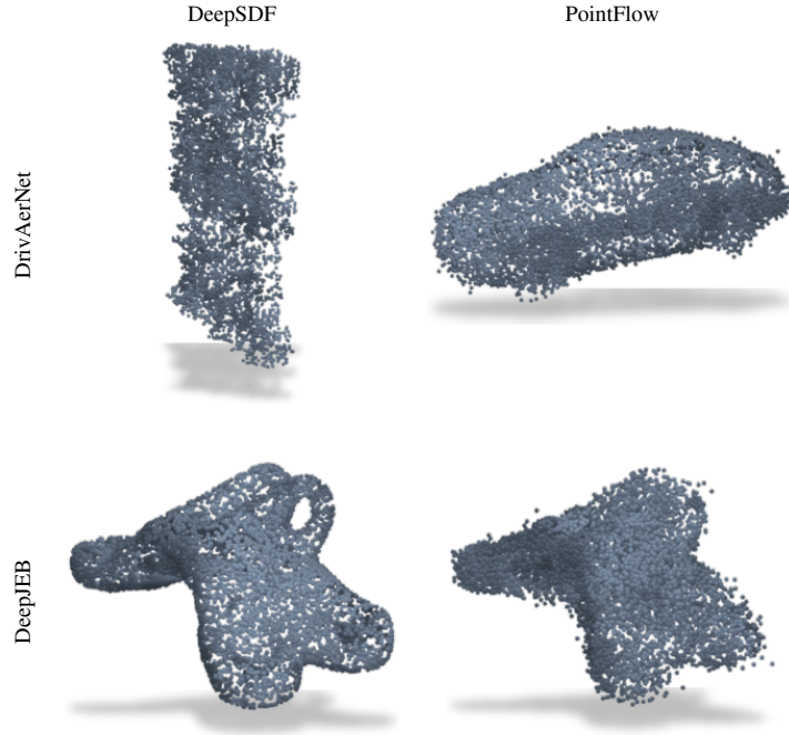
Figure 11: Qualitative 3D geometry generation at the smallest scale, with n=20 . Point clouds from the SDF auto-decoder DeepSDF and the continuous-normalizing-flow generator PointFlow on two datasets, namely DrivAerNet cars and DeepJEB brackets.
