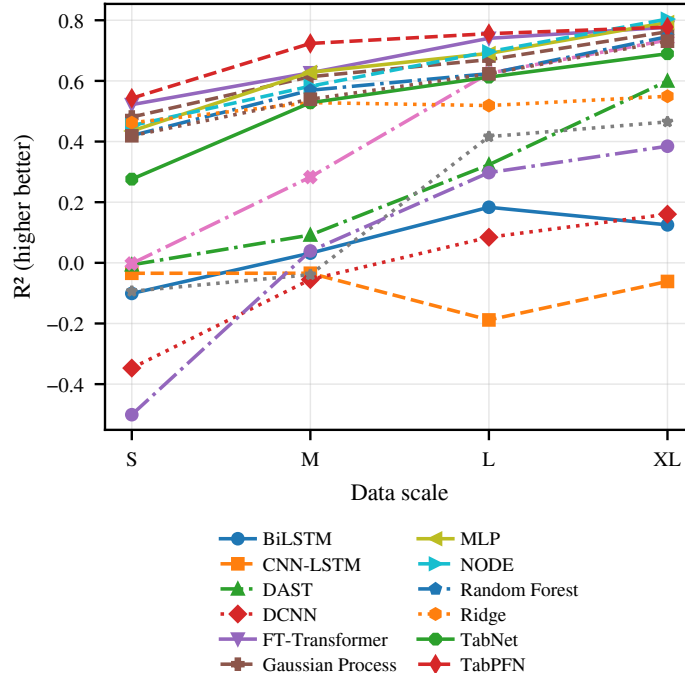
Figure 10: Primary accuracy R^2 versus data scale for 1D scalar prediction, one line per model. The tabular models are scored on Concrete and Airfoil pooled and the time-series models on CMAPSS, so the two pools share the axis without competing.
