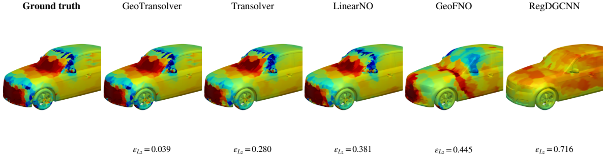
Figure 7: Local view of the DrivAerML surface-pressure case at scale XL. The ground truth is at left, followed by five models ordered best to worst from left to right by relative L_2 error.
