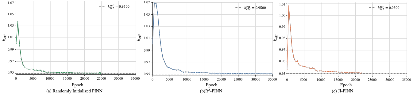
Fig. 9. Convergence history of k_{eff} for the three-dimensional single-group cubic case.
