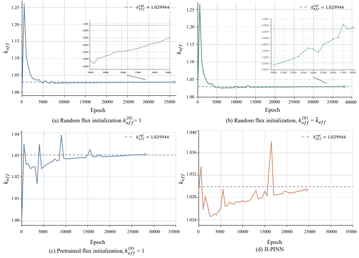
Fig. 5. Convergence histories of k_{eff} under different initialization configurations.
