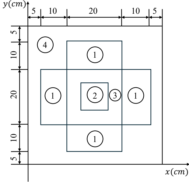
Fig. 6. Geometry and material distribution of the two-dimensional two-group four-material case.
