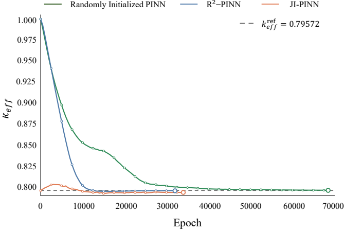
Fig. 7. Convergence history of k_{eff} for the two-dimensional two-group four-material case.
