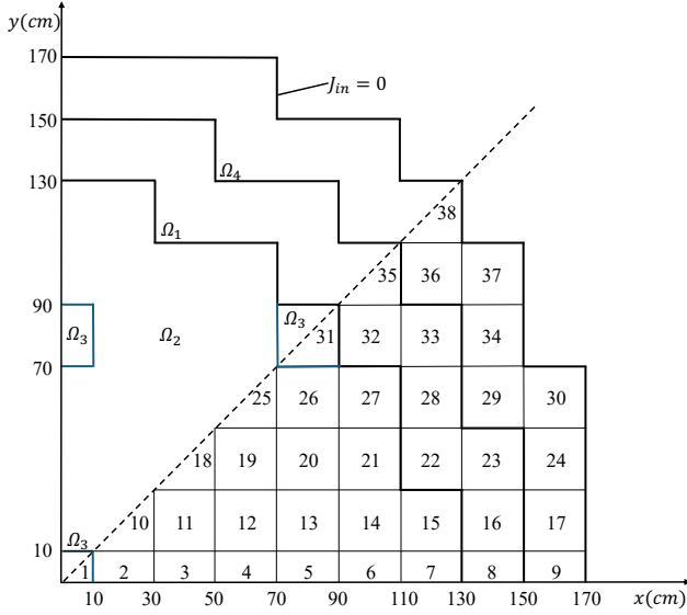
Fig. 4. Geometric layout of the IAEA 2D benchmark.
