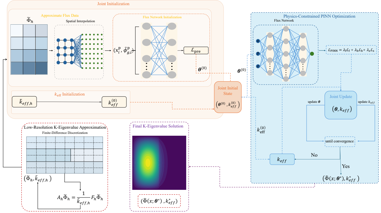
Fig. 1. Overall framework of JI-PINN.
