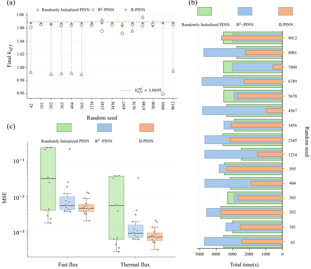
Fig. 3. Solution results and computational time for different random seeds: (a) final k_{eff} ; (b) total computational time; (c) MSE of the neutron flux for the fast and thermal groups.
