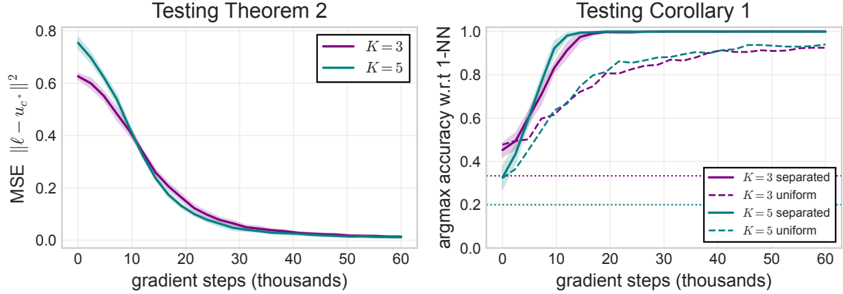
Figure 3: Distribution shift (Theorem 2) and argmax classification (Corollary 1). On the separated test distribution the logit MSE \|\ell - \mathbf{u}_{c_*}\|_2^2 \rightarrow 0 (left) and the argmax matches the 1-NN label (right). The uniform-data accuracy is shown for contrast.
