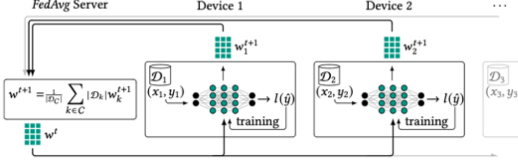
Figure 1: Schematic of a Federated Learning system where, the knowledge of devices 1, \dots , is shared through averaging the NNs’ weights. Each device trains on its disjoint local data D_1, \dots , producing newly trained weights w_1^{t+1}, \dots . Every round, the new averaged weights w^{t+1} are distributed to all devices. see in [25].
