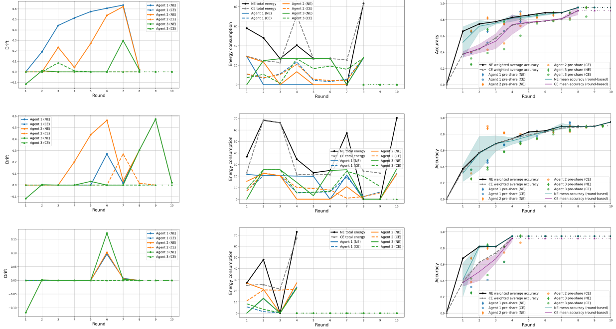
Figure 11: Blending effect. Drift per user (left column), energy consumption per agent (middle column), training accuracy (right column), for the case where agents are energy-aware, with \gamma = 1 (upper row), \gamma = 10 (middle row), and \gamma = 100 (lower row), with h = 1 .
