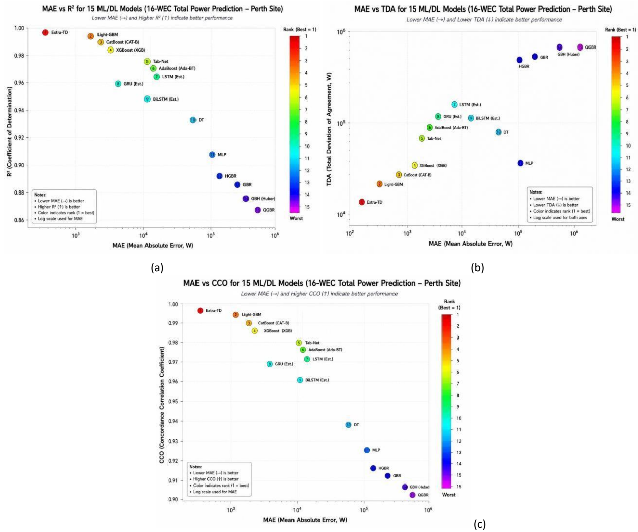
Figure 5: 2D performance comparison of 15 ML/DL models for 16-WEC total power prediction at the Perth site based on MAE– R^2 , MAE–CCO, and MAE–TDA relationships. Marker colors indicate the relative model ranking, with optimal performance characterized by lower MAE and TDA and higher R^2 and CCO.
