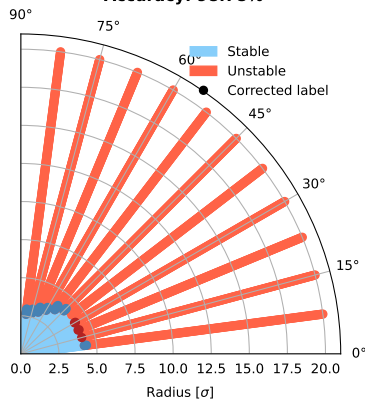
Predicted dynamic aperture for configuration 29472 Accuracy: 98.78%
