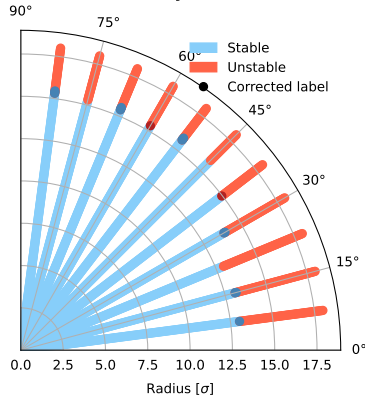
Predicted dynamic aperture for configuration 29876 Accuracy: 99.44%
