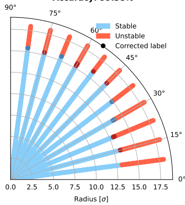
Predicted dynamic aperture for configuration 29876 Accuracy: 99.38%
