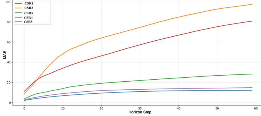
Figure 4: Evolution of forecasting drift over a 60-step (0-59) prediction horizon measured by horizon-wise MAE. Error increases progressively for all TPS traffic streams, with CSR2 and CSR4 exhibiting the largest drift, while CSR1, CSR3, and CSR5 maintain comparatively stable long-term prediction performance.
