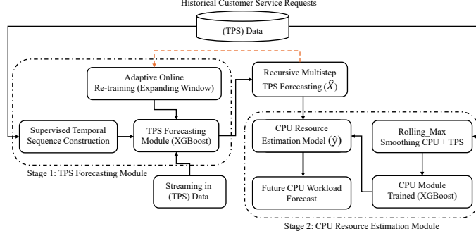
Figure 1: Architecture of the proposed two-stage integrated forecasting system with adaptive expanding-window retraining for proactive CPU resource prediction in private cloud.
