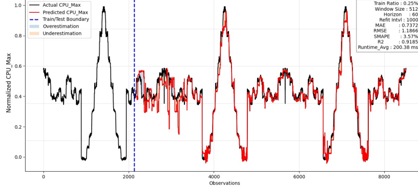
Figure 3: Performance analysis of the proposed two-stage integrated forecasting model for the application A , where a forecasting horizon of 60 corresponds to a 1-hour-ahead resource prediction.
