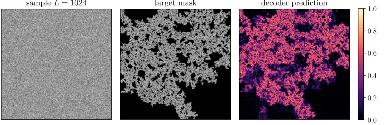
FIG. 1. Site-percolation configuration at criticality ( left ), mask of the spanning cluster ( center ), and prediction of the neural network ( right ). The lattice size is L = 1024 , which lies outside the training range and therefore probes finite-size extrapolation.
