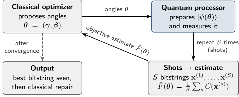
Figure 2: The hybrid variational loop used by QAOA and other variational quantum algorithms. The quantum processor acts as a parameterized sampler; all optimization of the parameters happens classically, using objective estimates obtained from S shots.
