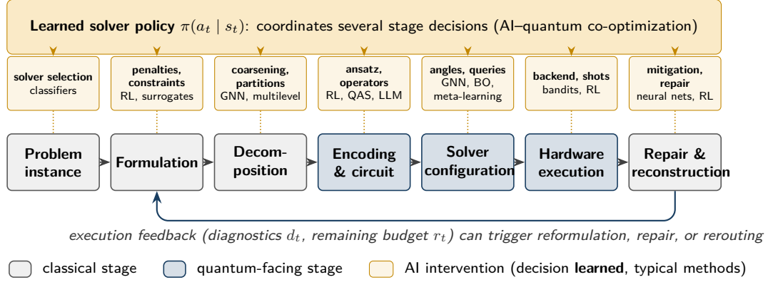
Figure 3: Pipeline view of AI intervention points and execution feedback. Each stage carries the decision that is learned and the AI methods typically used (Table 3). Component-level methods (AI-for-QO) act on a single stage; co-optimization methods learn a policy that coordinates several stages, conditioned on execution feedback.
