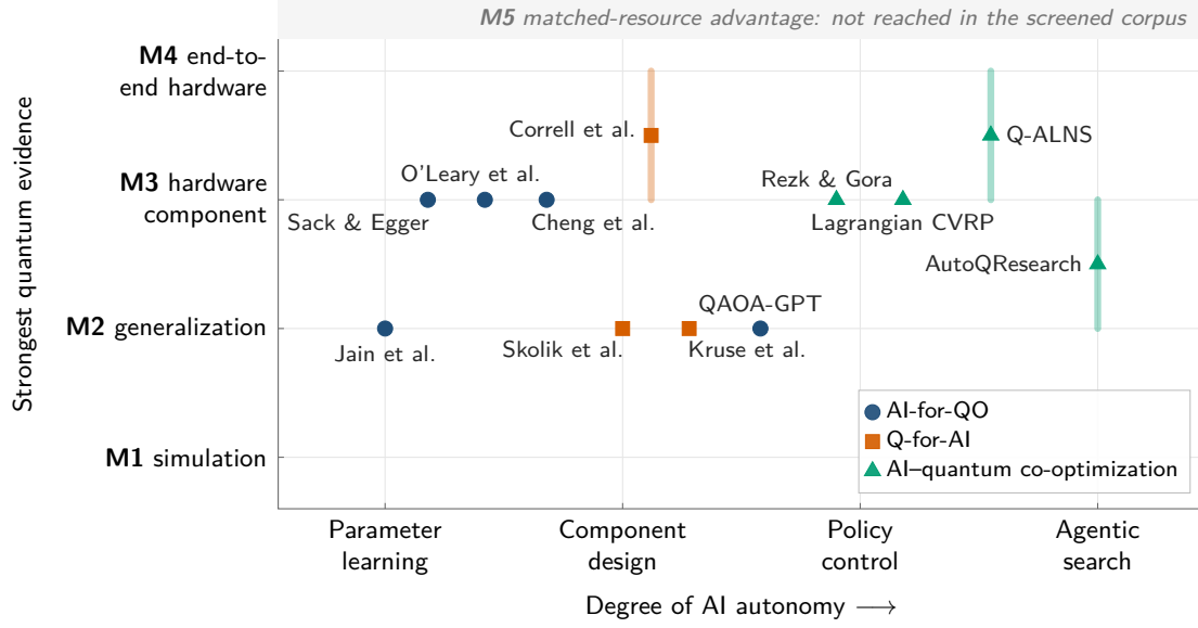
Figure 4: Degree of AI autonomy versus the strongest quantum evidence reported by representative studies. Vertical positions are the maturity levels coded in the evidence matrix (Section A); translucent bars mark studies coded as a range (e.g., M3–M4), with the marker at the midpoint. Horizontal positions are qualitative. Marker shape and colour indicate the paradigm.
