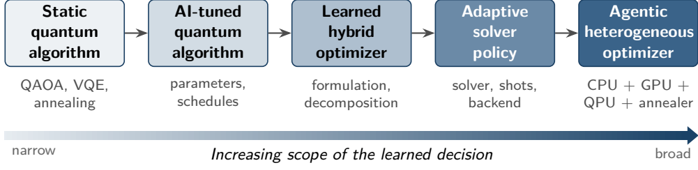
Figure 1: Increasing scope of learned decisions in quantum combinatorial optimization. Each stage widens what is learned (labels below each box), from a fixed quantum algorithm to policies that allocate work across heterogeneous classical and quantum resources.
