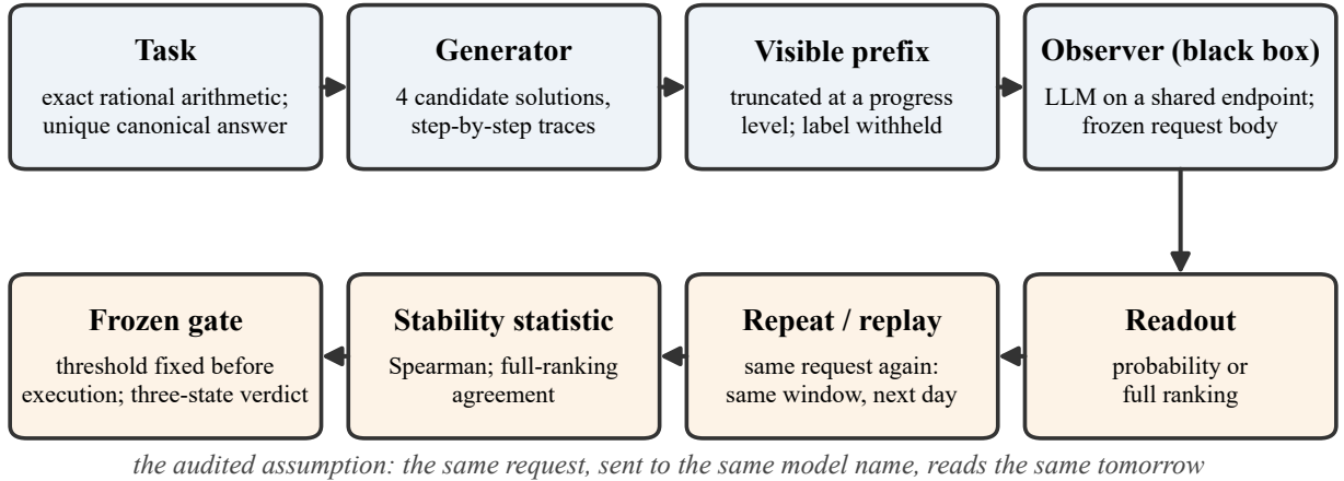
Figure 1: The measurement chain. A generator writes four candidates per exact-arithmetic task; a black-box LLM observer sees the task plus a truncated trace prefix and returns a probability or full ranking; repeats and replays feed a stability statistic against a threshold fixed before execution. The paper audits the italicised assumption.
