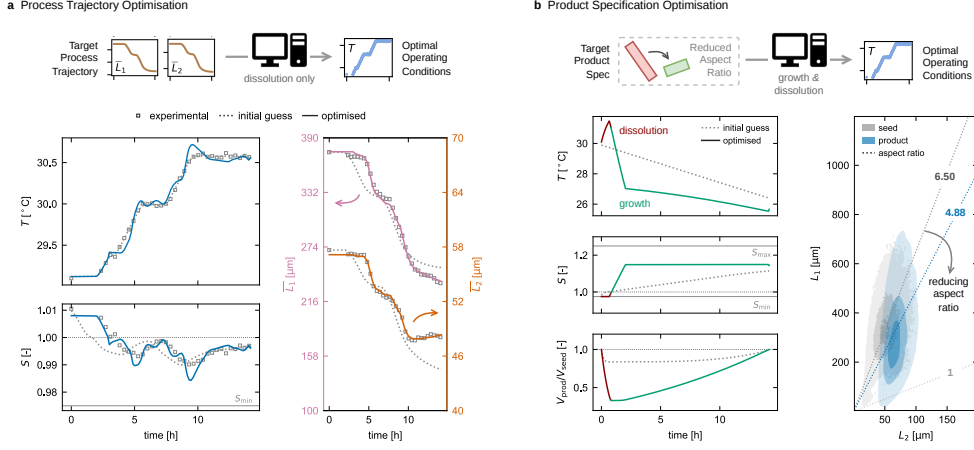
Fig. 3 End-to-end optimisation of operating conditions recovers real process trajectories and proposes new conditions to meet a product specification. (a) Process trajectory optimisation. Using the frozen hybrid dissolution model (Figure 2), the temperature profile T(t) and initial condition (f_0, c_0) are optimised (solid) from an initial guess (dotted) to match the observed \bar{L}_1 (pink) and \bar{L}_2 (orange) trajectories of the held-out experiment E5 (open squares). The optimised S(t) remains within the S_{\min} bound throughout, and the recovered T(t) closely tracks the true experimental profile despite the profile never being provided as an optimisation target. (b) Product specification optimisation. Using the size-dependent growth & dissolution model with the initial condition of E5, T(t) is optimised (solid, from a linear dissolution \rightarrow growth initial guess, dotted) to reduce the final product aspect ratio subject to S_{\min} , S_{\max} , and a volume-conservation constraint ( V_{\text{product}}/V_{\text{seed}} \geq 1 ). The optimal profile first dissolves the seed population ( S < 1 , red, with volume falling to \approx 35\% ) before switching to growth ( S > 1 , green, with volume recovering to 100%). The seed (grey) and product (blue) PSSDs are shown, with dotted lines marking the aspect ratio ( \bar{L}_1/\bar{L}_2 ) of each. The optimised profile reduces the aspect ratio from 6.50 to 4.88 (25% reduction) with the same final mass.
