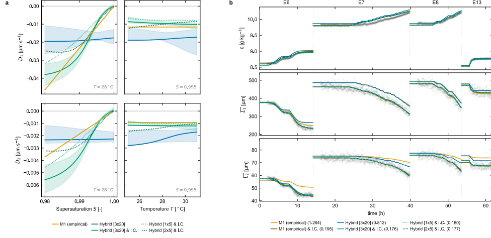
Fig. 5 Learned functional forms and predictive performance. (a) Learned dissolution rate functional forms D_1 and D_2 vs. supersaturation S (fixed T = 28^\circ\text{C} , left) and vs. temperature T (fixed S = 0.995 , right), for the M1 empirical baseline and hybrid models of varying architecture ( 1 \times 5 , 2 \times 5 , 3 \times 20 hidden layers \times nodes), with and without joint IC assimilation. Shaded bands give the spread across the 20-member ensembles where multiple models were trained. Importantly, this shows how the hybrid model trained on the measured initial condition can learn a non-physical form, with the rate never approaching zero at S = 1 . (b) Predicted vs. measured trajectories for the four validation experiments (E6, E7, E8, E13) across all three target metrics ( c , \bar{L}_1 , \bar{L}_2 ). Legend values give the combined trajectory loss across these experiments for each model. IC assimilation improves the fit for both the empirical (M1) and hybrid models, with the largest gain for the hybrid model, and the improvement is consistent across network architecture.
