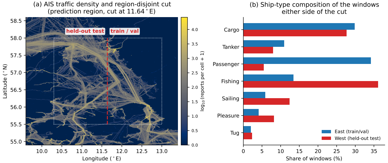
Figure 1: Study area. (a) AIS traffic density over the prediction region (log-scaled report counts per grid cell, four sample days spread across the month). The dotted box is the 10.3–13.0°E, 55.5–58.0°N region of the prediction and imputation windows, and the dashed line is the region-disjoint cut at the median anchor longitude (11.64°E), with the western side held out for test. Coastlines and traffic separation schemes are traced by the reports themselves; no basemap is overlaid. (b) Ship-type composition of the region-manifest windows on either side of the cut. Types are each vessel’s modal static AIS type, available for 94.5% of the windows.
