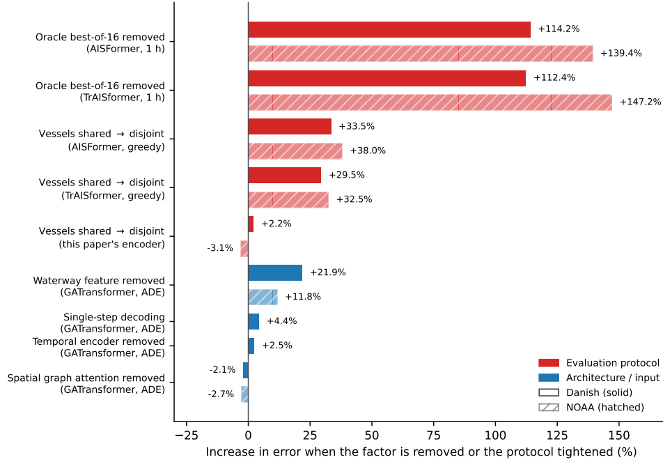
Figure 8: Increase in error when a factor is removed or the protocol tightened, from the results in Sections 5, 5.2, 6 and 6.1. Protocol effects (red) exceed the architectural ones (blue) for the two TrAISformer-family comparators, on both corpora; the compact encoder, which shows little to no benefit from shared vessels, is the exception on both. Each percentage is the stricter error over the more permissive one; a 23% reduction in the text corresponds to a 30% increase here. Solid bars are Danish, hatched bars are NOAA. The two are not on an identical footing: Danish protocol-effect bars are ratios to constant velocity on each split's own test set (Table 9), controlling for the three regimes' unequal difficulty, whereas NOAA bars use raw km (Table 12), since NOAA lacks a constant-velocity control on every split; NOAA bars are therefore only comparable to their Danish counterparts in sign and rough magnitude, not exactly. Two GATransformer architectural ablations (single-step decoding, temporal encoder) were not rerun on NOAA and have no hatched bar.
