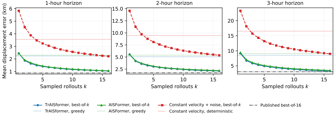
Figure 4: Mean displacement error against the number of sampled rollouts k under best-of- k selection, vessel-disjoint test split. Both systems and a noise-perturbed constant-velocity control improve steeply with k , because selection consults the ground truth; the control learns nothing from the trajectory, so its descent is due to the protocol. Dotted lines: deterministic error; dash-dotted line: published best-of-16 value. The two systems' curves overlap at every horizon.
