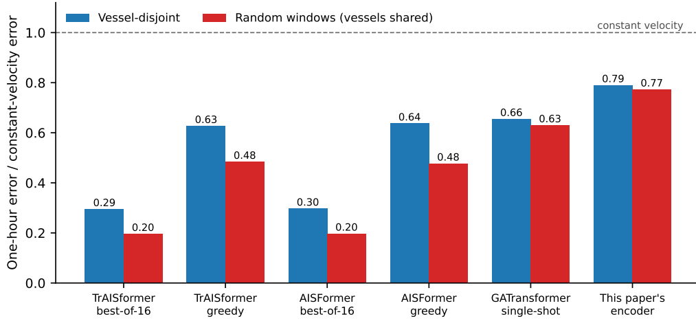
Figure 7: One-hour error as a fraction of constant-velocity error on each regime's own test split, under vessel-disjoint and random-window splits (values from Table 9). The two autoregressive TrAISformer-family comparators lose 23–25% of their greedy ratio when vessels are shared; the compact in-house encoder loses 2%.
