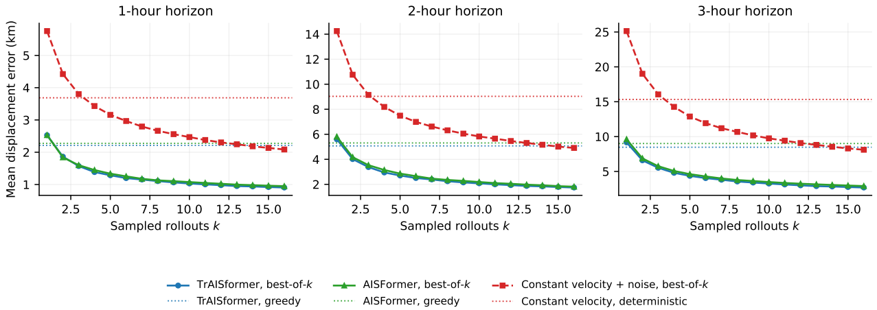
Figure 5: NOAA counterpart of Fig. 4: mean displacement error against the number of sampled rollouts k , vessel-disjoint test split, seed 42. Both systems again improve steeply with k and overlap at every horizon; there is no “published best-of-16” reference line here, since that value is TrAISformer’s own reported number on Danish waters and has no NOAA analogue.
