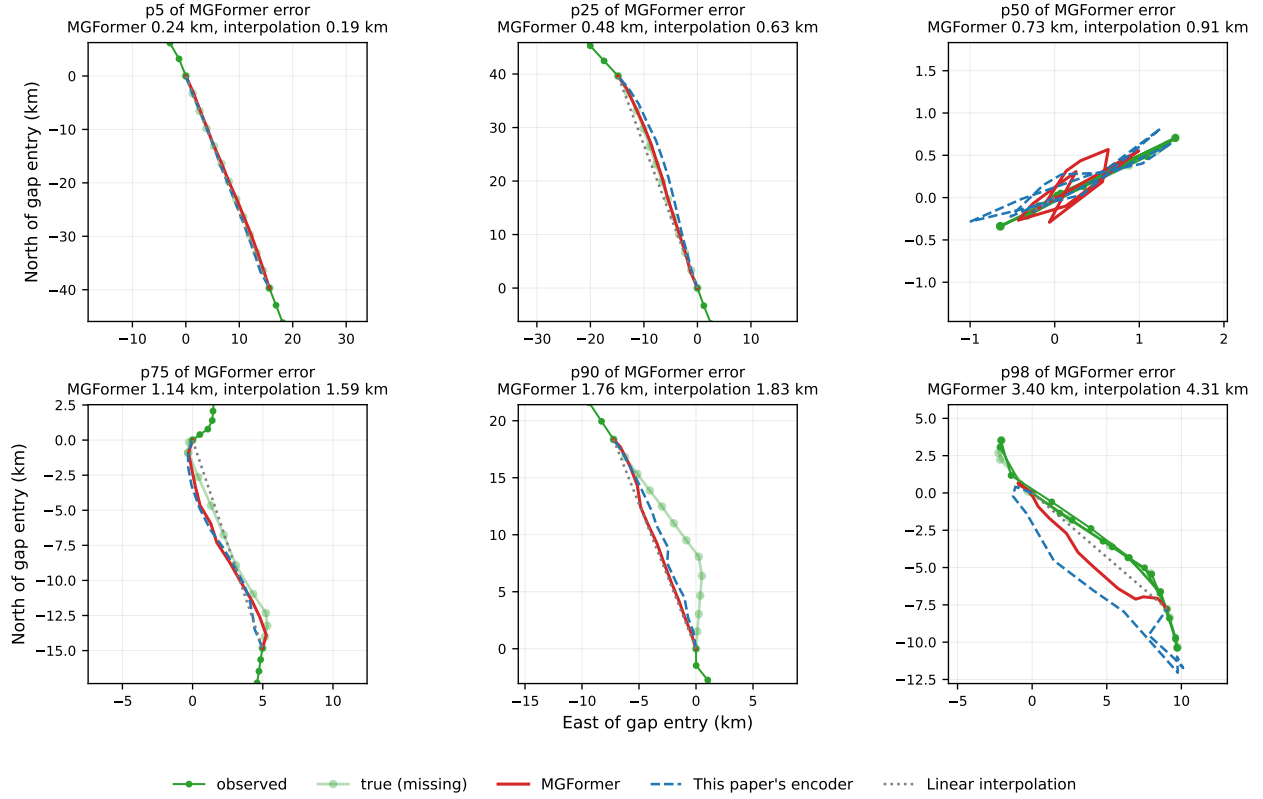
Figure 6: Six imputed gaps from the vessel-disjoint test split, drawn at fixed percentiles of MGFormer's per-window error; within each percentile band the window with the median interpolation error is shown (rule-based, not hand-picked). Each panel is framed in kilometers on the last observed report, and the scale differs between panels (about 45 km across at p5, about 3 km at p50). Green: observed steps; pale green: the eleven missing steps. In the median-error example neither learned system is reliably better than the straight line; the average advantage is carried by the minority of gaps where interpolation fails badly (see text).
