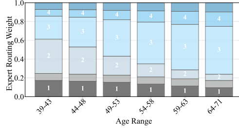
(a) UKB-Center
