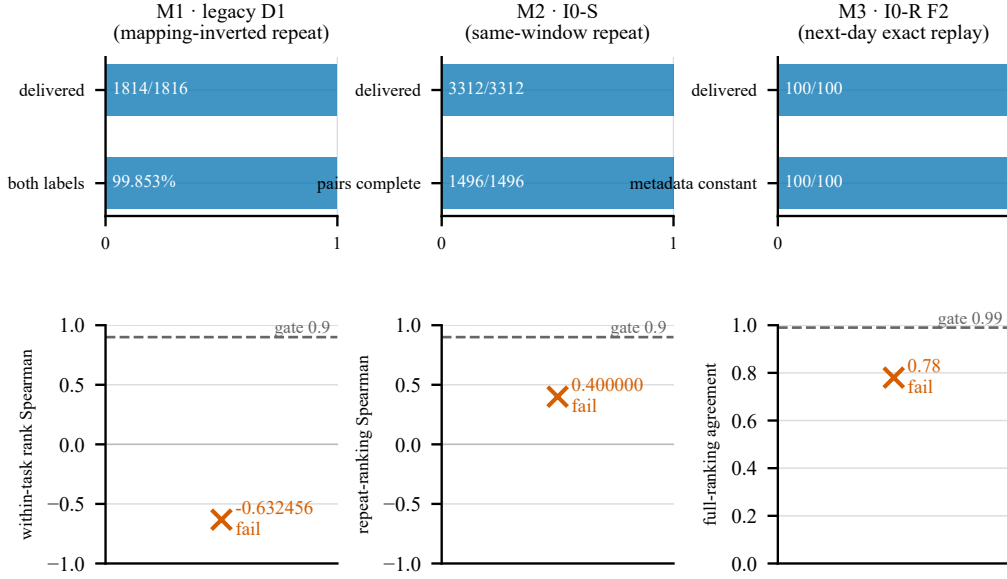
top: execution integrity (delivery, validity, metadata constancy) — at ceiling in all three campaigns; bottom: the preregistered verdict against its frozen gate — fail in all three.
