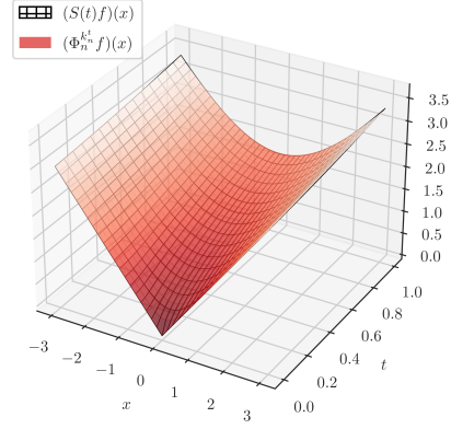
(E2) Approximation of S(t)f^{ab} by \Phi_n^{k_n^t} f^{ab} .
