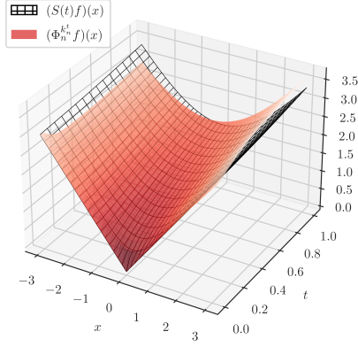
(C2) Approximation of S(t)f^{ab} by \Phi_n^{k_n^t} f^{ab} .
