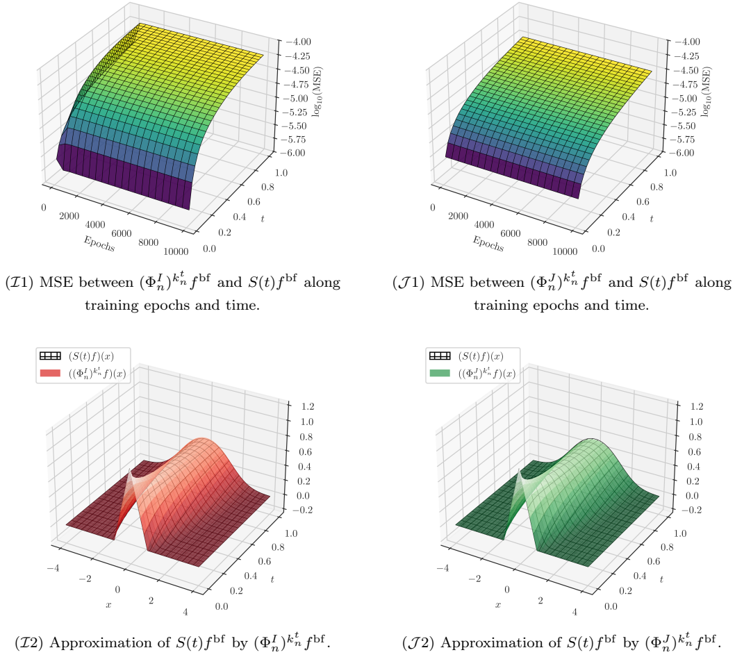
FIGURE 5. Approximating the Wasserstein-perturbation semigroup f \mapsto S(t)f with two envelope-neural operators, evaluated on the out-of-sample butterfly f^{\text{bf}} in (5.19). The operator \Phi_n^I in (5.16) in (I1)-(I2), and the operator \Phi_n^J in (5.17) in (J1)-(J2). In (I1)+(J1), the MSE between the iterations (\Phi_n^I)^{k_n^t} f^{\text{bf}} , respectively (\Phi_n^J)^{k_n^t} f^{\text{bf}} , and S(t)f^{\text{bf}} is displayed along the training epochs and the time t = kh_n , k = 1, \dots, n . In (I2)+(J2), the approximation of S(t)f^{\text{bf}} by the two iterated neural operators is compared with the finite difference solution of the corresponding HJB equation over [0, T] .
