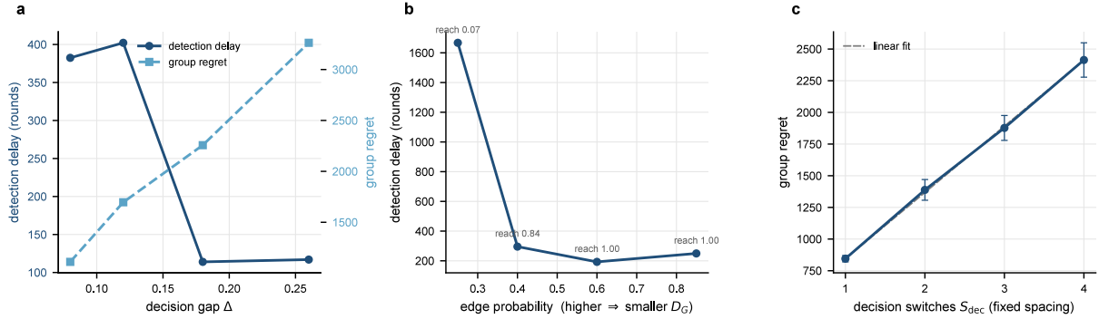
Figure 14: Switching-regime stress at S_{\text{dec}} > 0 ( N = 12 , K = 4 , 20 seeds), validating the bound's three dependences. (a) Detection delay falls with the gap \Delta (easier certification, the \mathcal{C}_r \sim (K-1)/\Delta branch) while regret rises with \Delta (the monitoring branch, each wasted pull costing \Delta ). (b) Detection delay collapses as connectivity rises and the reach rate climbs, the NS_{\text{dec}}D_G delay term. (c) Group regret grows linearly in S_{\text{dec}} at fixed inter-switch spacing, the NS_{\text{dec}} switch term. Reproduced by the switching-regime stress sweep.
