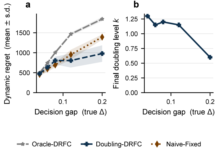
Figure 12: Geometric scan-budget walk-up for Gap-Adaptive DRFC (labeled Doubling-DRFC in the plot). Mean walk-up \leq 1.5 levels across a 5\times range of \Delta , matching oracle-tuned regret.
