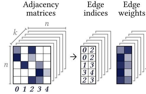
Figure 4: Adjacency matrices → edge states.
