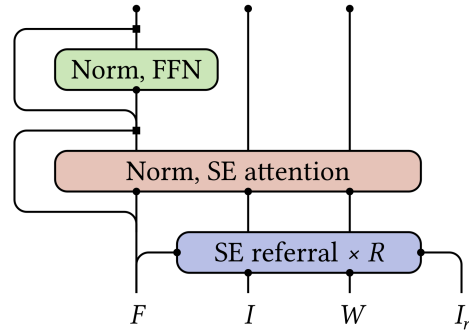
Figure 6: A sparse GM layer.
