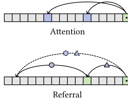
Figure 1: Attention and referral viewed as pointer operations.
