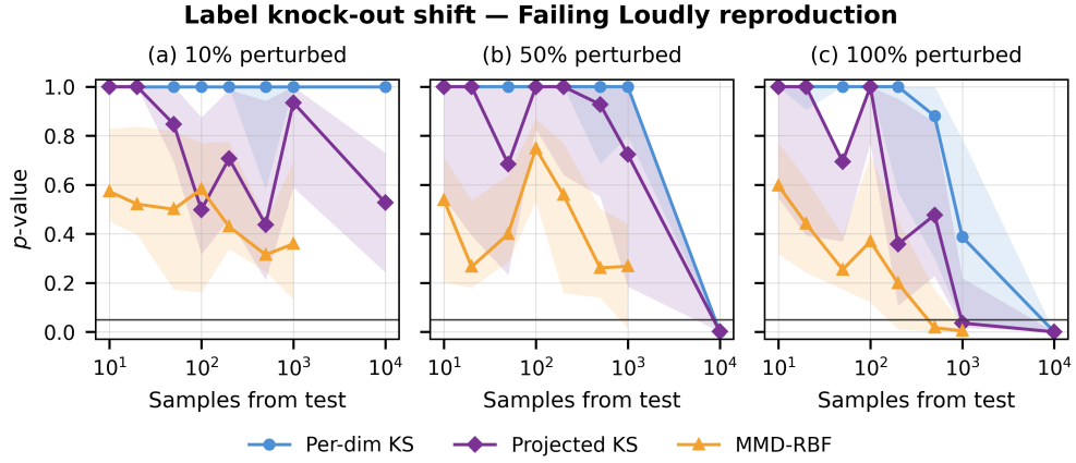
Fig. 8 Failing Loudly reproduction: class knock-out (label) shifts. Panels correspond to \{10\%, 50\%, 100\% perturbed test data. Because knock-out shifts change P(Y) rather than P(X) , MMD-based tests detect the shift through its indirect effect on the observed covariate distribution.
