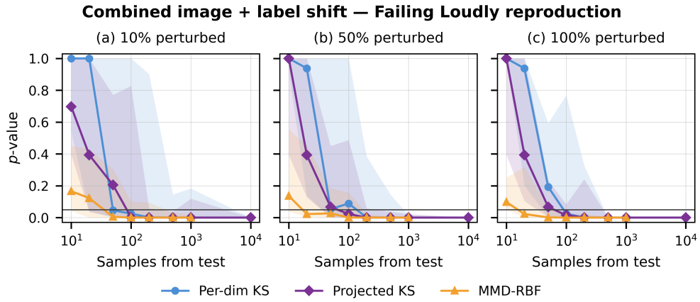
Fig. 9 Failing Loudly reproduction: combined image transformation + class knock-out shifts. Panels correspond to \{10\%, 50\%, 100\% perturbed test data. Combined shifts show the sharpest median- p descent because covariate and label distributions shift jointly.
