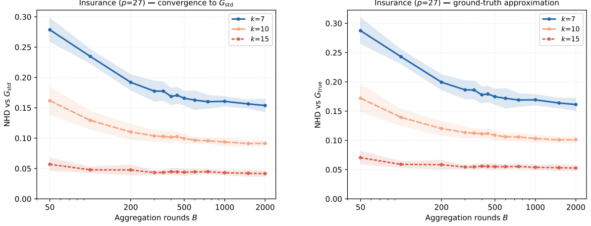
Figure 2: Convergence of subsample-aggregated GES+BDEU with B for Insurance ( p=27 ) at k \in \{7, 10, 15\} , evaluated at the fixed threshold \tau = 0.5 used in the main experiments. Left: NHD vs. G_{\text{std}} (convergence to standard learner). Right: NHD vs. G_{\text{true}} (ground-truth approximation). Shaded bands: \pm 1 std over 10 seeds.
