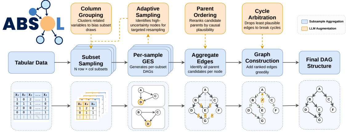
Figure 1: The ABSOL algorithm. Blue components form the subsample-aggregated GES+BDEU backbone, and orange components are the four bounded LLM augmentations, each acting at a fixed decision point. Graph construction is specified fully in Algorithm 1.
