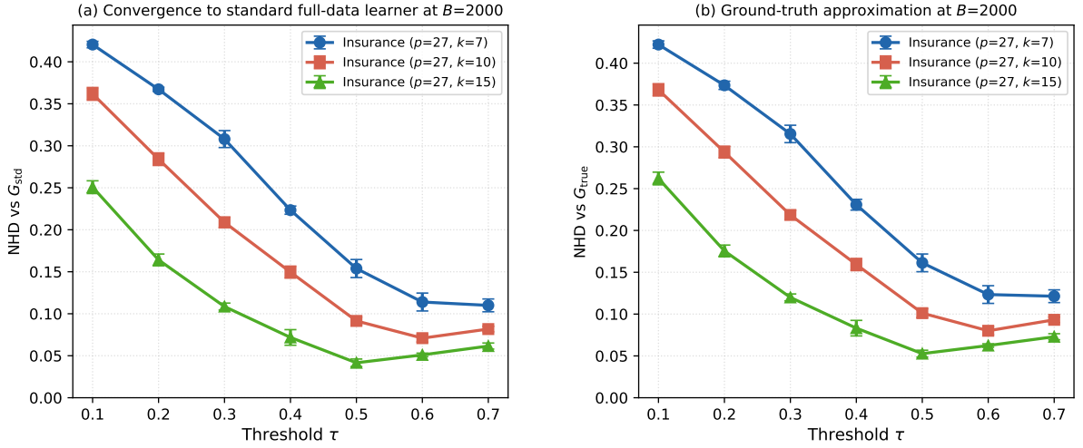
Figure 3: \tau sensitivity at B = 2000 on Insurance ( p=27 ). NHD vs. G_{\text{std}} (left) and vs. G_{\text{true}} (right) as a function of \tau for k \in \{7, 10, 15\} . Error bars: \pm 1 std over 10 seeds. The optimal \tau decreases from 0.70 to 0.50 as k increases.
