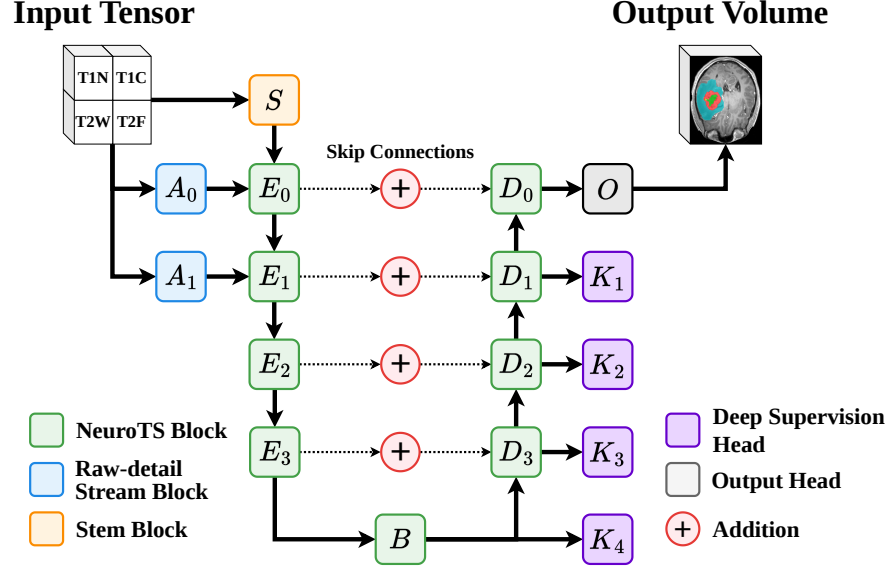
Fig. 1. Overview of the proposed NeuroTS-Net architecture.
