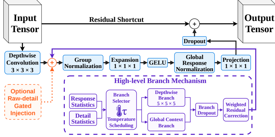
Fig. 2. Overview of the proposed NeuroTS block.
