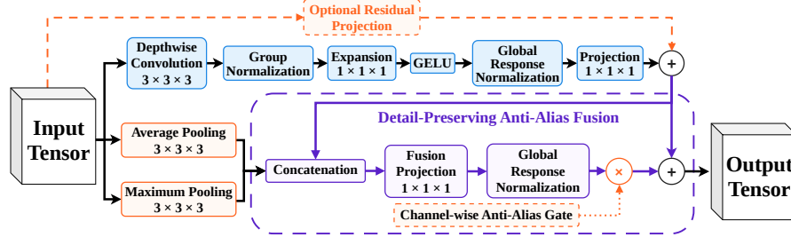
Fig. 3. The proposed detail-preserving multipath downsampling mechanism.
