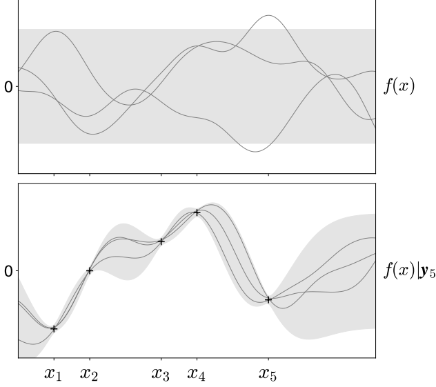
Fig. 1. GP prior (top) and GP posterior (bottom), i.e., the GP prior conditioned on observations (indicated by + markers). The solid lines represent sample functions drawn from the GP. The shaded area covers \pm 1.96 standard deviations from the mean. Example adapted from [1, Ch. 2].
