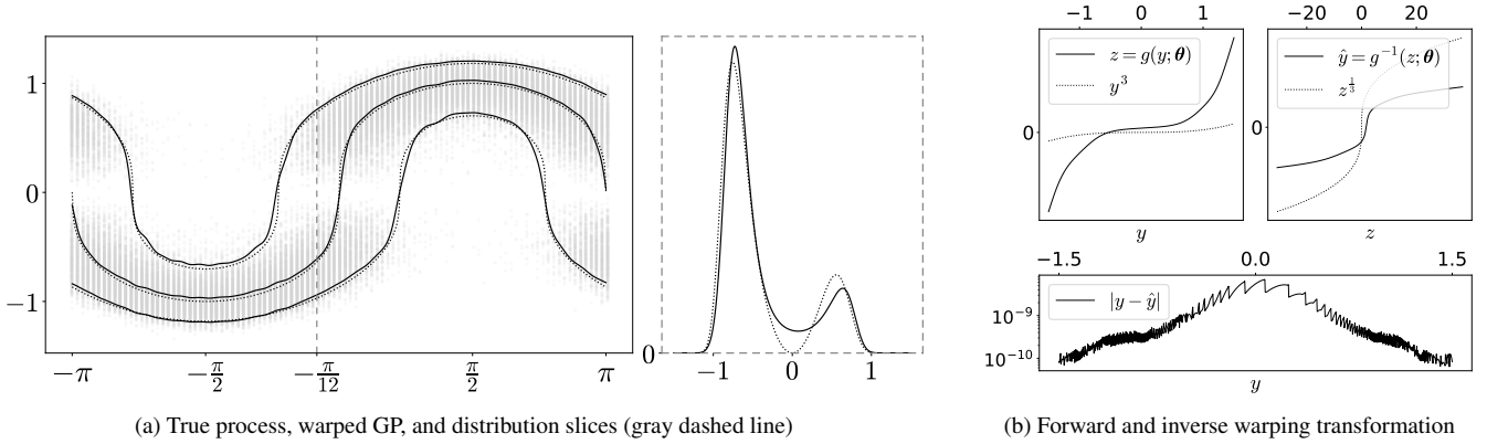
Fig. 2. In Fig. 2a, the observations are marked with gray dots. The dotted lines show the true generating distribution p(\mathbf{y}) and the solid lines show the warped GP prediction p(\mathbf{y}|\boldsymbol{\theta}) . The triplets of lines represent the median, along with the 2.5th and 97.5th percentiles in each case. The cross-section shows the probability densities at x = -\frac{\pi}{12} ; that is, p(y|x = -\frac{\pi}{12}) and p(y|\boldsymbol{\theta}, x = -\frac{\pi}{12}) . Fig. 2b shows the forward-inverse pass of the estimated warping transformation as well as its inversion error.
