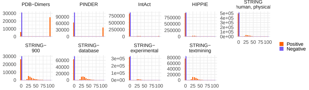
Figure A1: Percentage of identical residues (BLAST pident output) between the interaction candidates of the training datasets.
