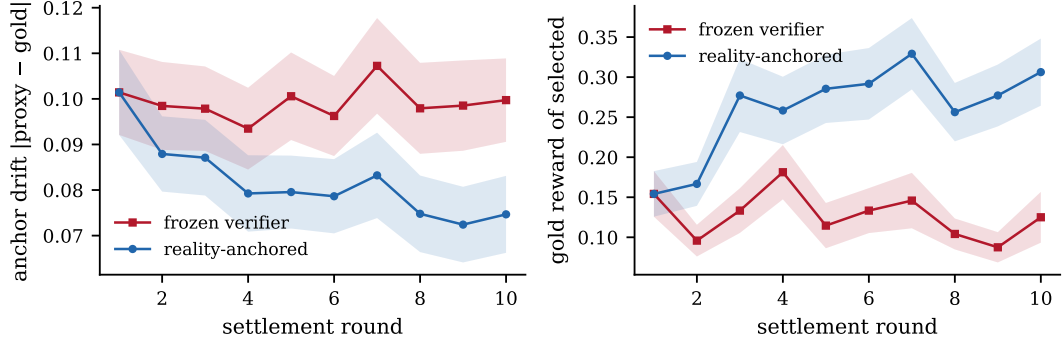
Figure 4: The settlement loop of Algorithm 1 in miniature (60 tasks, \pm 1 s.e.). Left: anchor drift |\text{proxy} - \text{gold}| on selected claims. Anchored settlement reduces drift by 26%; the frozen verifier does not improve. Right: gold reward of the top selection per round. Anchoring roughly doubles achieved reward ( 0.154 \rightarrow 0.306 ) while the frozen verifier stagnates and slightly degrades ( 0.154 \rightarrow 0.125 ).
