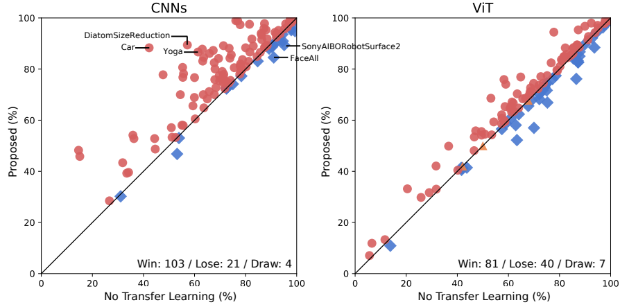
Figure 5: Dataset-wise comparison between the proposed Shapelet Matching multi-source transfer learning and no transfer learning. Each point represents one UCR target dataset and reports the average accuracy over three fine-tuning runs. The x-axis shows the no-transfer accuracy, and the y-axis shows the accuracy obtained by the proposed method; points above the diagonal indicate improvement and points below the diagonal indicate degradation. Red points indicate wins for the proposed method, and the win/loss/draw counts summarize the 128 target datasets for each displayed backbone.
