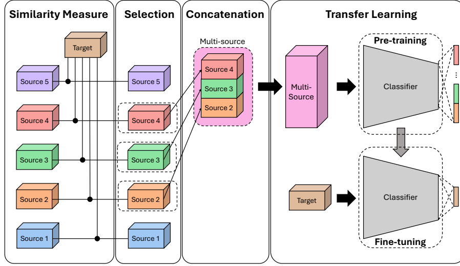
Figure 1: End-to-end overview of the proposed multi-source transfer learning framework. In the Similarity Measure stage, class-discriminative shapelets are discovered from the target dataset and each candidate source dataset using the matrix profile-based procedure, and each source is assigned a Shapelet Matching distance to the target. In the Selection stage, sources are ranked by this distance and the top- K sources (dashed boxes) are retained. In the Concatenation stage, the selected sources are resized to the target temporal length, their label spaces are remapped into a unified multi-source label set, and the datasets are balanced so that each source contributes the same number of samples. In the Transfer Learning stage, a backbone network is pre-trained on the aggregated multi-source dataset and then fine-tuned on the target dataset with a target-specific classifier head.
