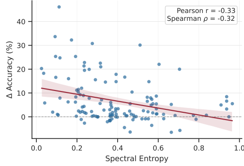
Figure 6: Accuracy gain of Shapelet Matching over no transfer learning versus normalized spectral entropy across 128 UCR datasets (VGG, K = 16 ). Each point represents a target dataset; the red line and shading show the linear regression fit and its 95% confidence interval. Lower (higher) entropy indicates spectral power concentrated in fewer (spread across more) frequencies.
