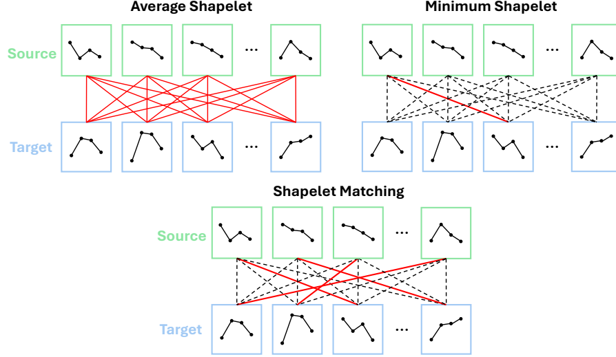
Figure 2: Comparison of the three shapelet-based dataset-similarity measures. Green boxes denote shapelets extracted from a source dataset, and blue boxes denote shapelets extracted from the target dataset. Red connections indicate the source–target shapelet pairs whose Euclidean distances are averaged to compute the dataset distance, whereas dashed black connections indicate candidate pairs that are not used in the final aggregation. Average Shapelet averages all possible pairs, Minimum Shapelet uses only the closest pair, and Shapelet Matching greedily selects multiple non-overlapping closest pairs.
