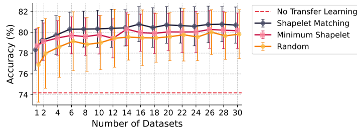
Figure 3: Effect of the number K of selected source datasets on VGG multi-source transfer learning. The y-axis reports the mean classification accuracy over the 128 UCR target datasets, and the dashed horizontal line indicates the no-transfer baseline. Error bars indicate the average per-target standard deviation over three fine-tuning runs.
