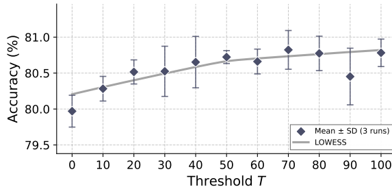
Figure 4: Performance transition from Minimum Shapelet to Shapelet Matching on the VGG backbone under the K = 16 multi-source setting. The point at threshold 0 denotes the Minimum Shapelet, which uses the single closest shapelet pair. For each positive threshold T , the score averages the smallest \lfloor (T/100)M \rfloor distances among the M one-to-one pairs produced by the greedy matching procedure; at threshold 100, all matched pairs are included, yielding full Shapelet Matching as described in Algorithm 2. For each run, classification accuracy is averaged over the 128 UCR target datasets; diamonds and error bars show the mean and standard deviation across three runs, respectively. The gray dotted curve represents LOWESS smoothing ( \text{frac} = 1.0 , three robust reweighting iterations) and is included only as a visual guide.
