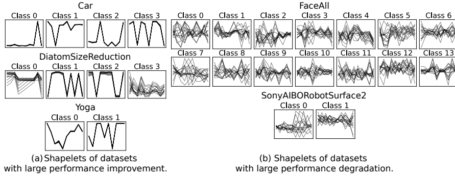
Figure 7: Illustrative examples of discriminative shapelets extracted from datasets with large improvement or degradation under the proposed method. Each small plot shows the discovered shapelets for one class of the corresponding UCR dataset. Panel (a) shows datasets where Shapelet Matching improved over no transfer learning, whereas panel (b) shows datasets where it degraded. These examples suggest that the proposed method is more effective when compact local class-discriminative subsequences are visible, and less effective when such local patterns are weak or ambiguous.
