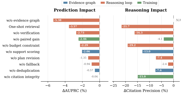
Figure 2: Ablation results from the full model, averaged across both datasets. Colors indicate framework stage.
