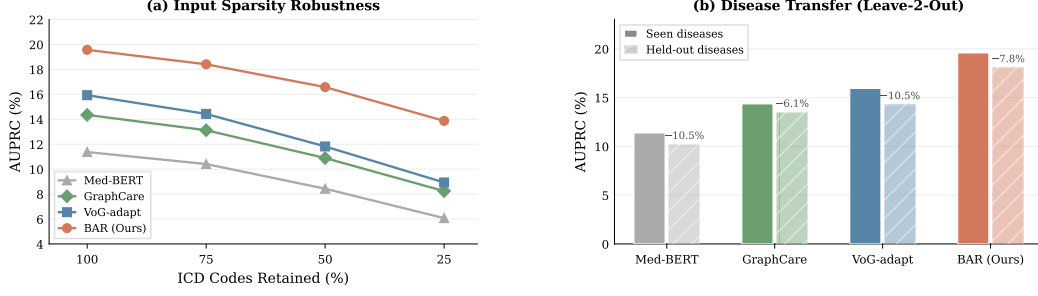
Figure 6: Robustness analysis on MIMIC-III. (a) AUPRC under random ICD code dropping at test time (no retraining). (b) Disease transfer via leave-2-out evaluation: train the full pipeline on 6 diseases, fine-tune only prediction heads on 2 held-out diseases (all other parameters frozen).
