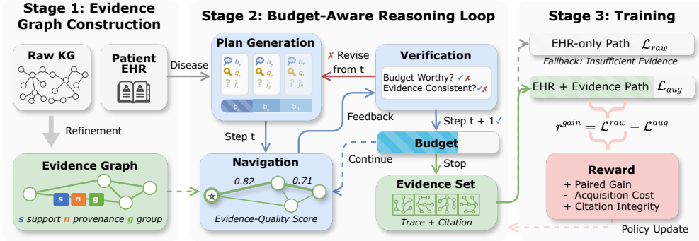
Figure 1: Overview of BAR. Stage 1: The raw KG is refined into a disease-specific evidence graph with per-edge support, provenance, and deduplication metadata. Stage 2: The LLM generates a budget-aware reasoning plan, navigates the evidence graph using a patient-conditioned quality score, and verifies each step for consistency and the cost-quality trade-off, revising as needed. Stage 3: The reasoning policy is trained via paired gain, acquisition cost, and citation-integrity reward.
