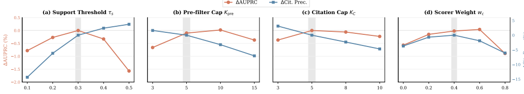
Figure 7: Sensitivity to key hyperparameters, averaged across 2 datasets. Gray bands mark defaults.
