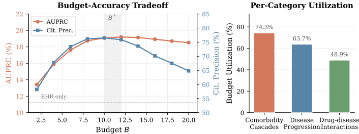
Figure 3: AUPRC and citation precision vs. budget B (left), and per-category budget utilization (right), averaged across both datasets.
