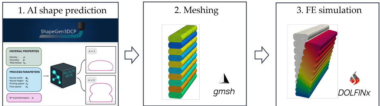
Figure 1: Automated workflow integrating machine-learning based filament shape prediction ( ShapeGen3DCP ) with robust layer-by-layer mesh generation ( gmsht ) and buildability finite element simulations (in DOLFINx ).
