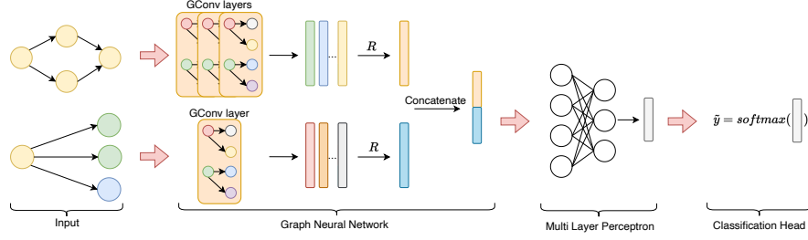
Fig. 4: The adopted network architecture for E3 and E4.
