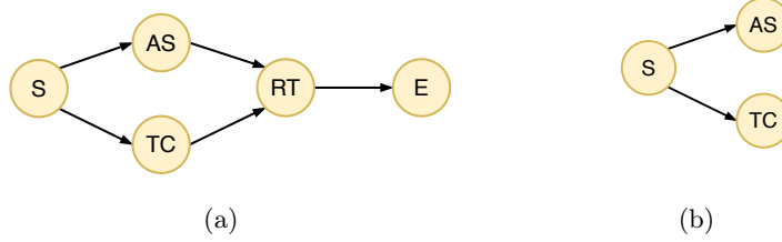
Fig. 1: The IG derived from Table 1 (a) and its prefix-IG of size 3 (b).
