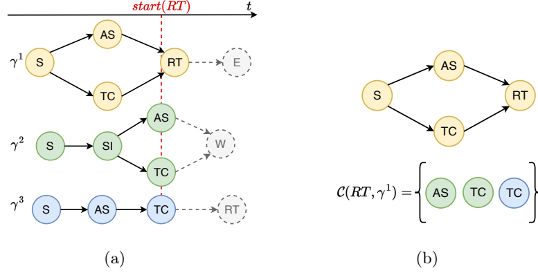
Fig. 2: An example of scenario in which \gamma^1 is the case under analysis (a), and RT the event for which the set of contextual events is identified (b).
