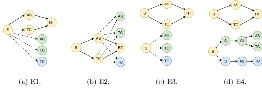
Fig. 3: The proposed encoding strategies.
