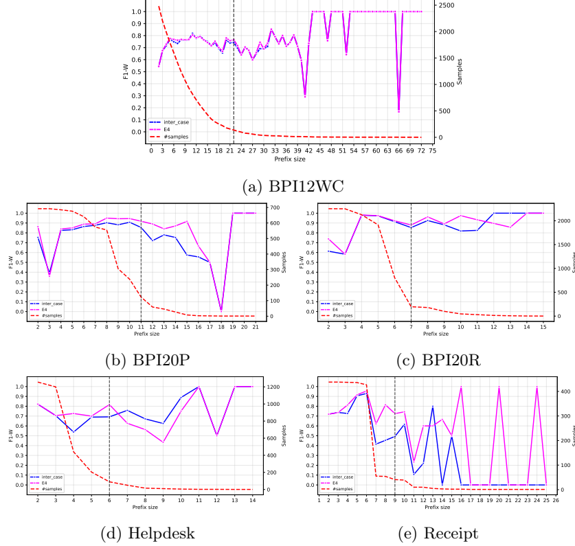
Fig. 5: F1-W on test set varying the prefix-IG size.
