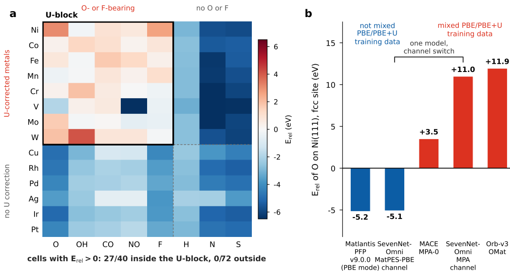
Figure 2: MACE-MPA-0 predicts anomalous energies only in the U -block. a , Relative energy E_{\text{rel}} of MACE-MPA-0 across 14 metal surfaces and 8 adsorbates, referenced to the clean slab and isolated adsorbate. E_{\text{rel}} > 0 indicates that the relaxed adsorbate–surface system lies above its separated-fragment reference; MLIP Detective used E_{\text{rel}} > 0 as a diagnostic flag for candidate failures. All 27 anomalous cases lie within the outlined U -block (27 of 40 cells). b , E_{\text{rel}} for O on Ni(111) at identical geometry across five model/channel configurations. The prediction varies substantially across model channels, supporting an association between the anomaly in the U -block and mixed PBE/PBE+ U training data.
