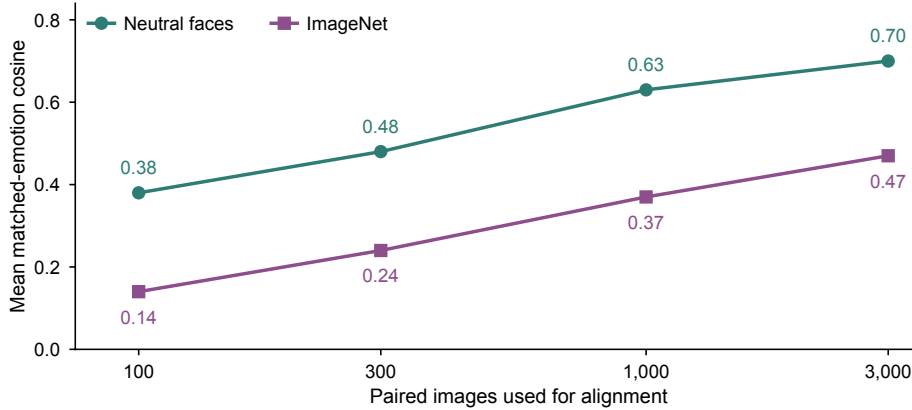
Figure 17: Alignment sample size and Ministral-3→Qwen3-VL correspondence. Maps use paired neutral-face or ImageNet activations without emotion-vector fitting. Points show mean cosine across six AffectNet emotion pairs. Sample size is on a logarithmic axis. Reference cosine similarities are 0.00 before alignment, 0.30 with LOEO, and 0.99 with a full fit.
